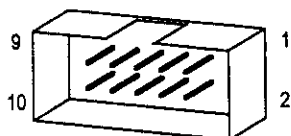
Figure C-1: Pin Locations for J2 (CQD-420) and J3
