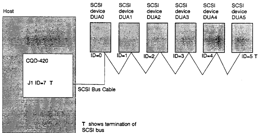
Figure 3-8: SCSI ID and Cabling
