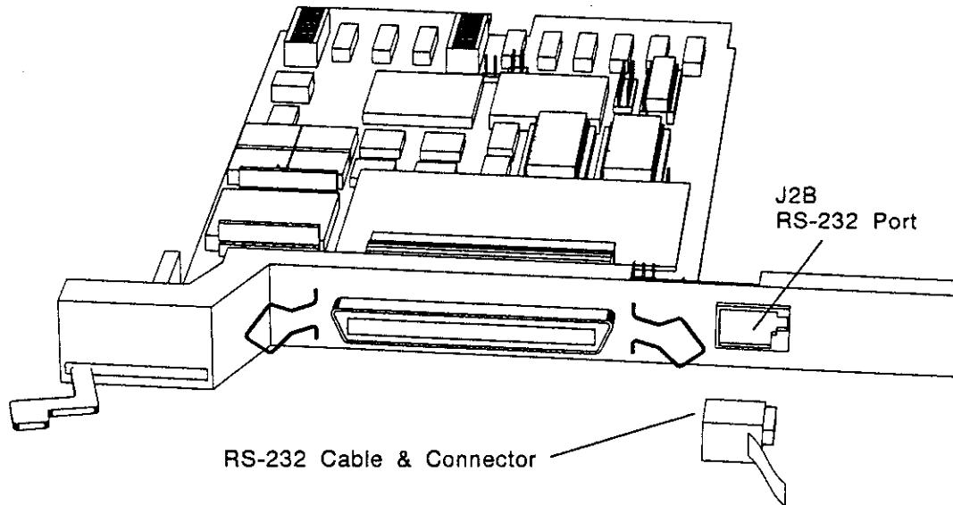
Figure 4-2: CQD-423 RS-232 Port
