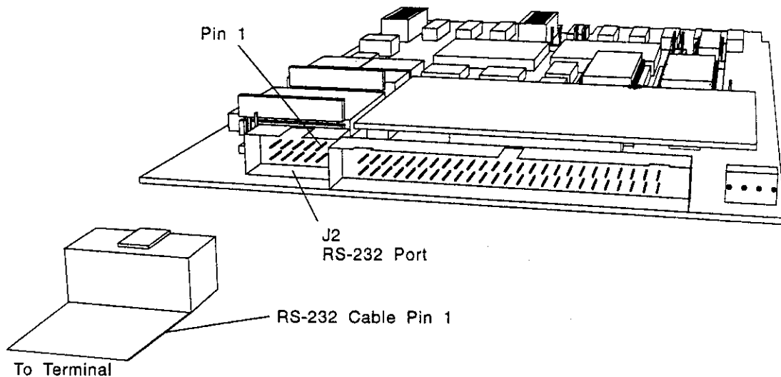
Figure 4-1: CQD-420 RS-232 Port
