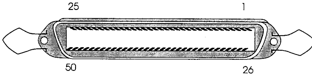
Figure 5-2: SCSI device shielded connector
