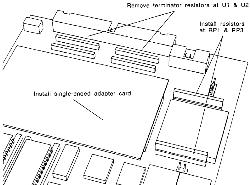
Figure 3-3: Single-ended Mode Selection
