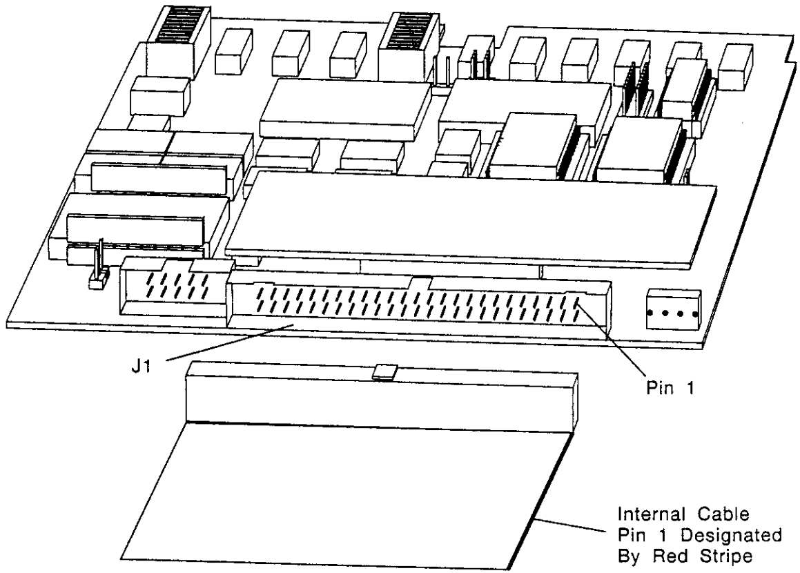
Figure 3-6: CQD-420 non-shielded cable connection
