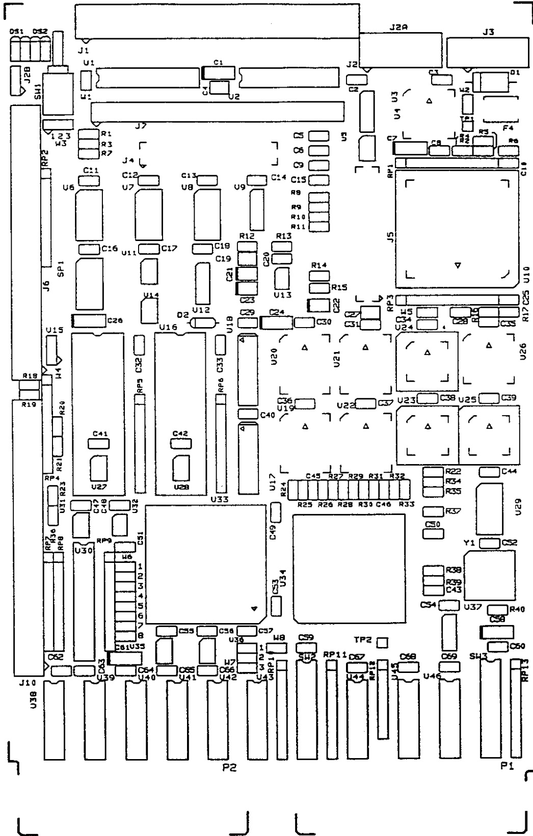
Figure 3-2: Jumper block locations
