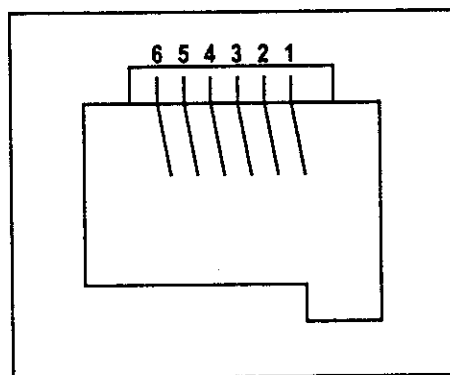
Figure C-2: Pin Locations for J2B (CQD-423)
