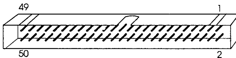
Figure 5-1: SCSI device non-shielded connector
