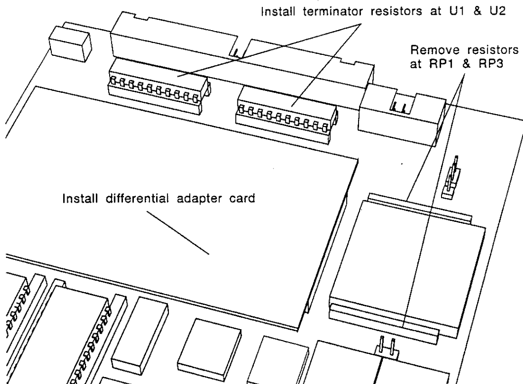
Figure 3-4: Differential Mode Selection
