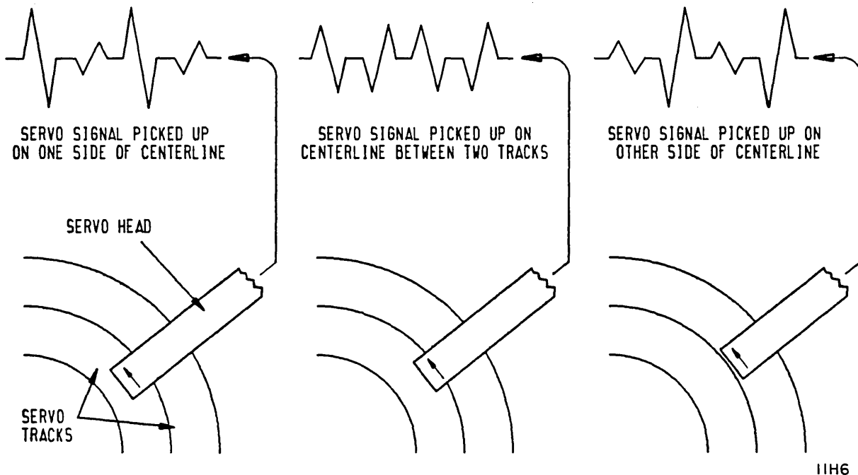
Figure 4-2. Dibit Signal Variations
