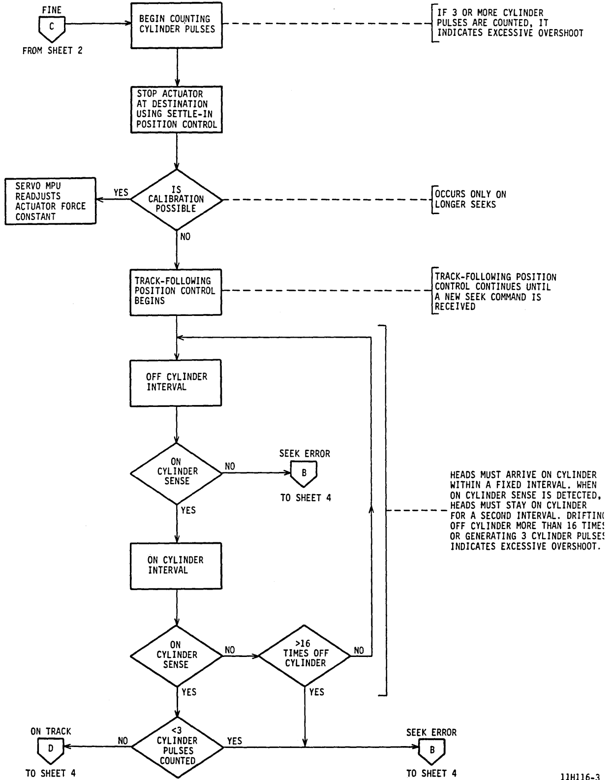
Figure 5-15. Normal Seek Flowchart (Sheet 3)
