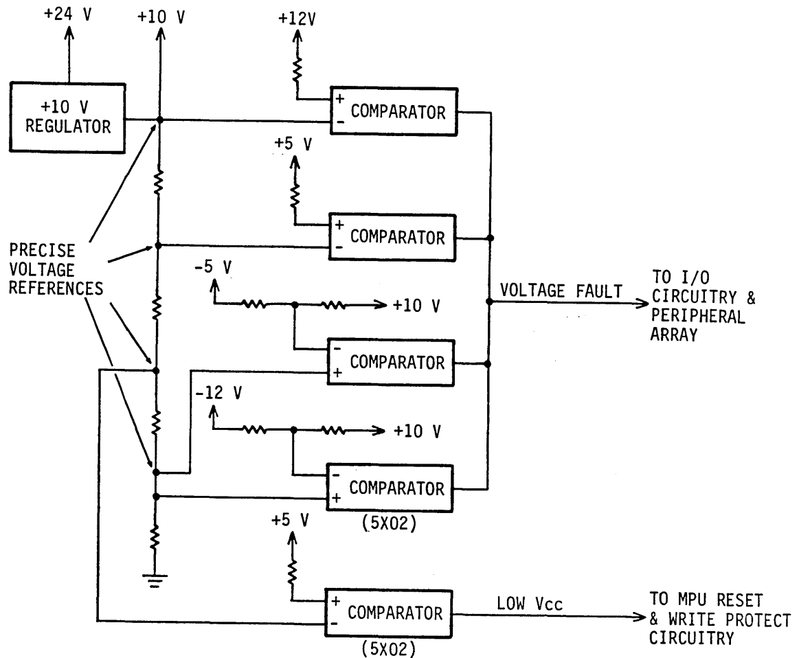
Figure 7-3. Detecting Voltage Faults
