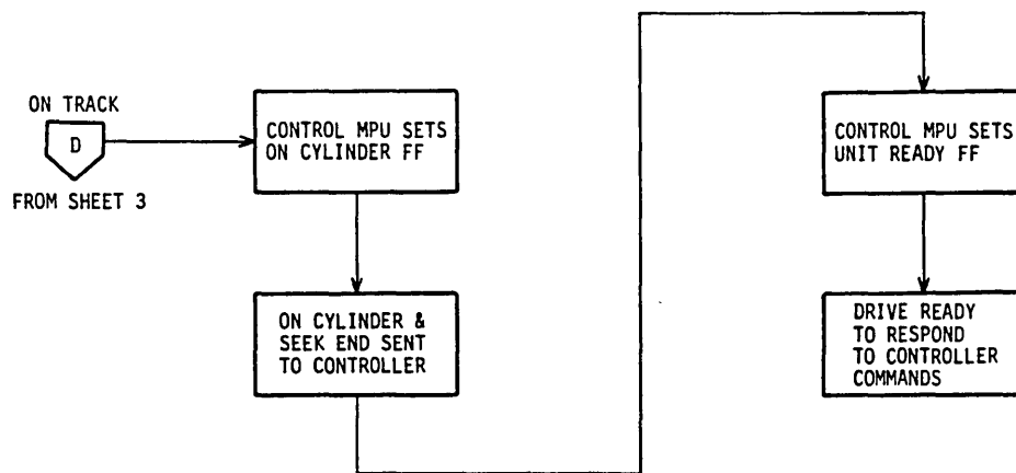
Figure 5-13. Load Operation Flowchart (Sheet 4)
