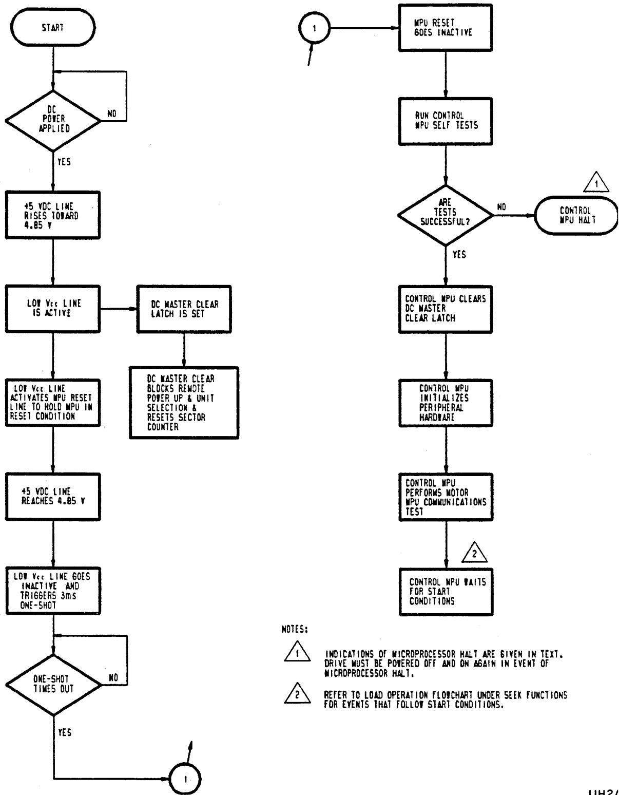
Figure 2-5. Power On Sequence Flowchart
