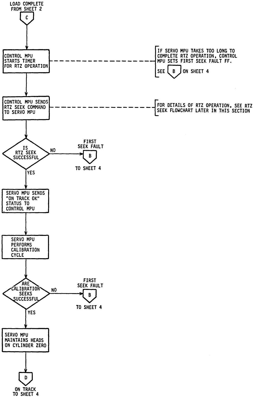
Figure 5-13. Load Operation Flowchart (Sheet 3)
