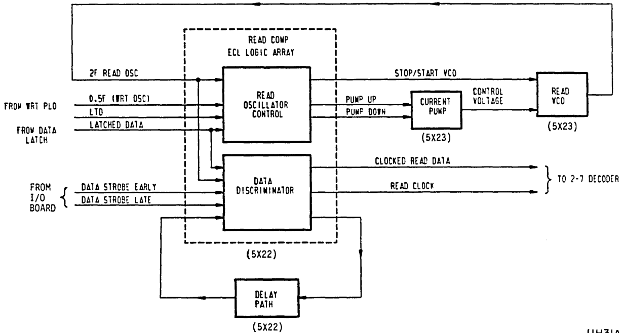
Figure 6A-12. Read Comparator and PLO Block Diagram
