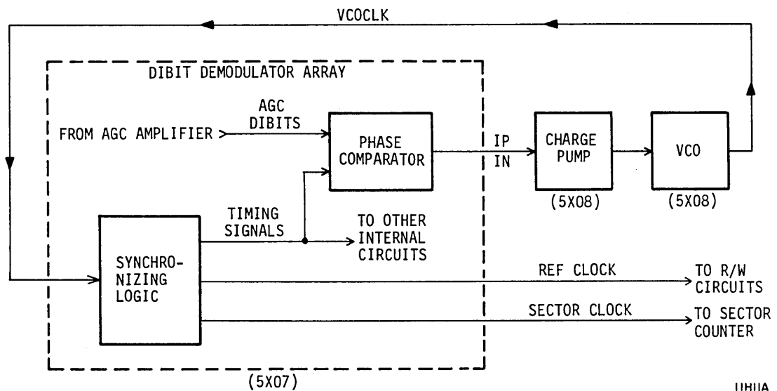
Figure 4-7. Servo PLO and Timing Circuitry
