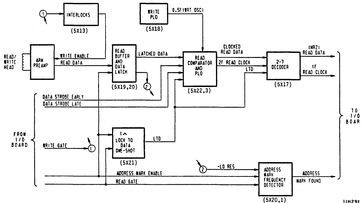
Figure 6A-9. Read Circuits Block Diagram
