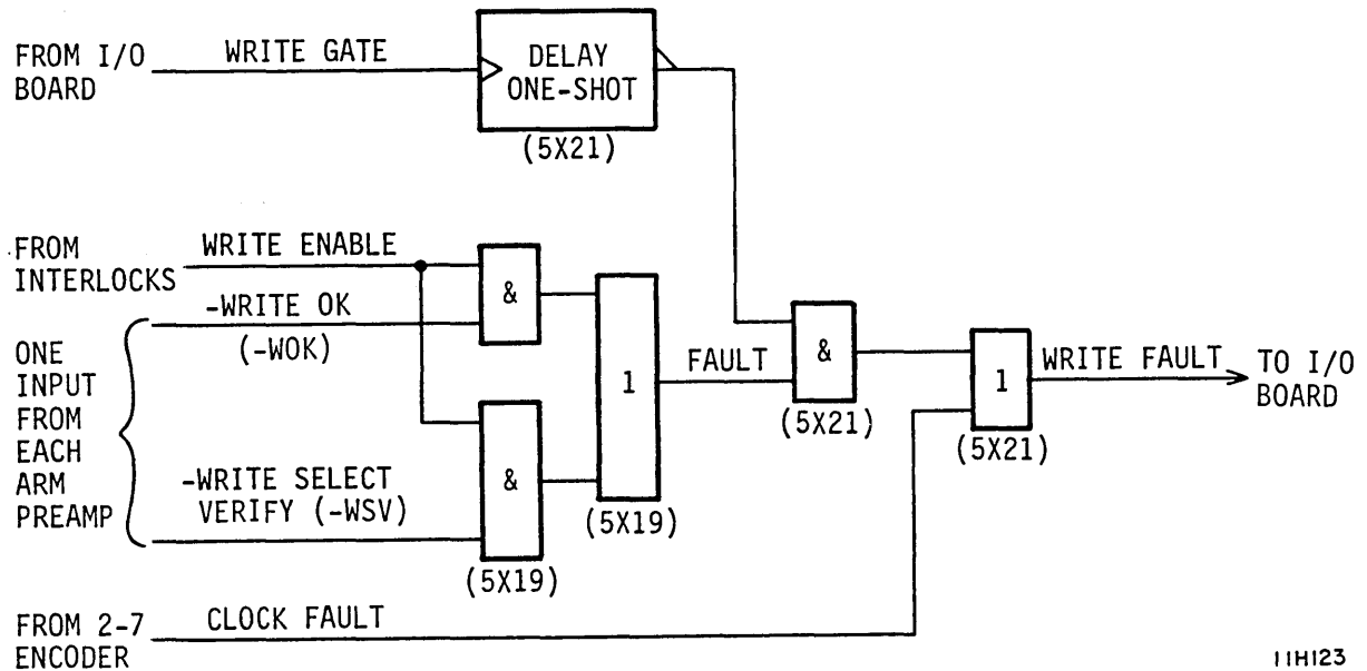
Figure 7-4. Detecting Write Faults
