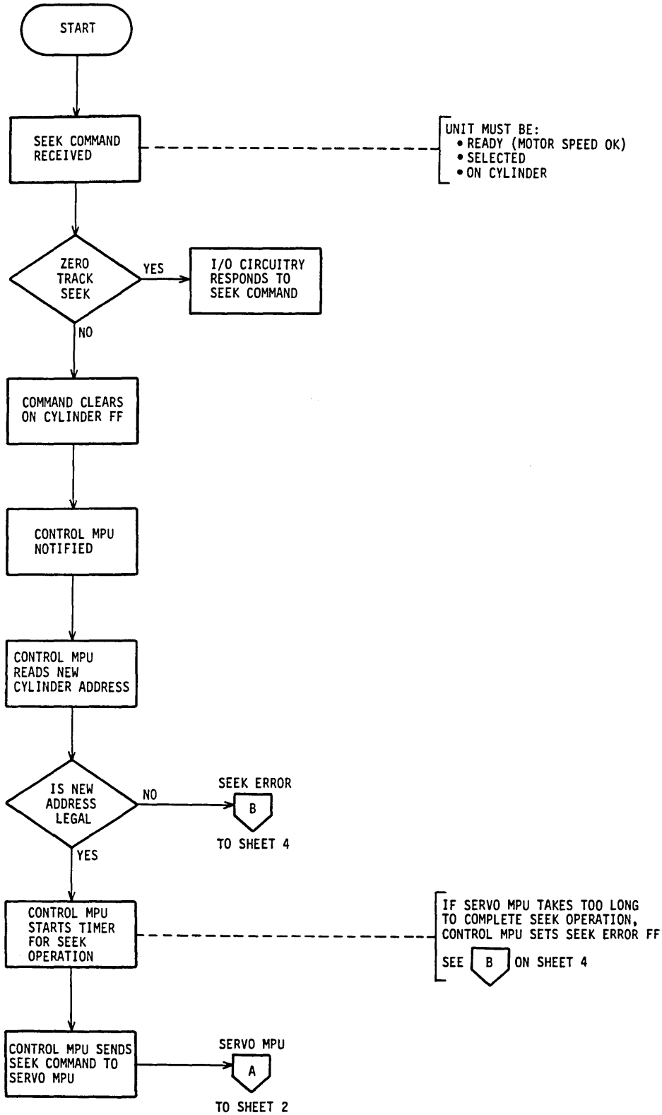
Figure 5-15. Normal Seek Flowchart (Sheet 1 of 4)
