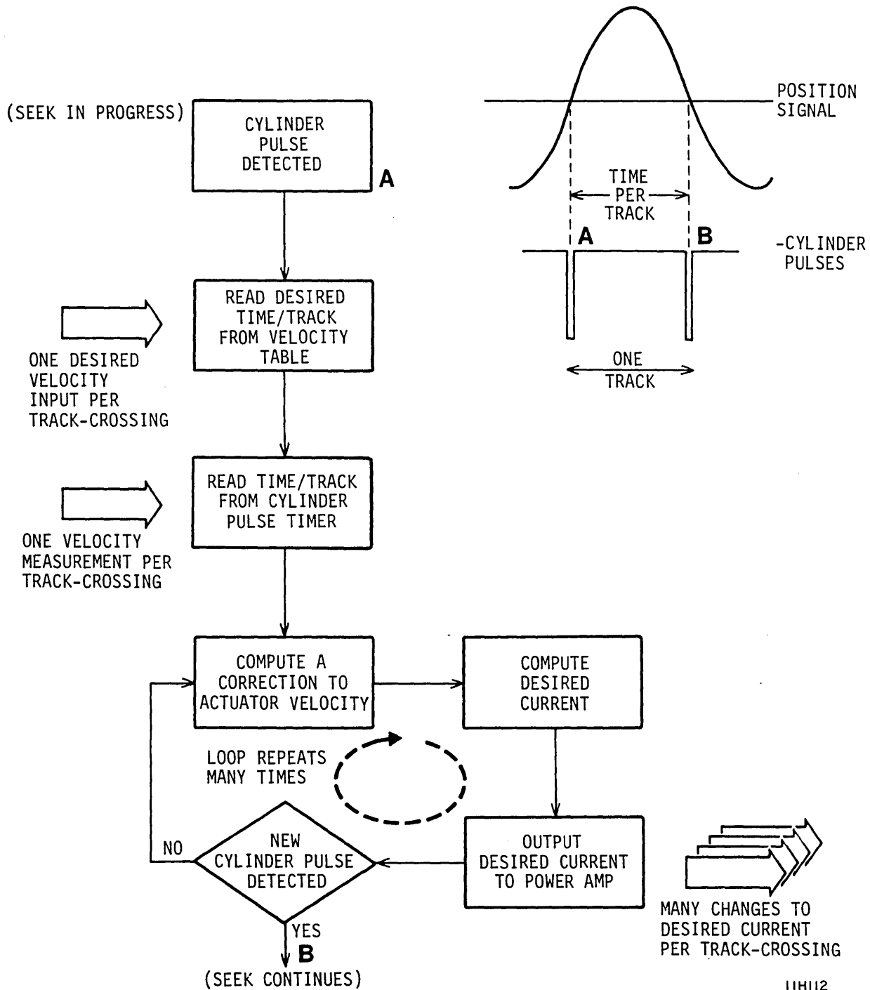
Figure 5-6. One Track of a High-Speed Seek
