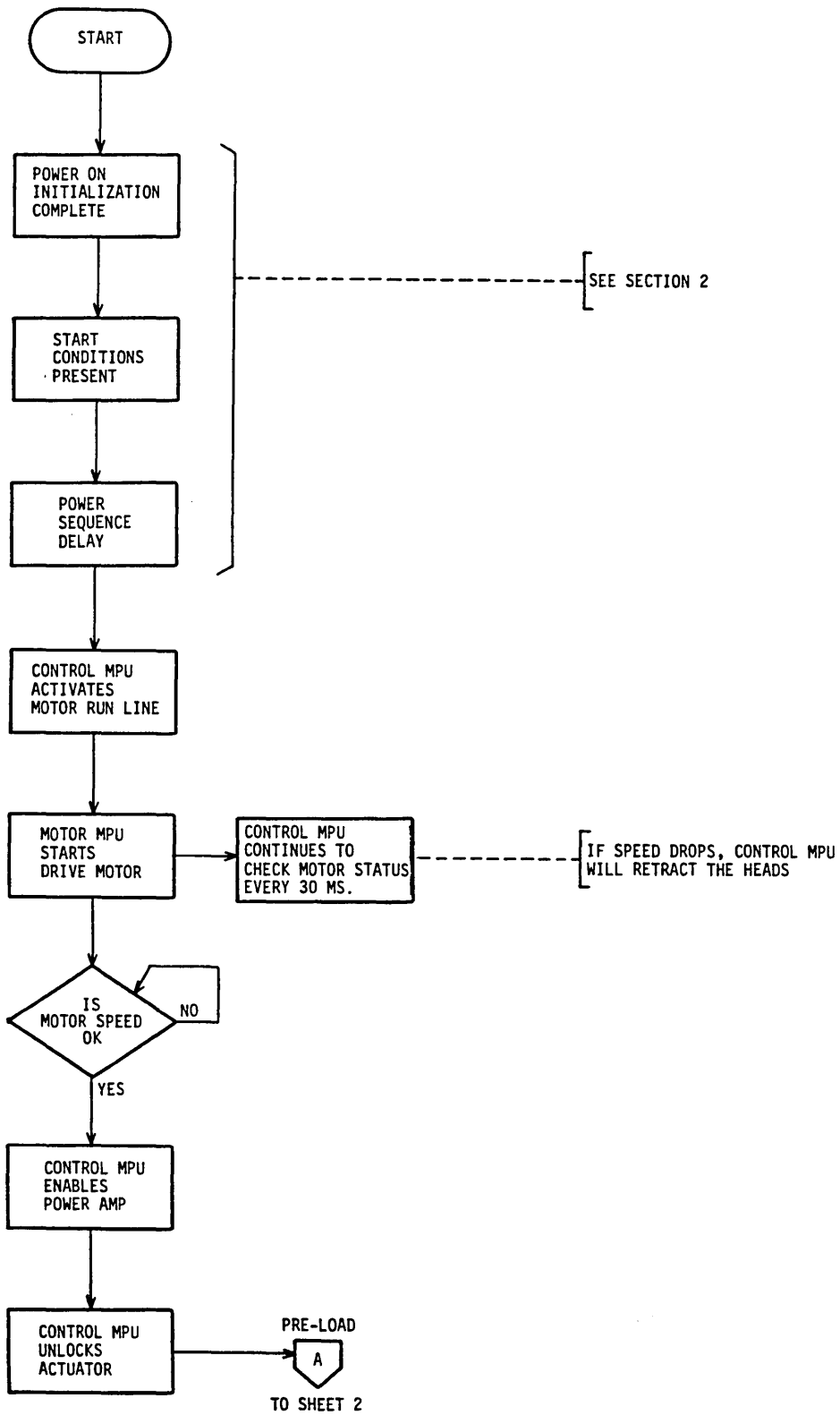
Figure 5-13. Load Operation Flowchart (Sheet 1 of 4)
