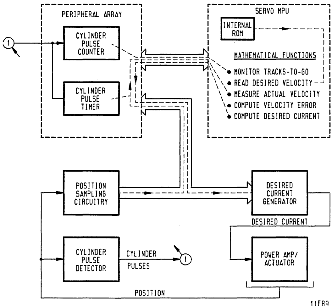
Figure 5-5. Simplified Coarse Servo Loop
