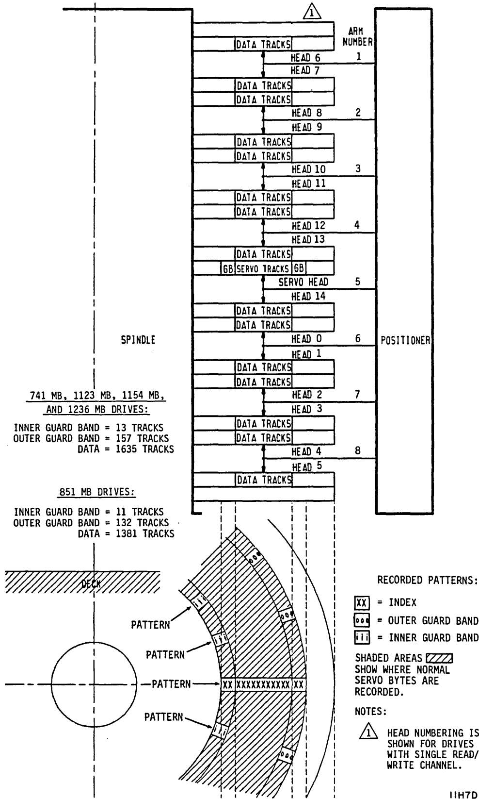
Figure 4-3. Servo Disc Format
