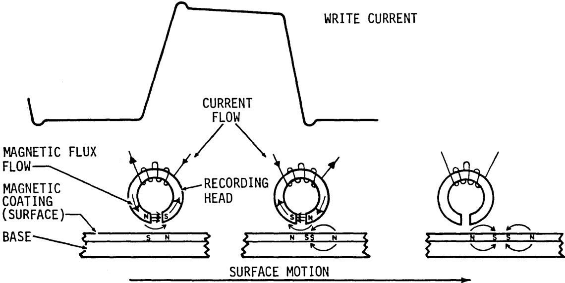
NOTE: RELATIVE HEAD TO SURFACE MOTION, RECORDING (WRITE OPERATION) 11D189
