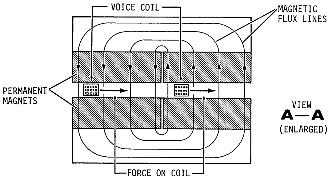
CROSS-SECTIONAL VIEW OF MAGNET AND COIL
