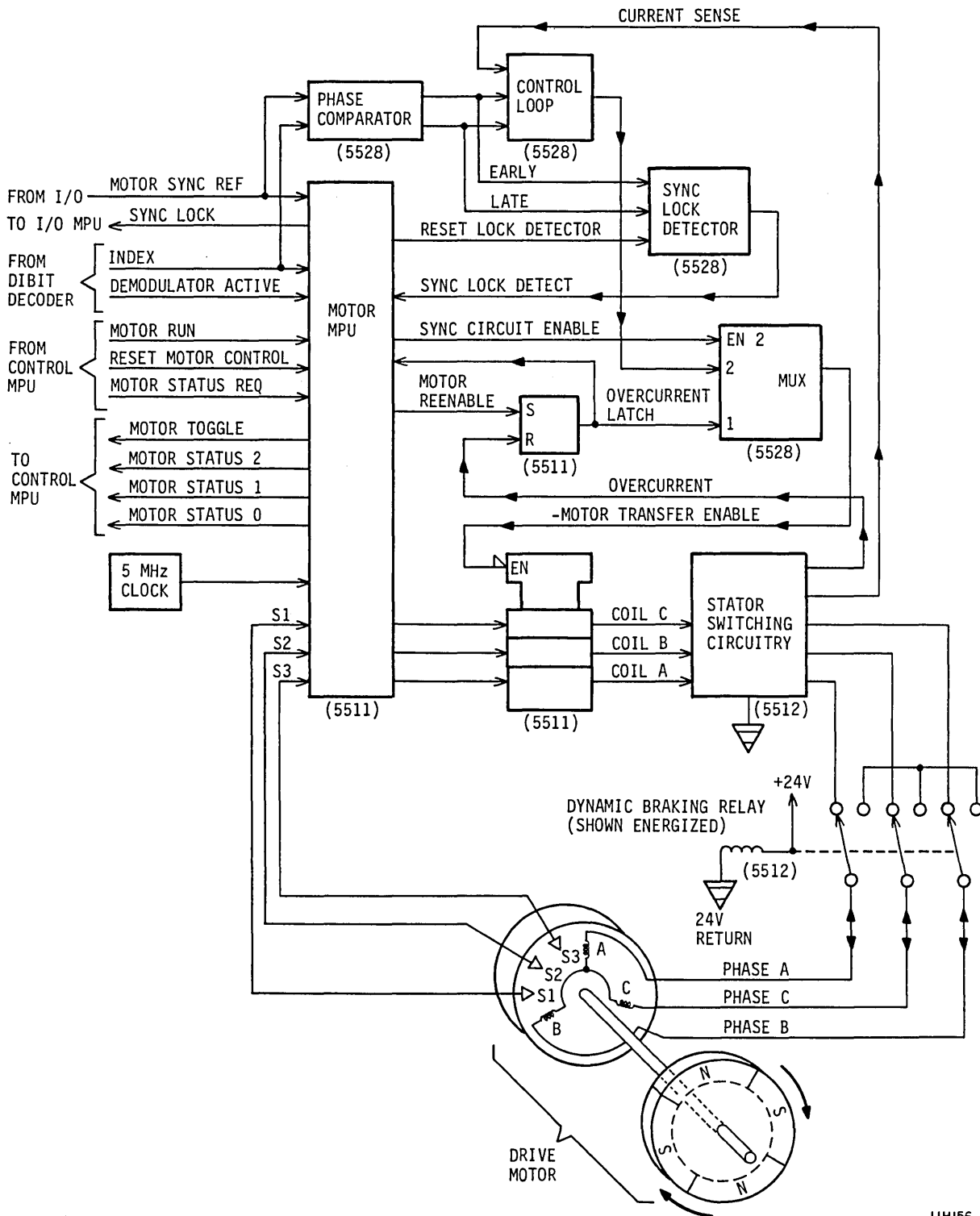
Figure 2-11. Synchronized Motor Speed Control Logic
