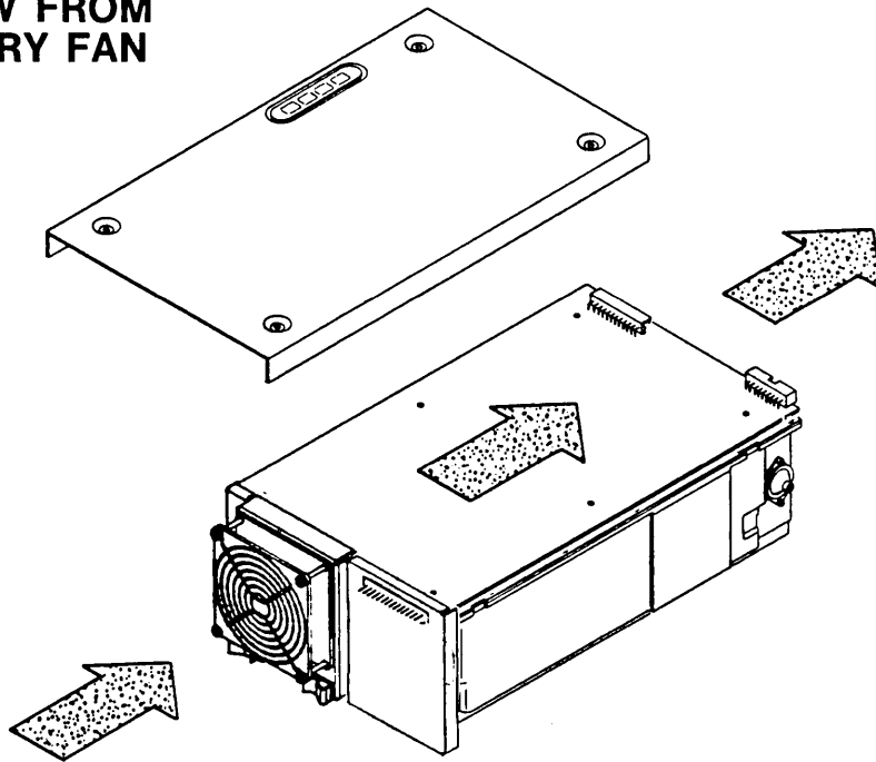
Figure 2-13. Drive Ventilation
