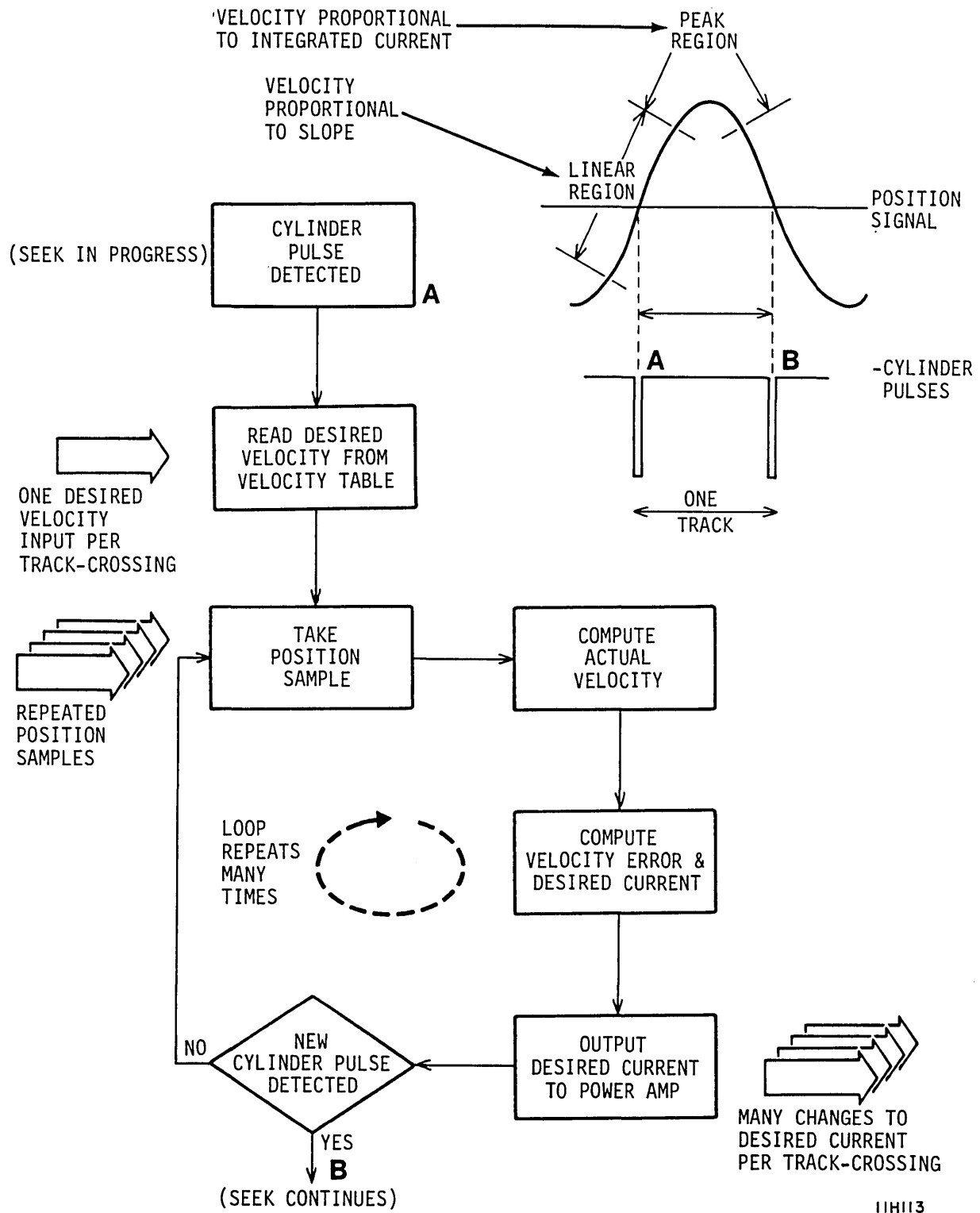
Figure 5-7. One Track of a Low-Speed Seek
