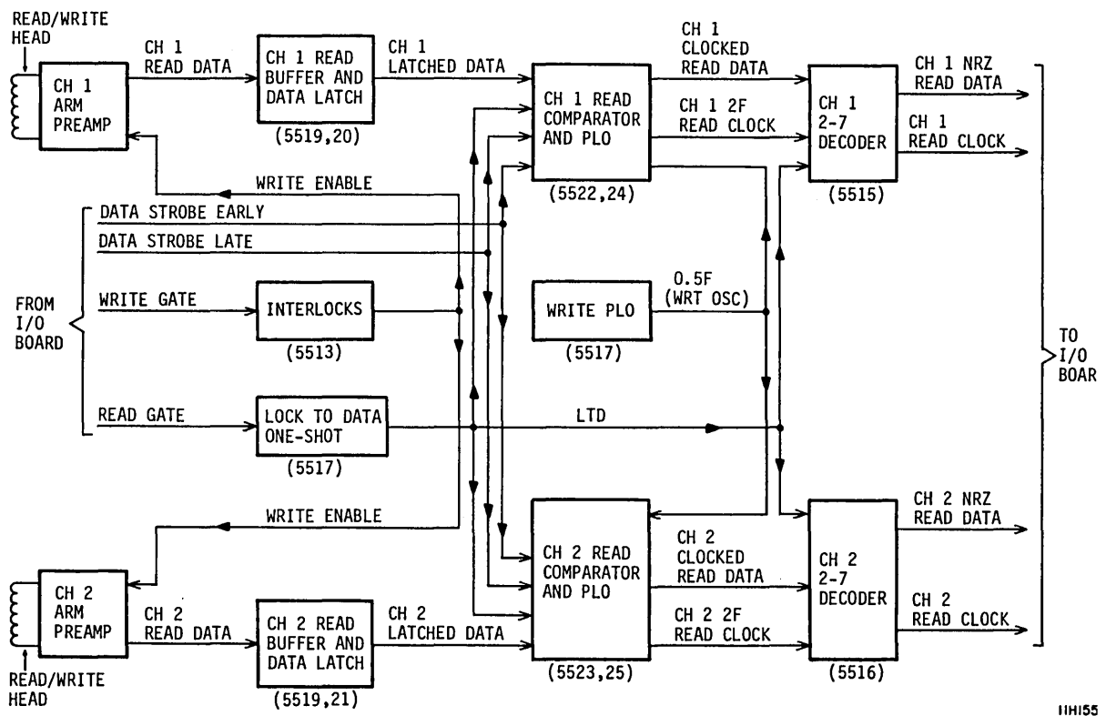
Figure 6B-4. Read Circuits Block Diagram (Parallel)
