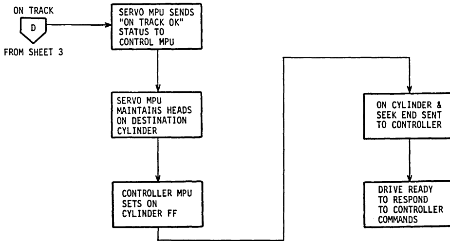
Figure 5-15. Normal Seek Flowchart (Sheet 4)
