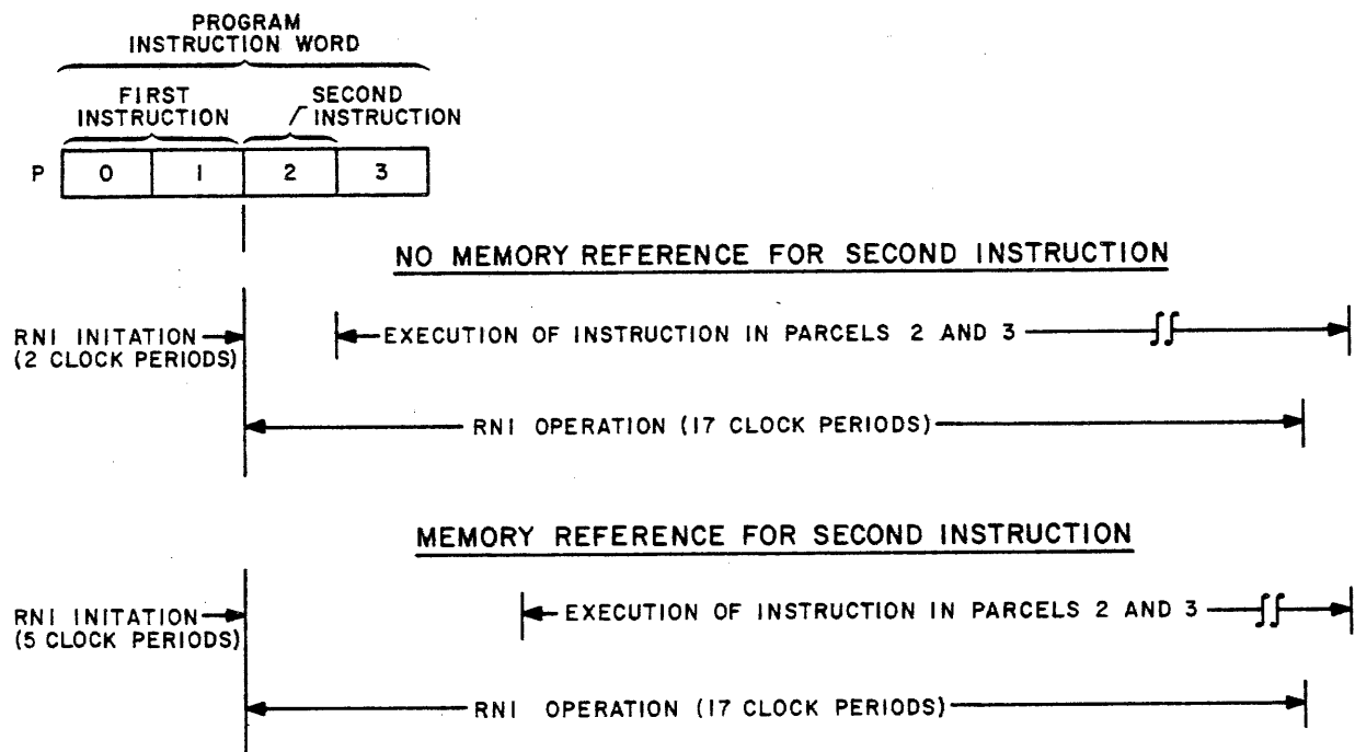
Figure 5-3. Instruction Execution - Models 720 and 730
