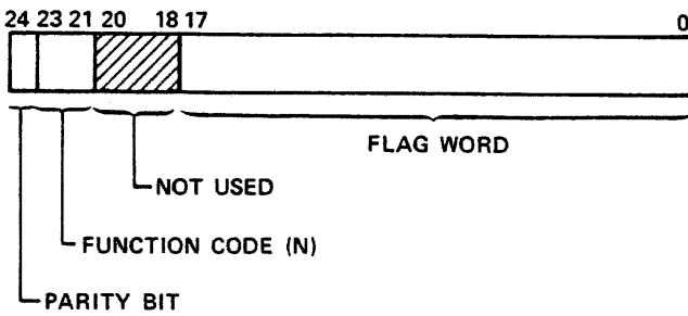
Figure 5-9. ECS Address Format for Flag Register Operation
