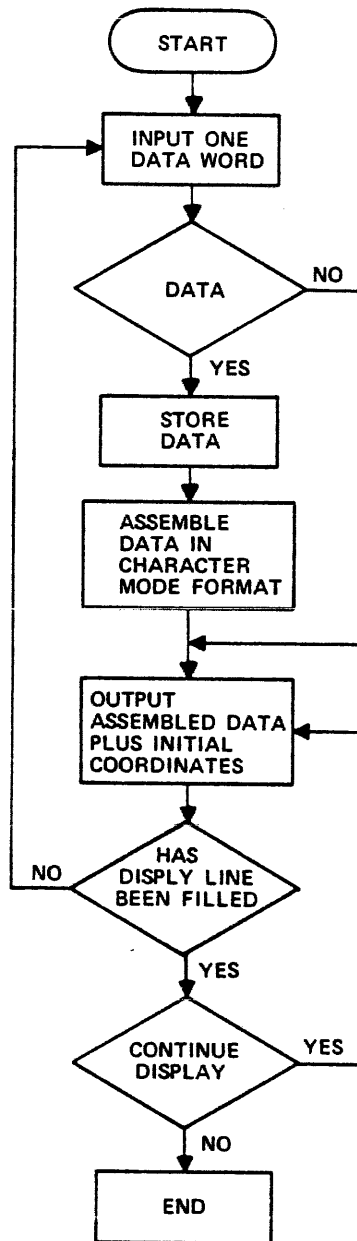
Figure 5-16. Receive and Display Program Flowchart
