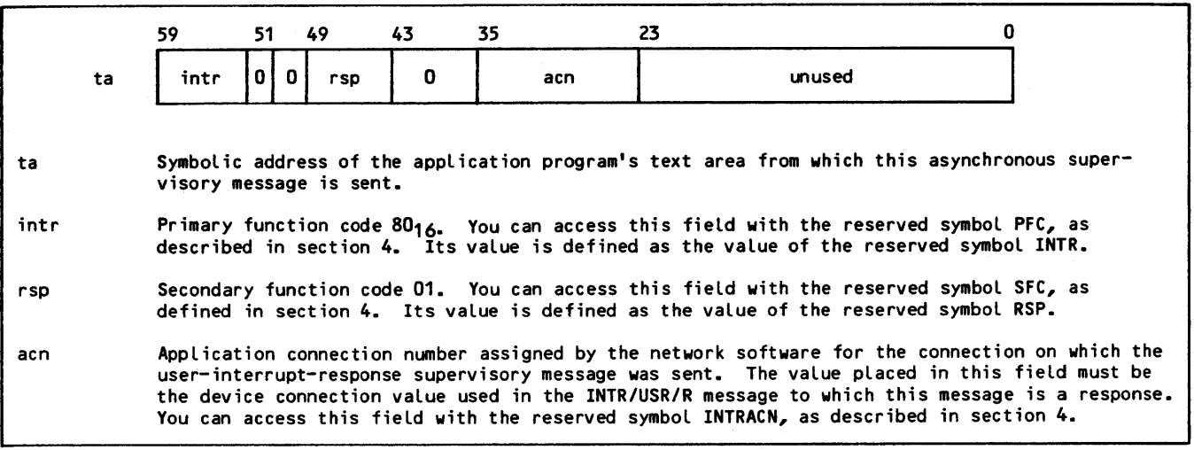
Figure 3-33. Application-Interrupt-Response (INTR/RSP/R) Supervisory Message Format
