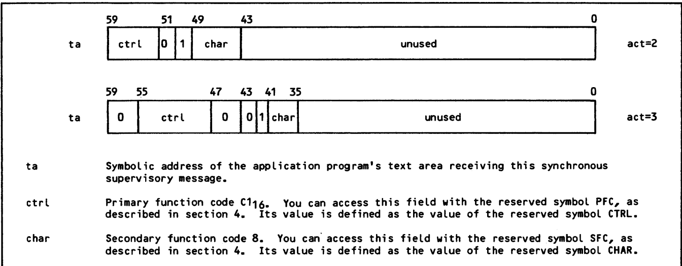
Figure 3-50. Multiple-Terminal-Characteristics-Defined (CTRL/CHAR/N) Supervisory Message Format
