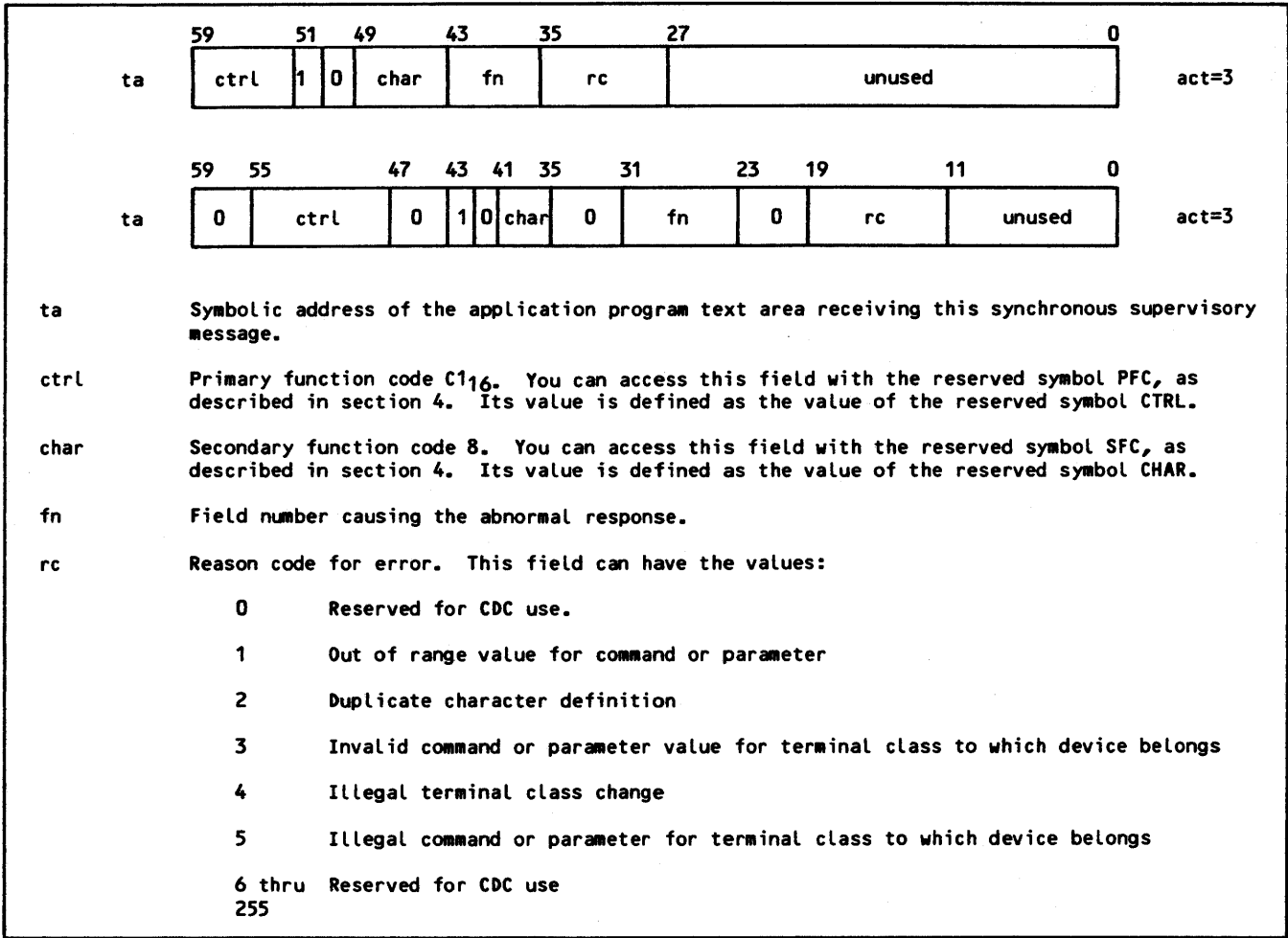
Figure 3-49. Define-Multiple-Terminal-Characteristics Abnormal Response (CTRL/CHAR/A) Supervisory Message Format
