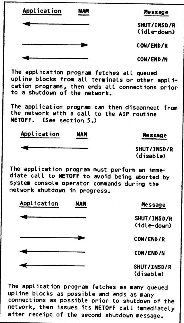
Figure 3-62. Host Shutdown Supervisory Message Sequences
