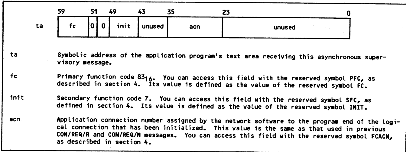
Figure 3-6. Initialized-Connection (FC/INIT/R) Supervisory Message Format
