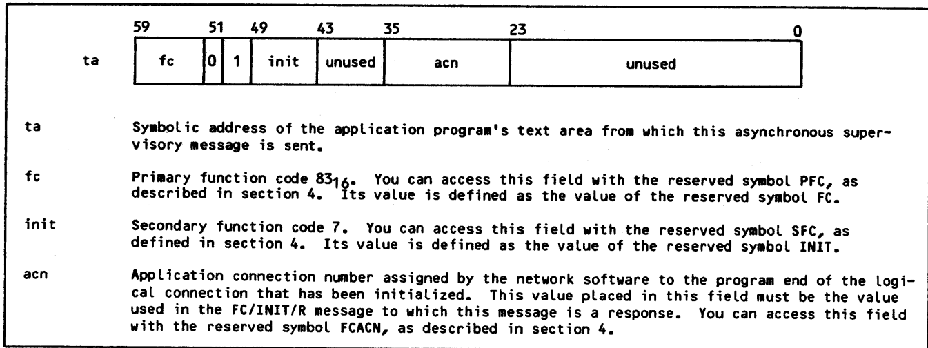
Figure 3-7. Connection-Initialized (FC/INIT/N) Supervisory Message Format
