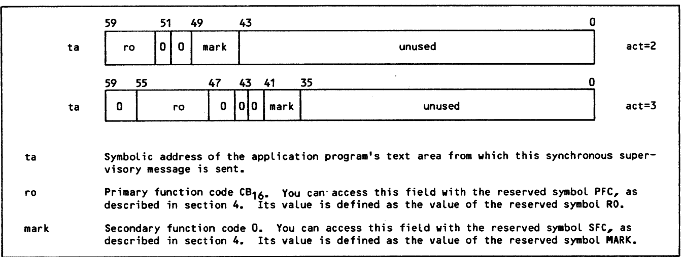
Figure 3-34. Resume-Output-Marker (R0/MARK/R) Supervisory Message Format
