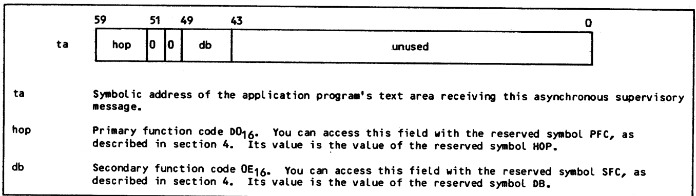
Figure 3-55. Host Operator Request-to-Activate-Debug-Code (HOP/DB/R) Supervisory Message Format
