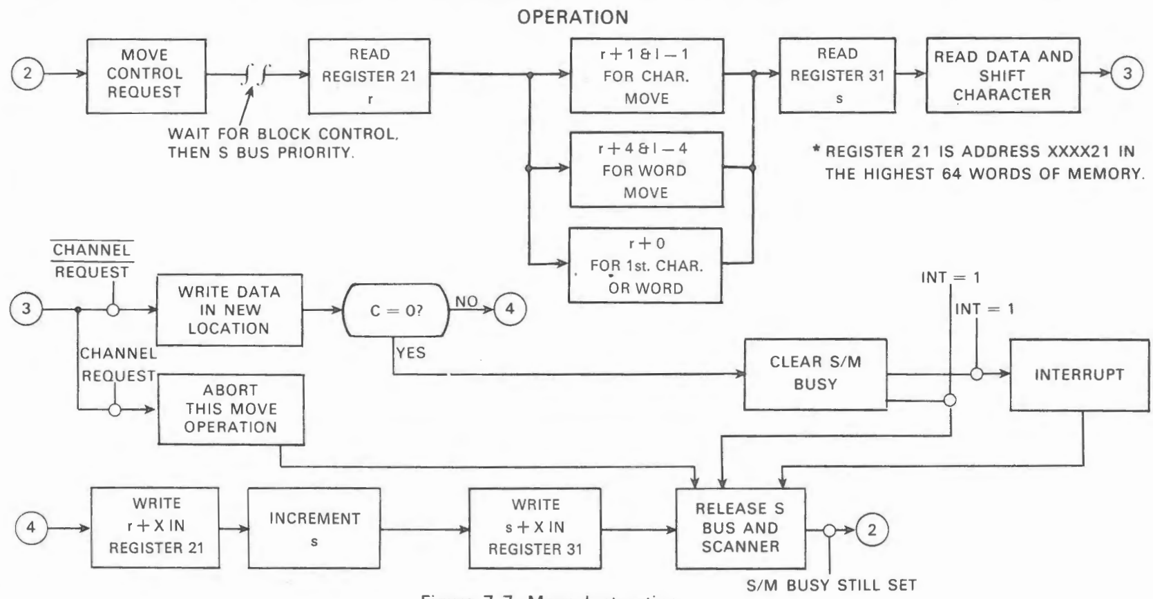
Figure 7-7. Move Instruction
