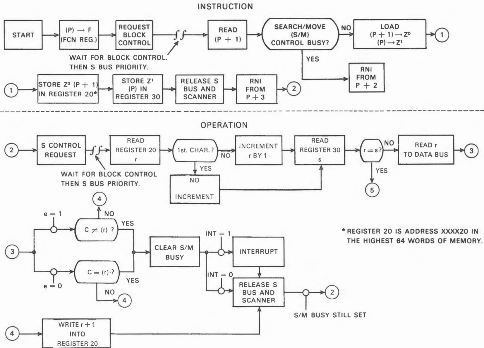
Figure 7-6. Search Operation
