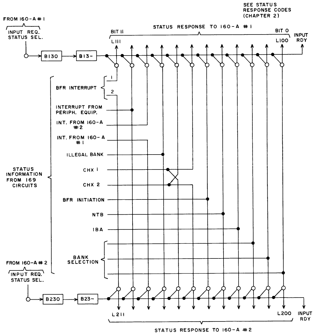
Figure 3-15. Status Response Gating
