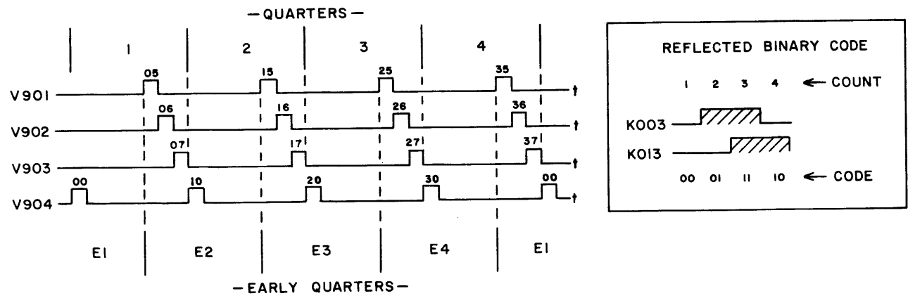
Figure 3-13. External Buffer Timing Controls
