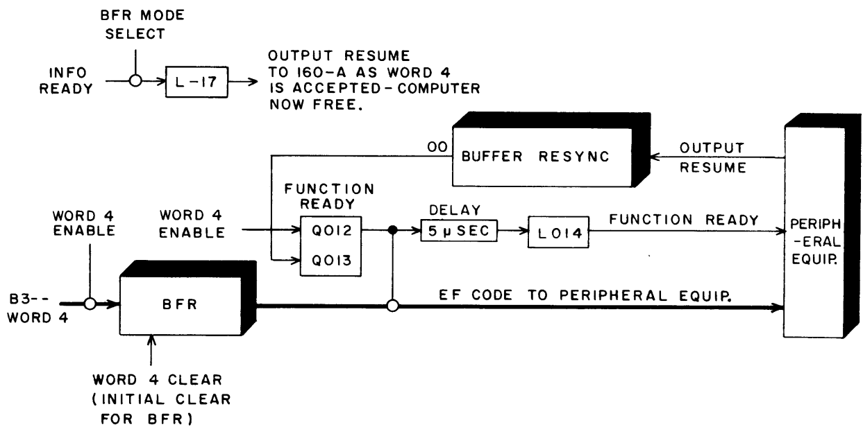
Figure 3-23. Word 4 Circuit
