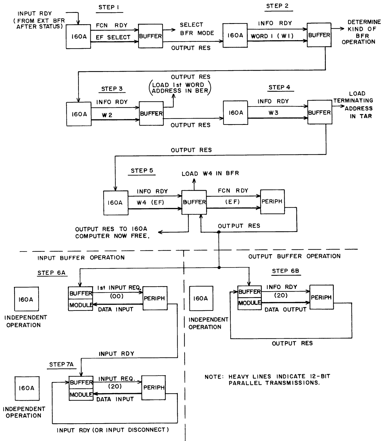
Figure 3-17. Control Signal Sequence for Buffer Mode Operation
