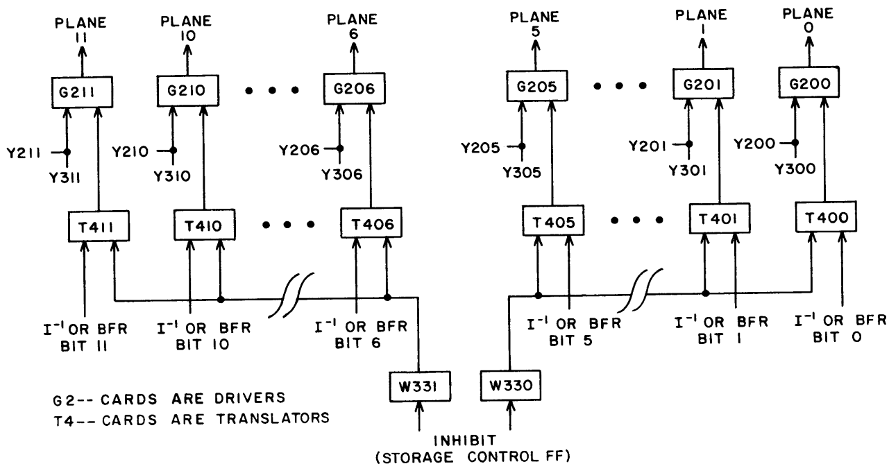
Figure 3-7. Inhibit Driver Selection
