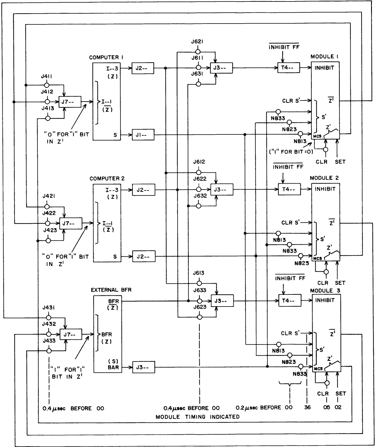
Figure 3-10. Module Gating Control (for 1 bit of 12-bit word)
