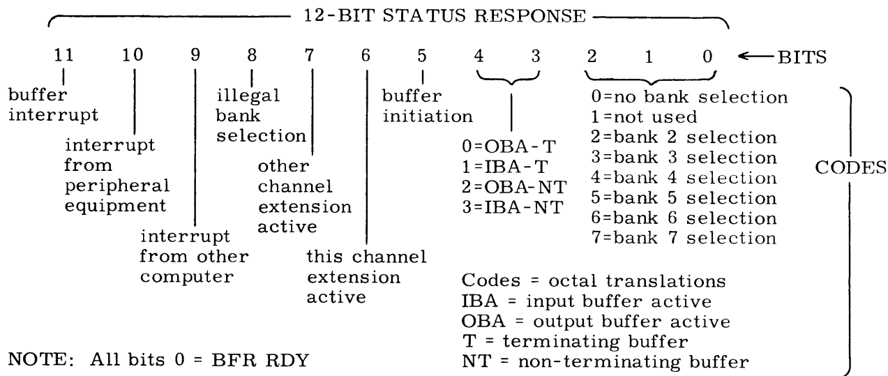
Figure 2-2. Status Response
