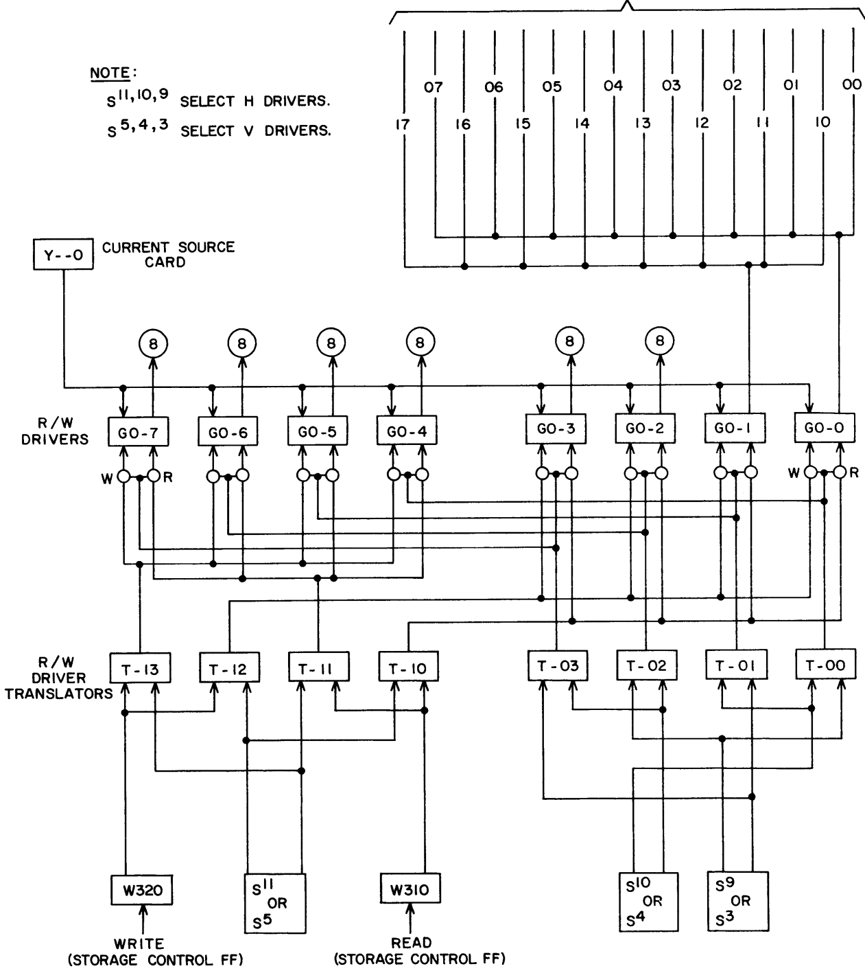
Figure 3-5. R/W Driver Selection
