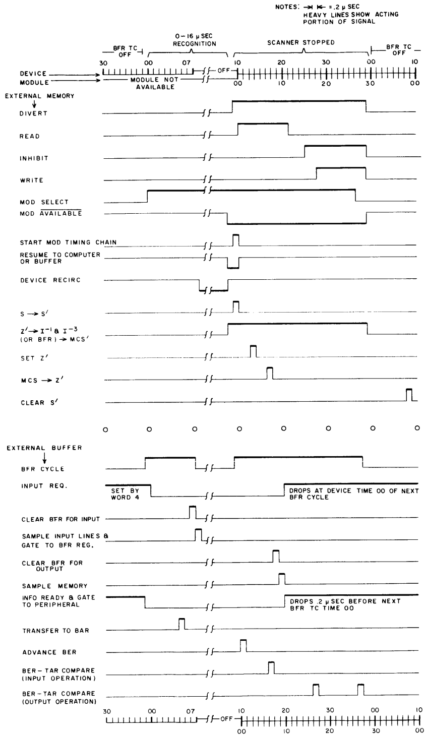
Figure 3-26. 169 Timing Chart
