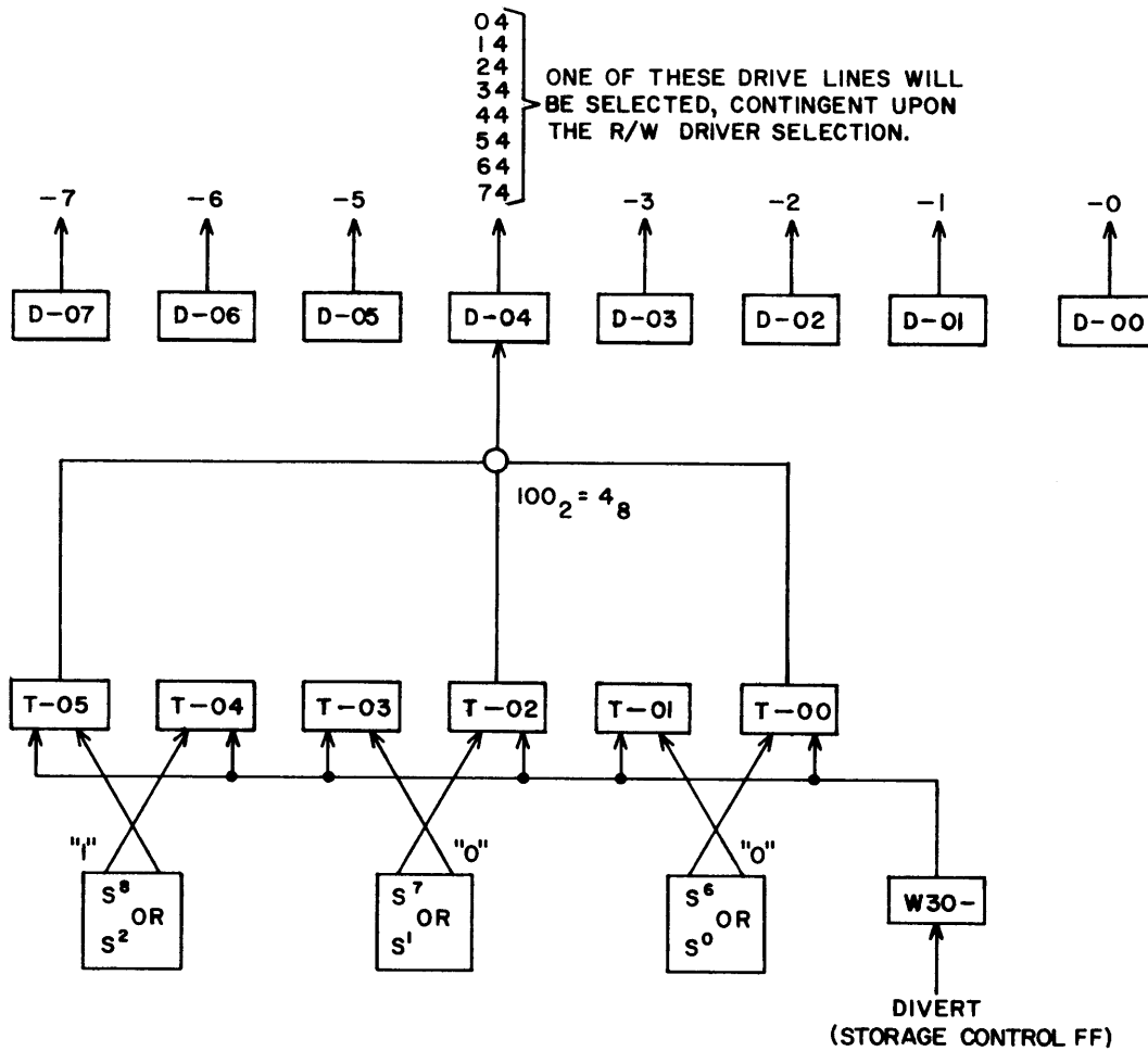
Figure 3-6. Diverter Selection
