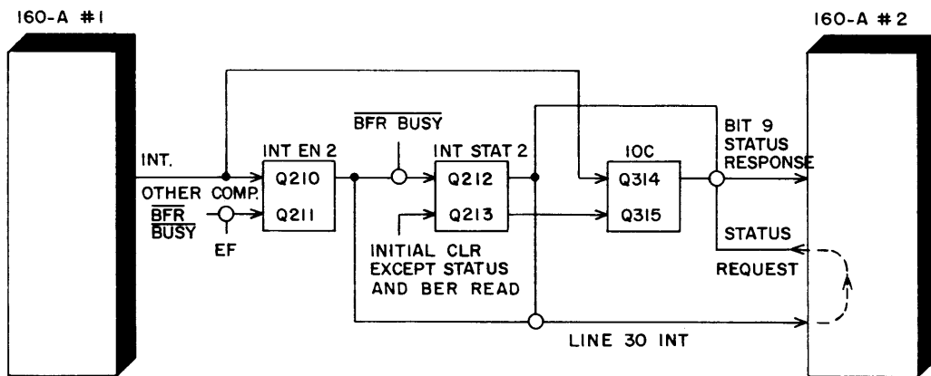
CASE 3: INTERRUPT OTHER COMPUTER
