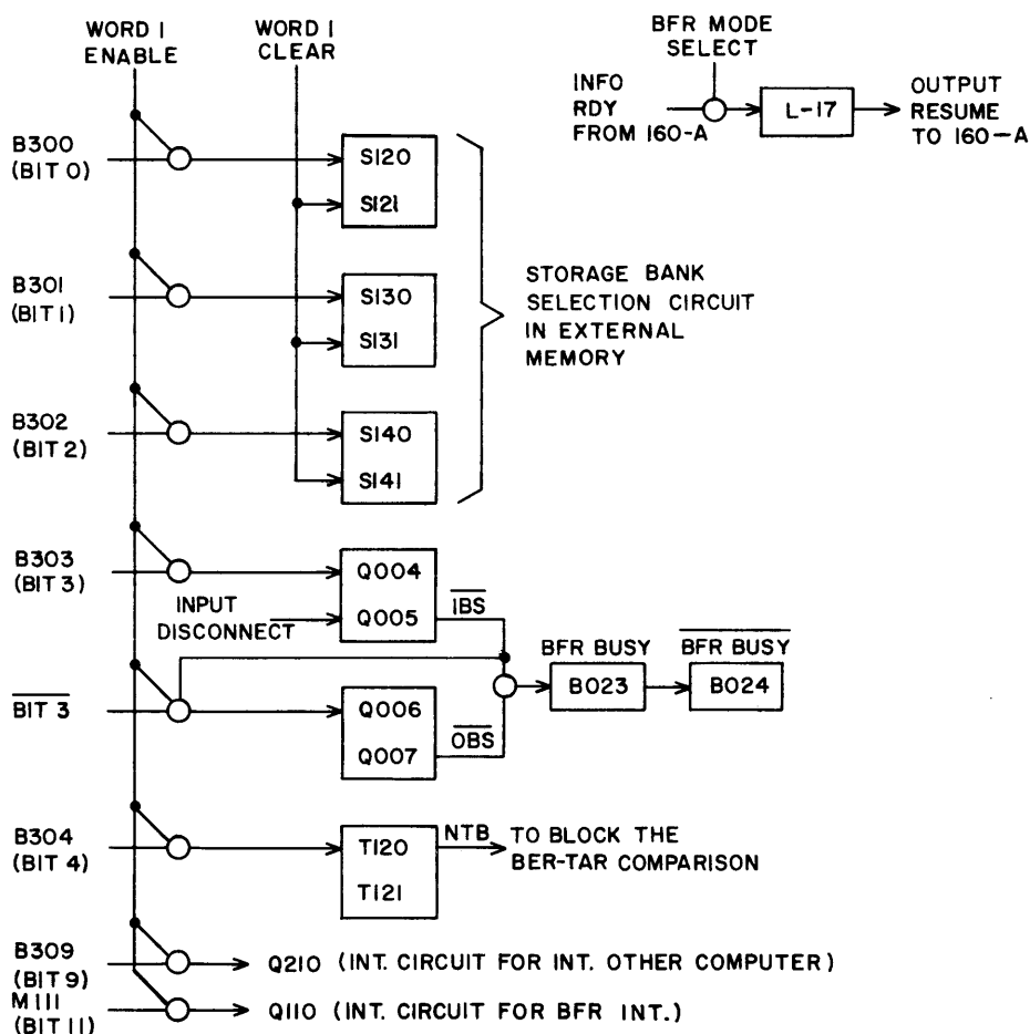
Figure 3-19. Word 1 Circuit
