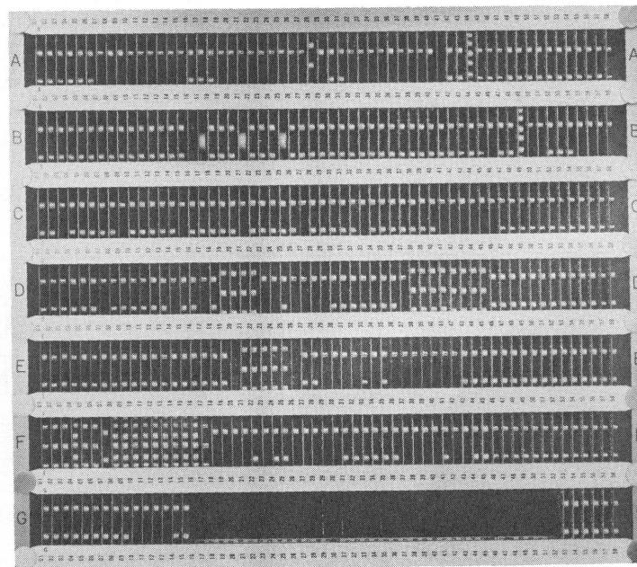
Figure 4-2. Control Chassis
