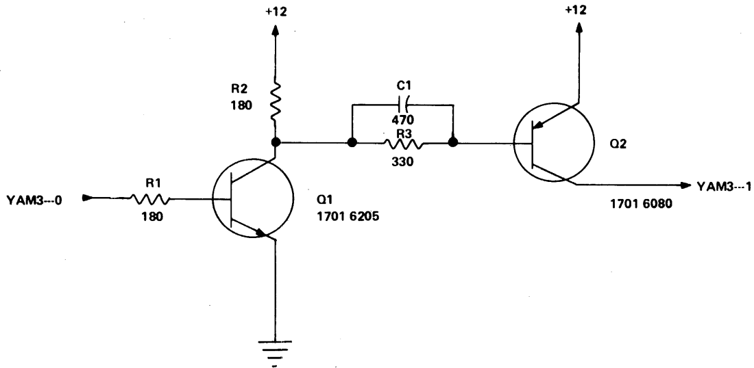
Fig. III-14 SELECTION SWITCH
