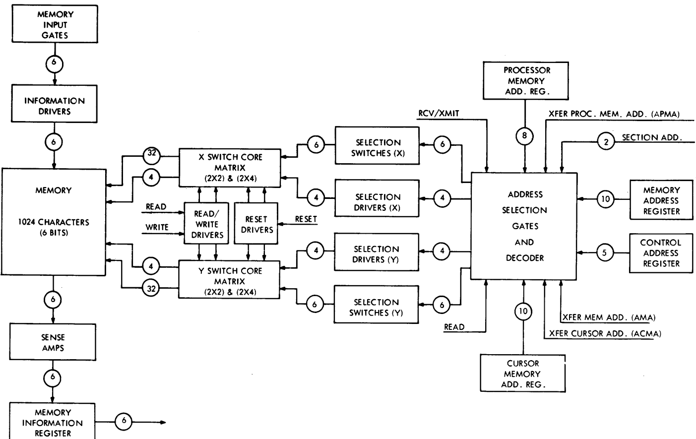
Fig. III-11 BLOCK DIAGRAM - MEMORY SECTION
