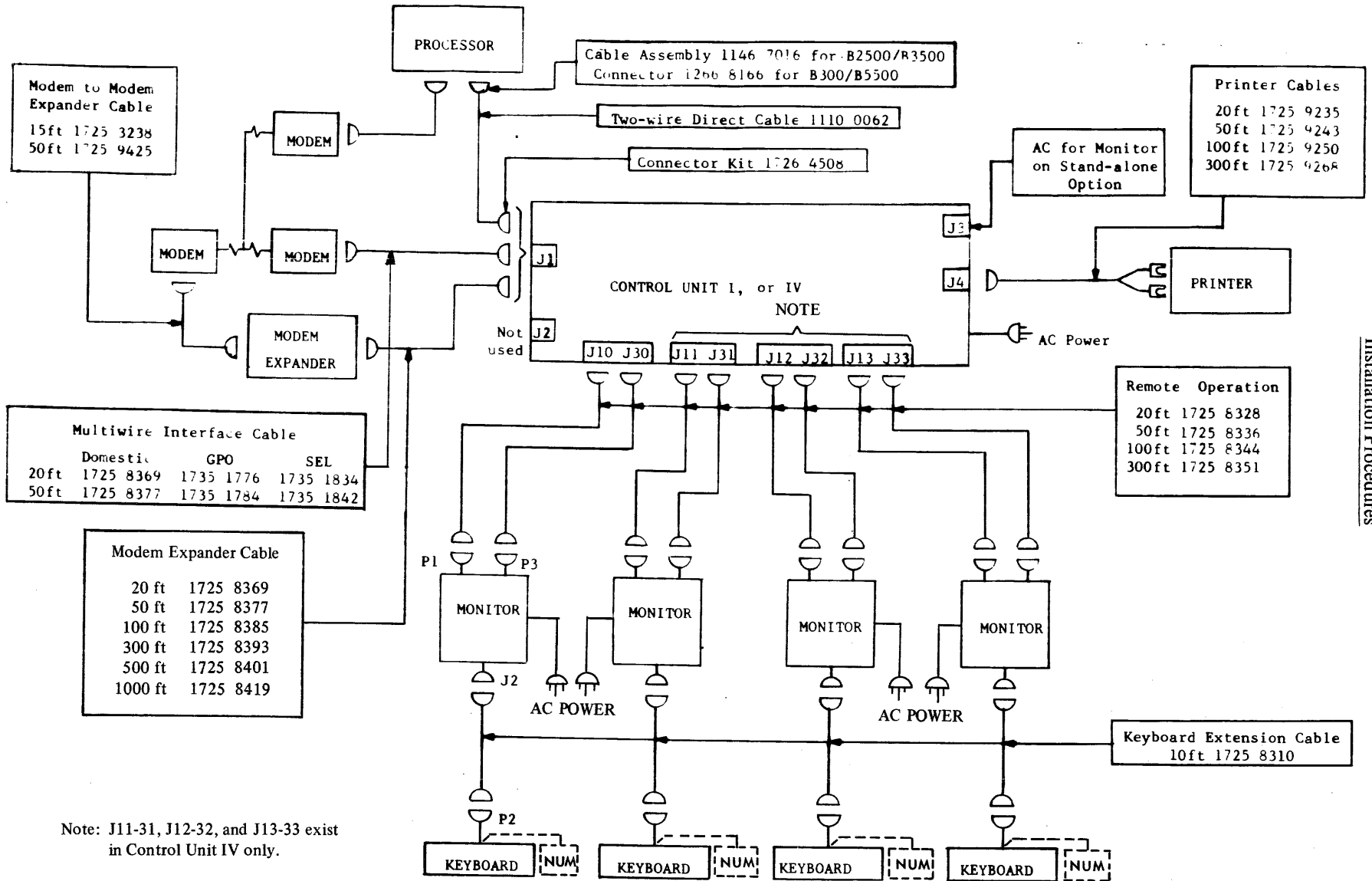
Fig. VI-1 INTER-SYSTEM CONNECTIONS
