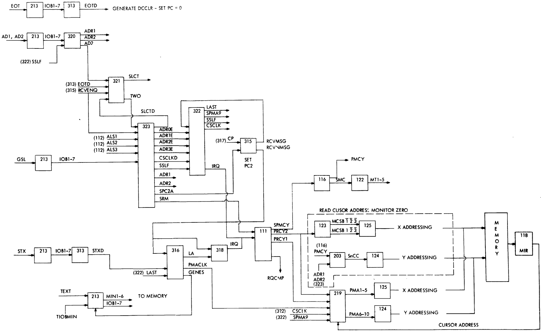
Fig. II-77 GROUP SELECT
