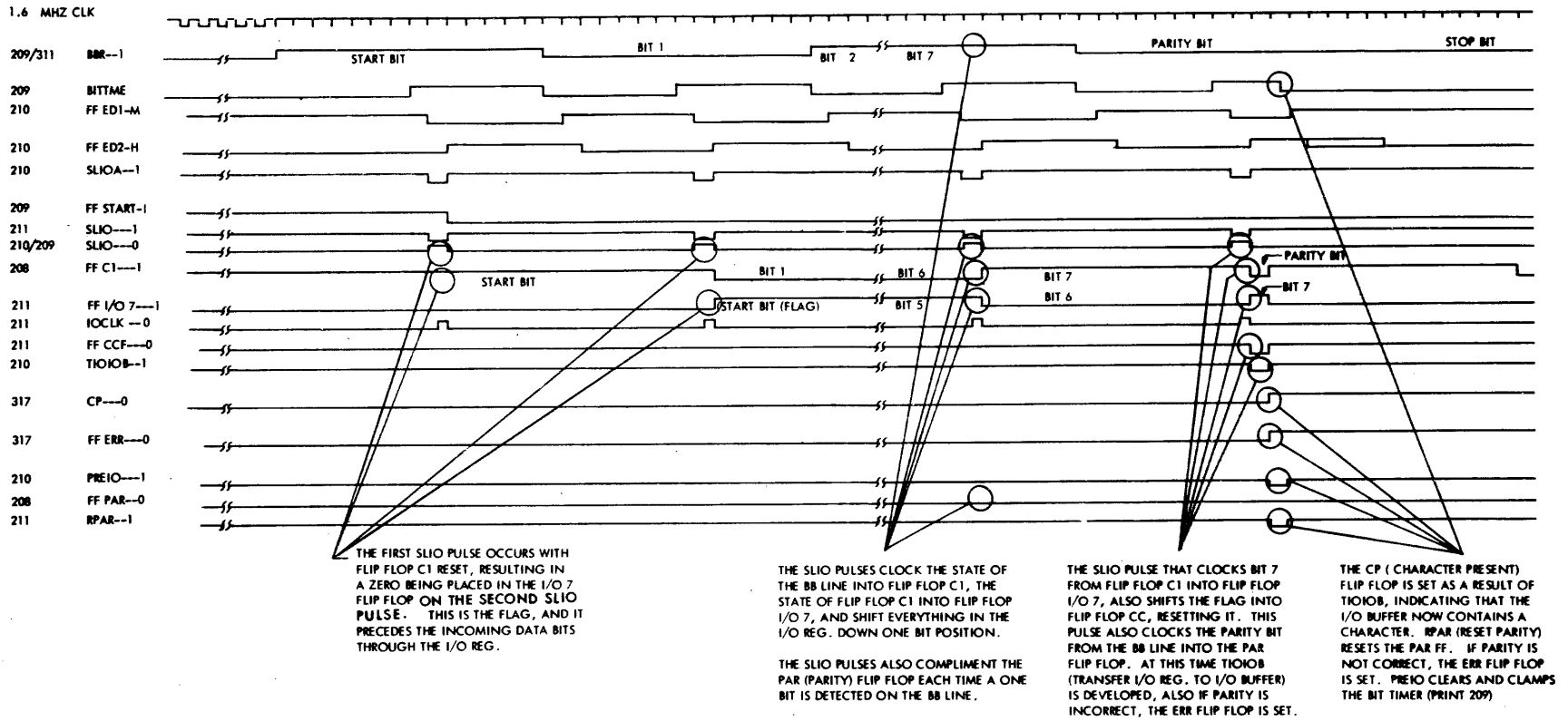
Fig. II-66 I/O REG SHIFT TIMING — RECEIVE
