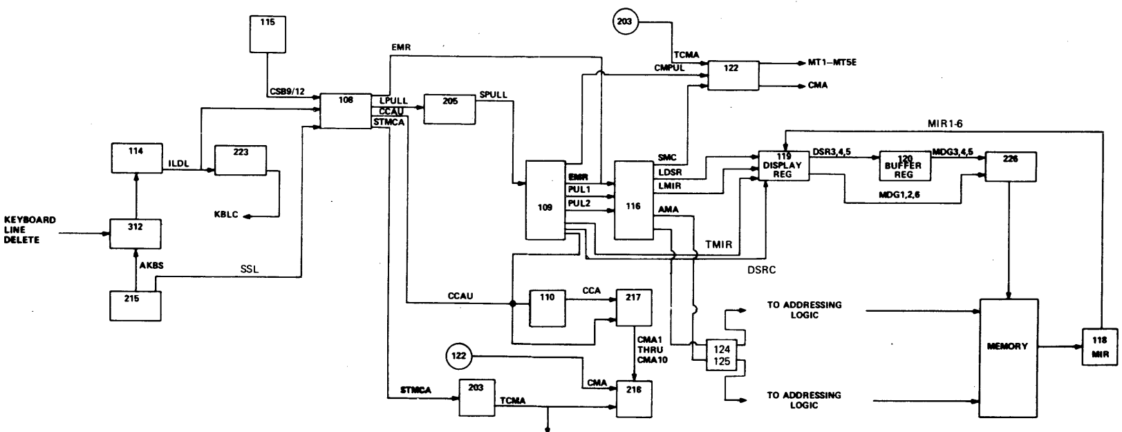
Fig. II-45 LINE DELETE
