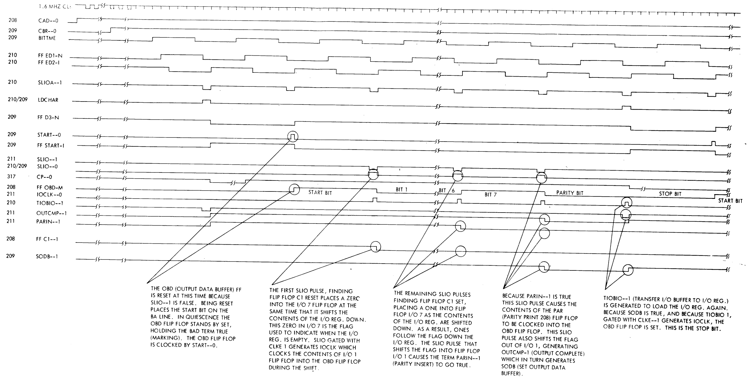
Fig. II-70 I/O REG SHIFT TIMING-TRANSMIT
