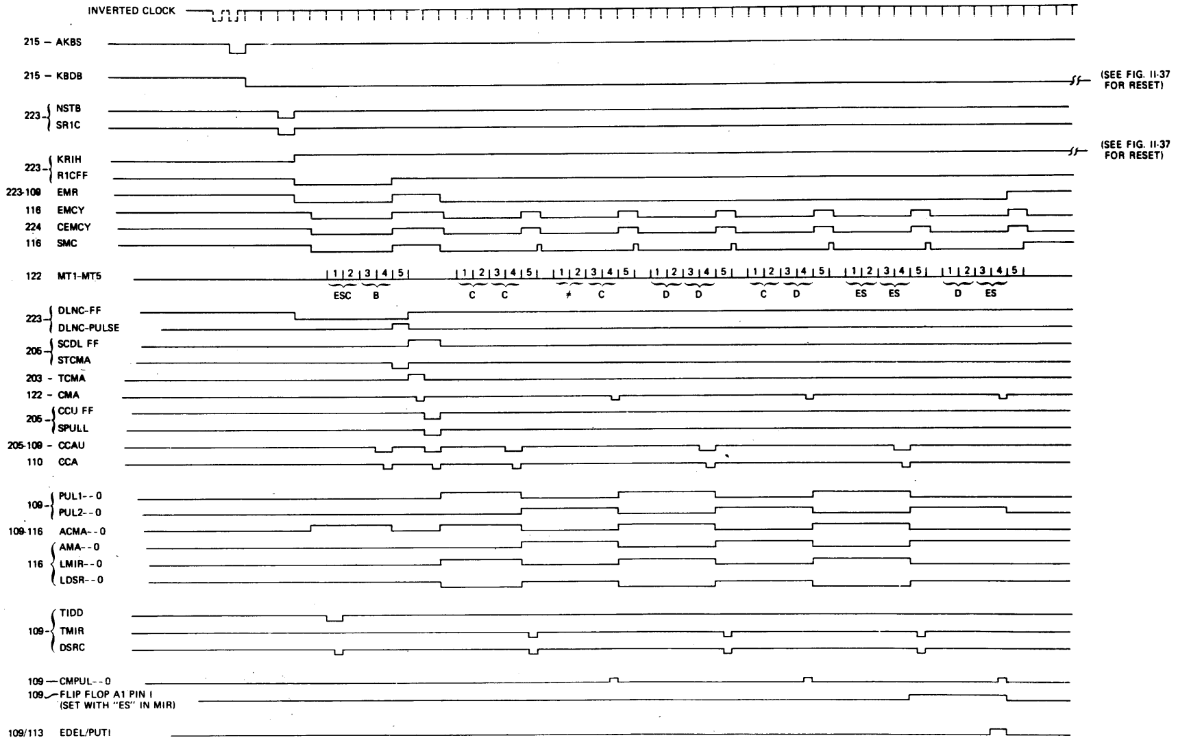
Fig. II-36 PULL BY ONE REPLACE
