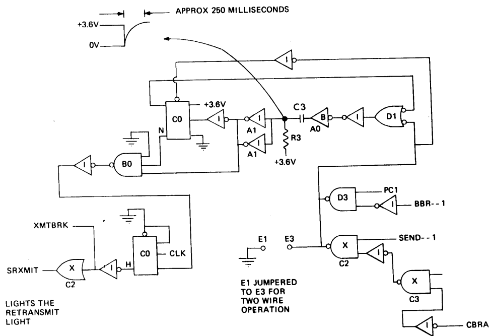
Fig. II-87 RECEIVE BREAK SIGNAL
