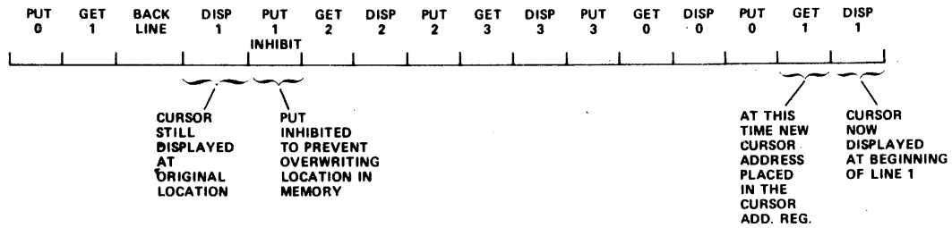
Fig. II-46 BACKLINE TIMING
