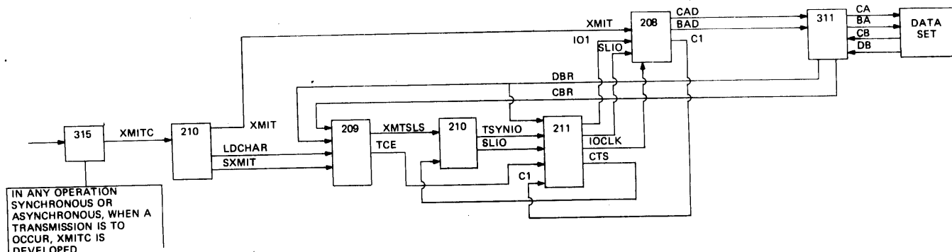
Fig. II-84 TRANSMIT 4 CONSECUTIVE SYNC CHARACTERS
