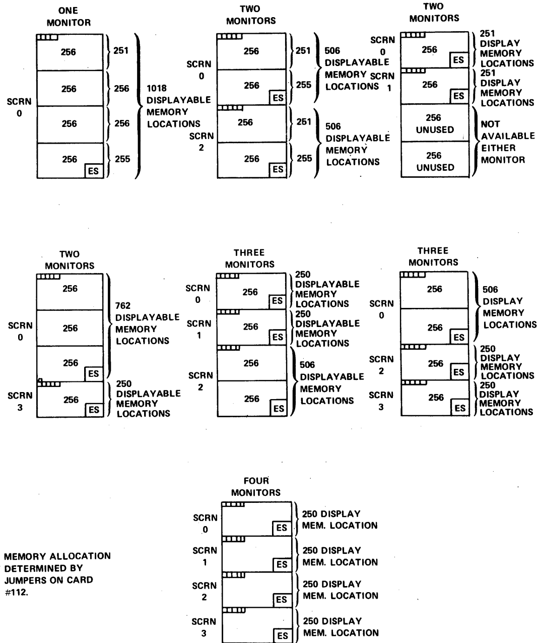
Fig. II-3 MEMORY ALLOCATION
