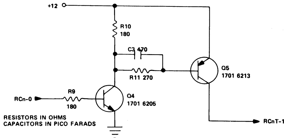
Fig. III-24 TRANSLATOR RECEIVER
