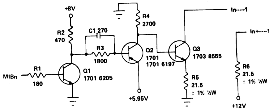
Fig. III-19 INFORMATION DRIVER
