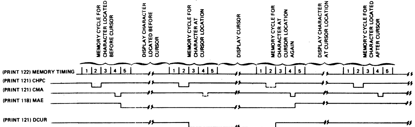
Fig. II-11A CURSOR DISPLAY TIMING
