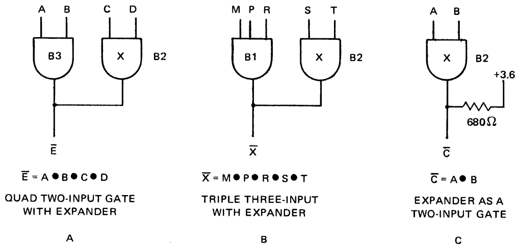
Fig. III-5 EXAMPLES OF EXPANDER GATE
