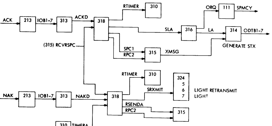
Fig. II-79 POINT TO POINT TRANSMIT
