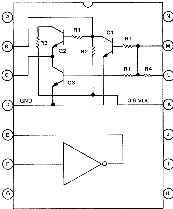
DUAL BUFFER 1701 6163
