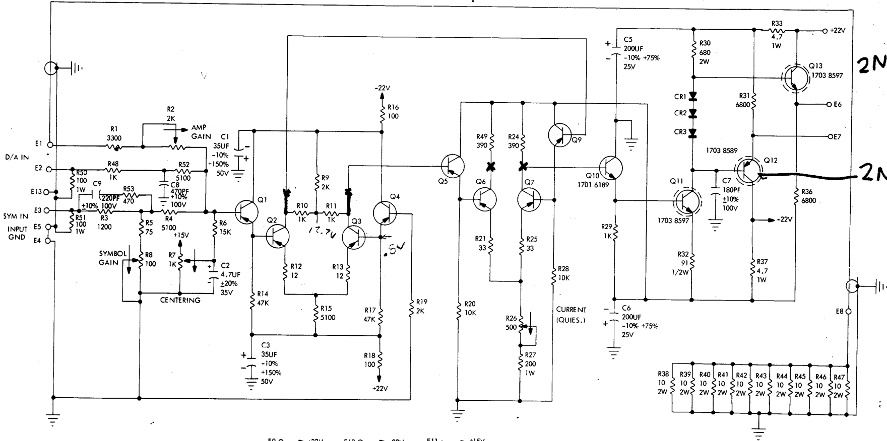
Fig. III-39 DEFLECTION AMPLIFIER - DA
