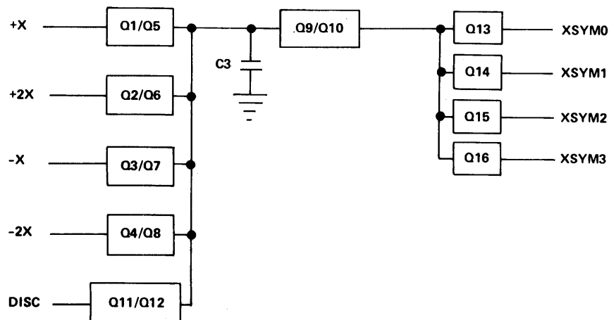
Fig. III-33 BI-DIRECTIONAL INTEGRATOR BLOCK DIAGRAM
