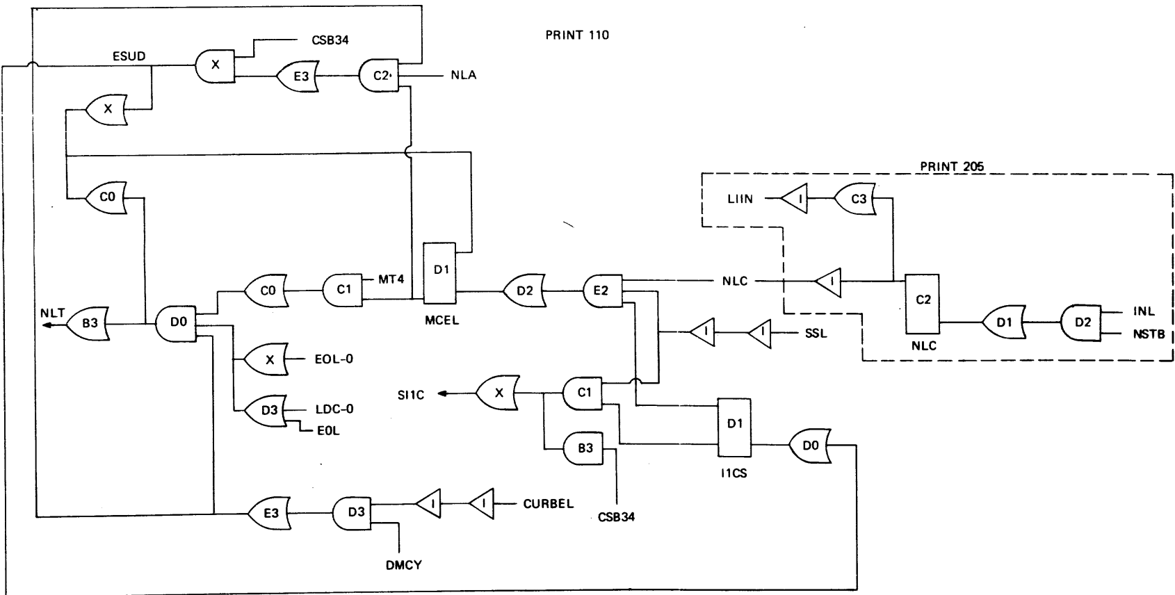
Fig. II-61 NEW LINE DIAGRAM
