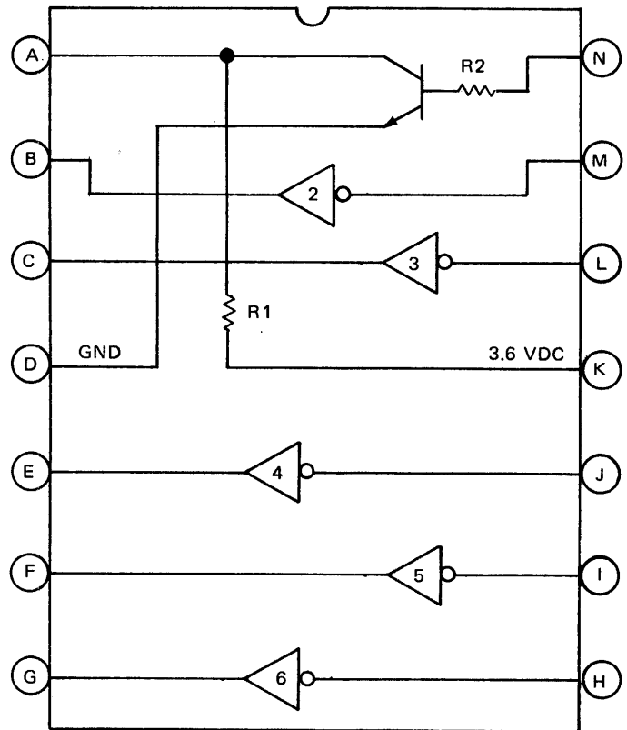
HEX INVERTER
