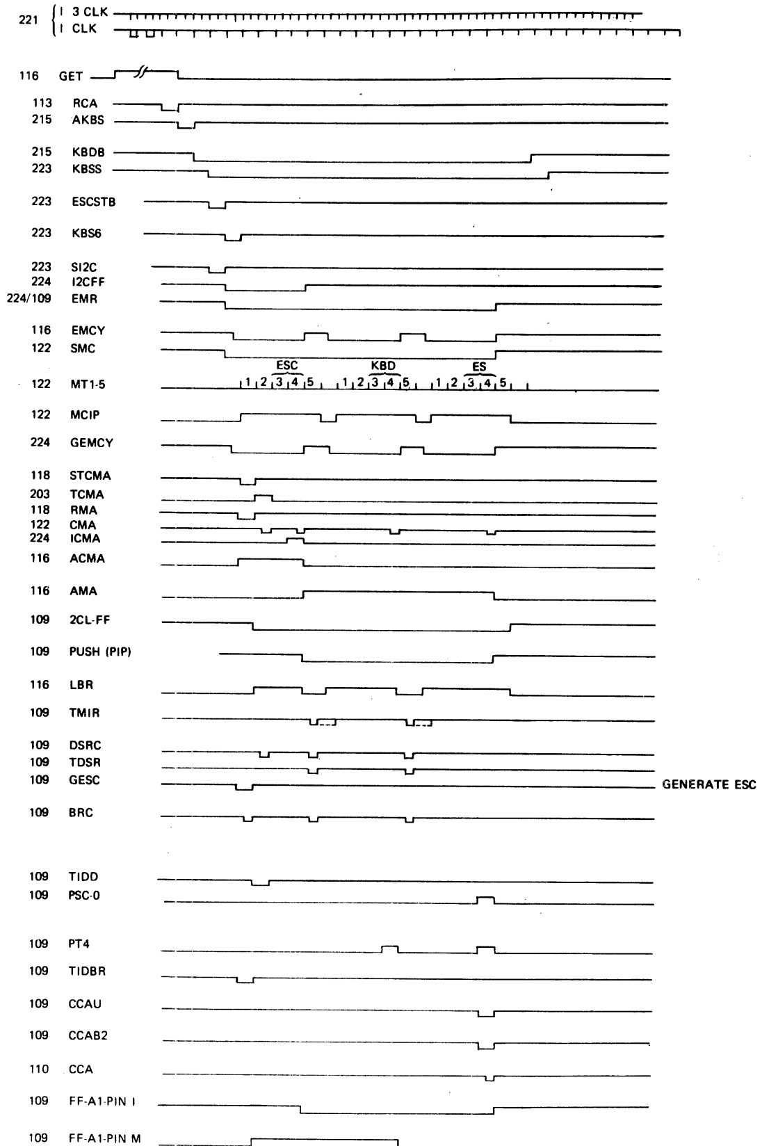
Fig. II-32 PUSH BY TWO REPLACE (CURSOR OVER ES)
