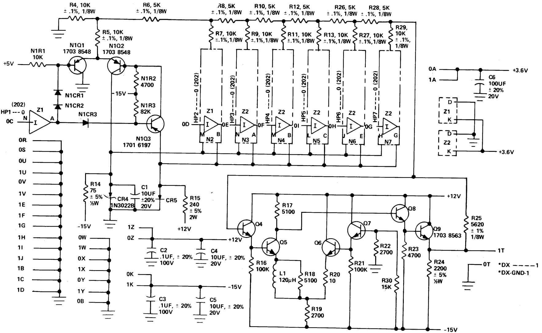
Fig. III-36 X AXIS DIGITAL-TO-ANALOG CIRCUIT SCHEMATIC
