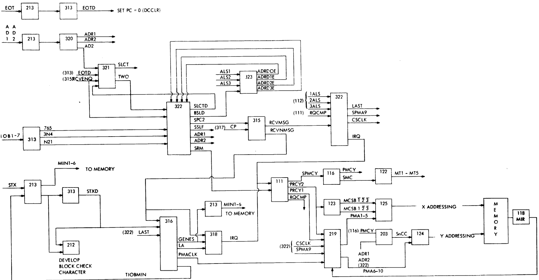
Fig. II-75 BROADCAST SELECT-RECEIVE
