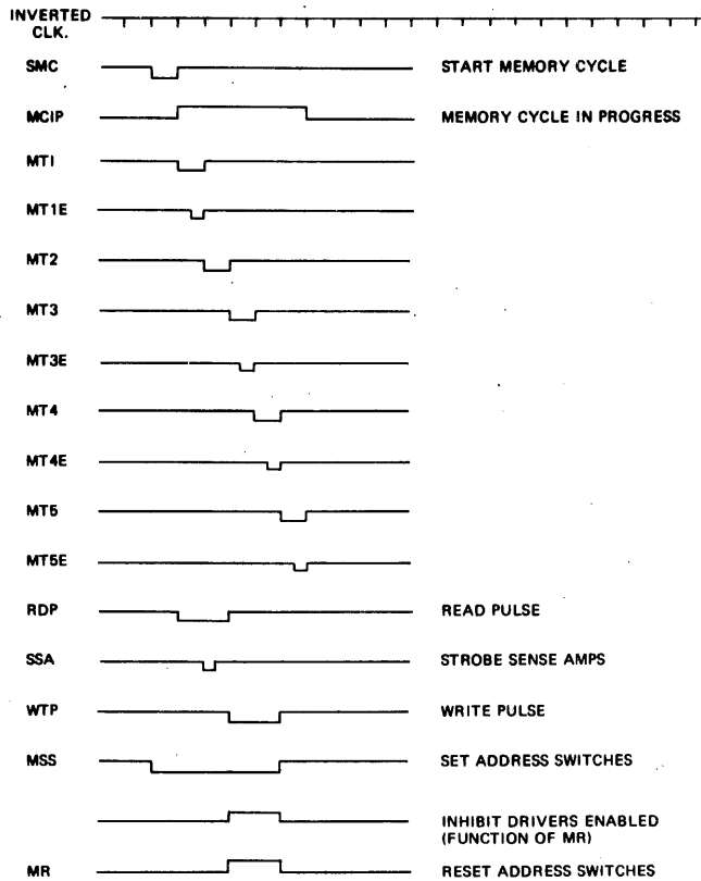
Fig. II-7 MEMORY TIMING
