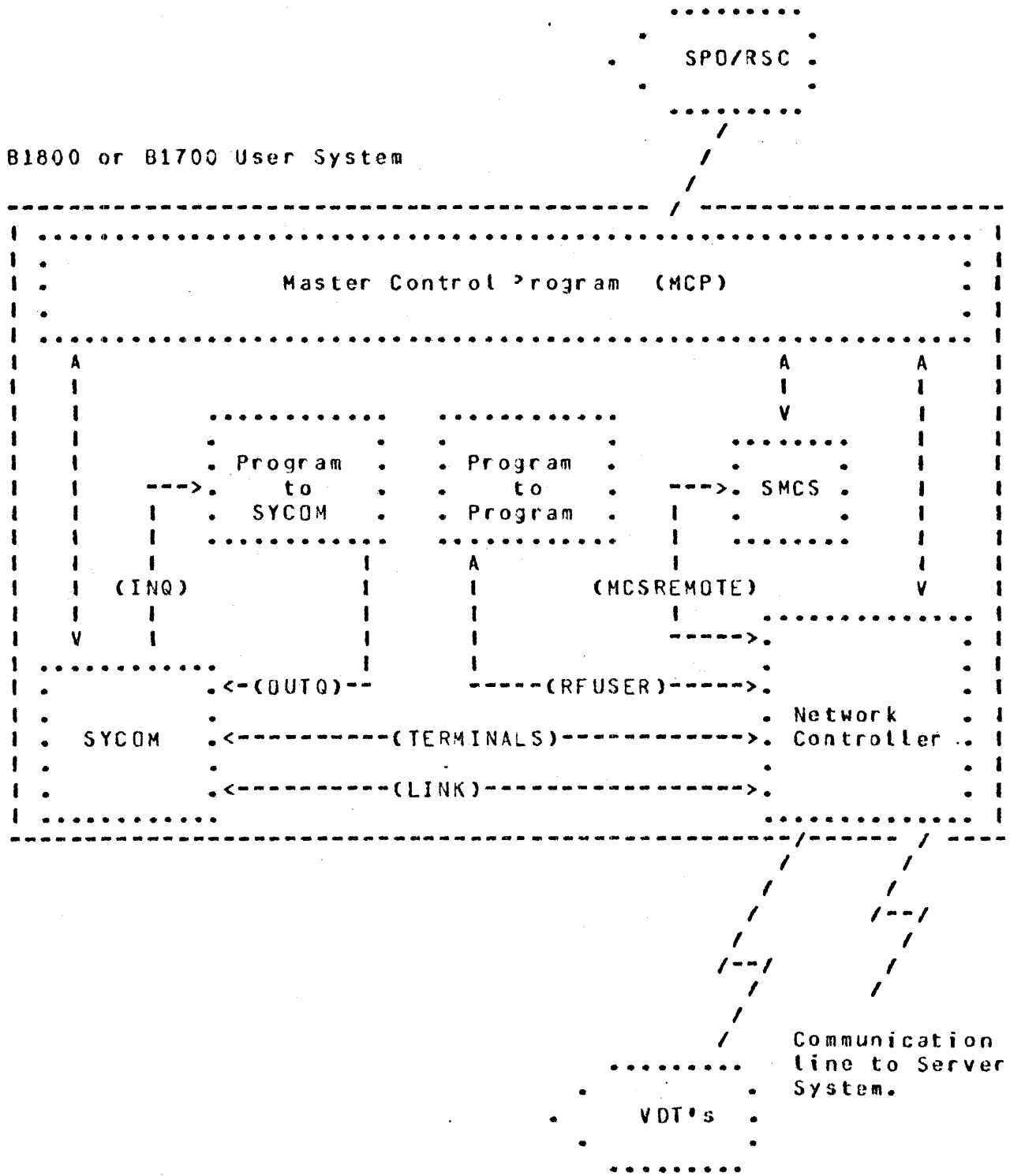
Figure II-11: User System Schematic (SMCS; terminals)
