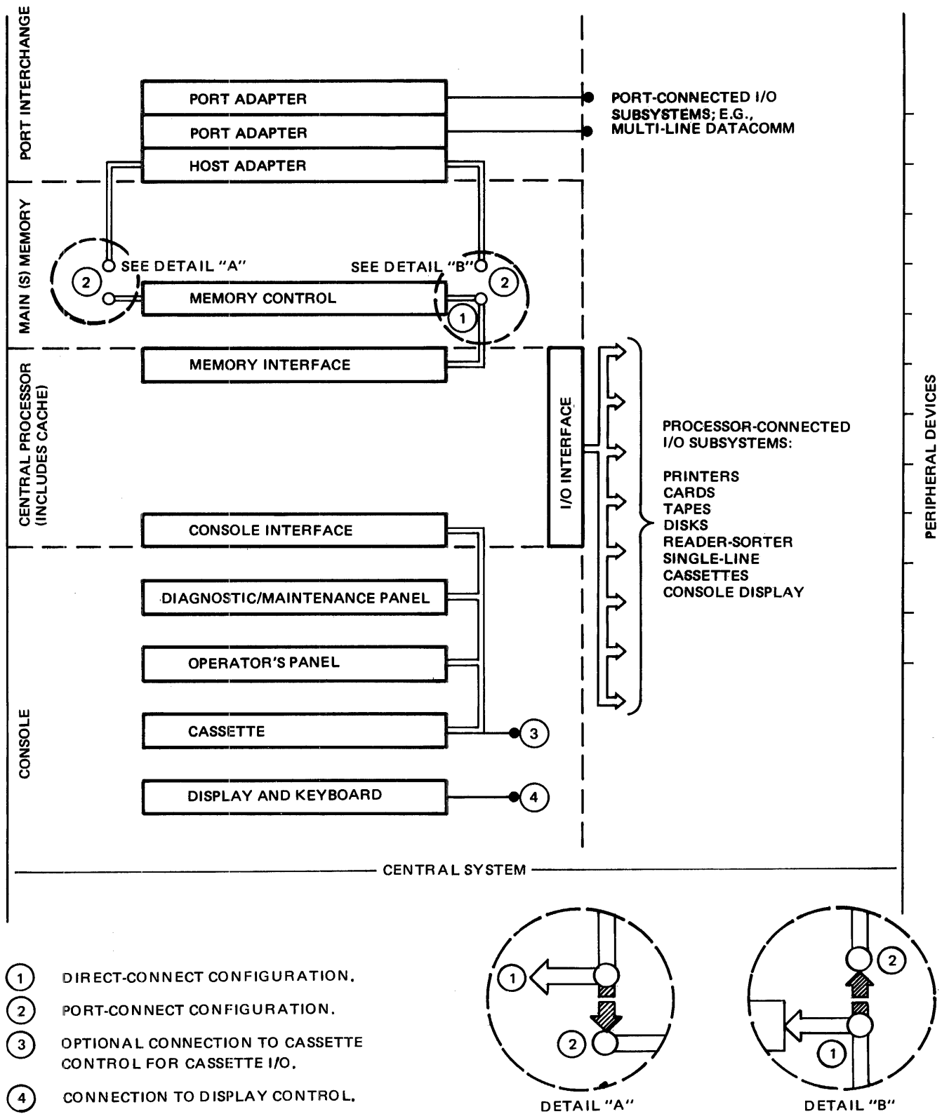
Figure 2-2. Functional Configuration, B 1800 Central Systems
