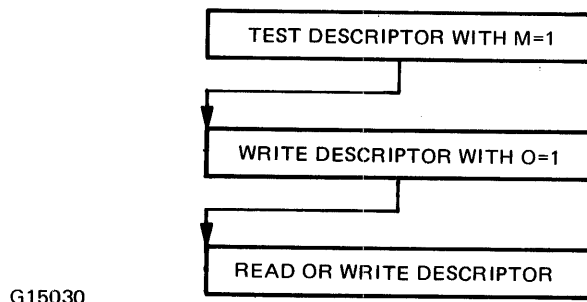
Figure 6-19. Use of Linking for Dialing
