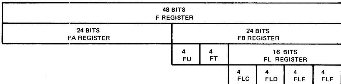
Figure 4-1. F Register and Subregisters
