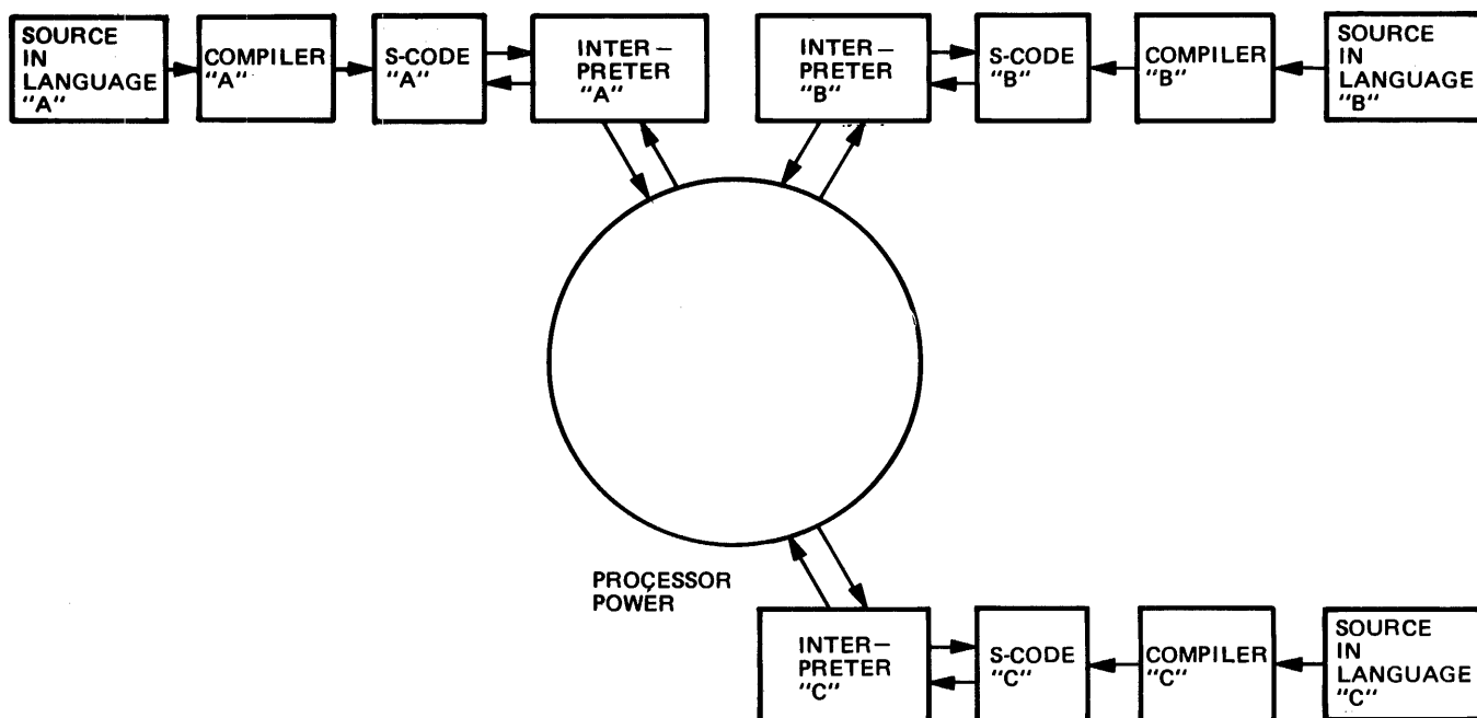
Figure 1-2. B 1800 Approach to Interpretation
