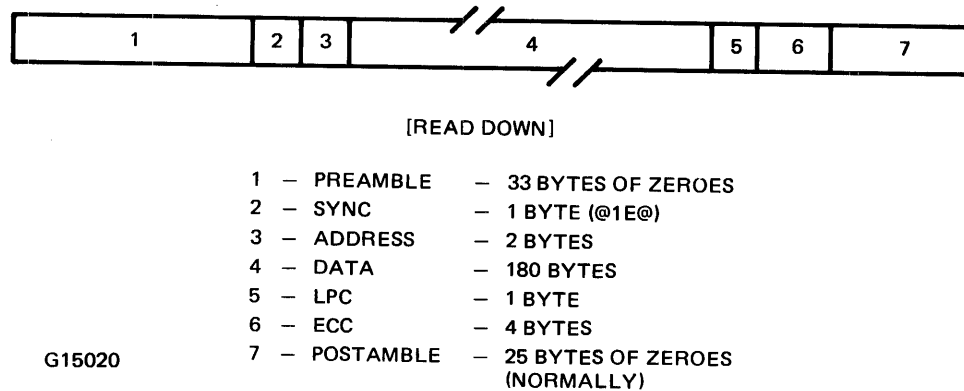
Figure 6-9. Burroughs Cartridge Disk Format
