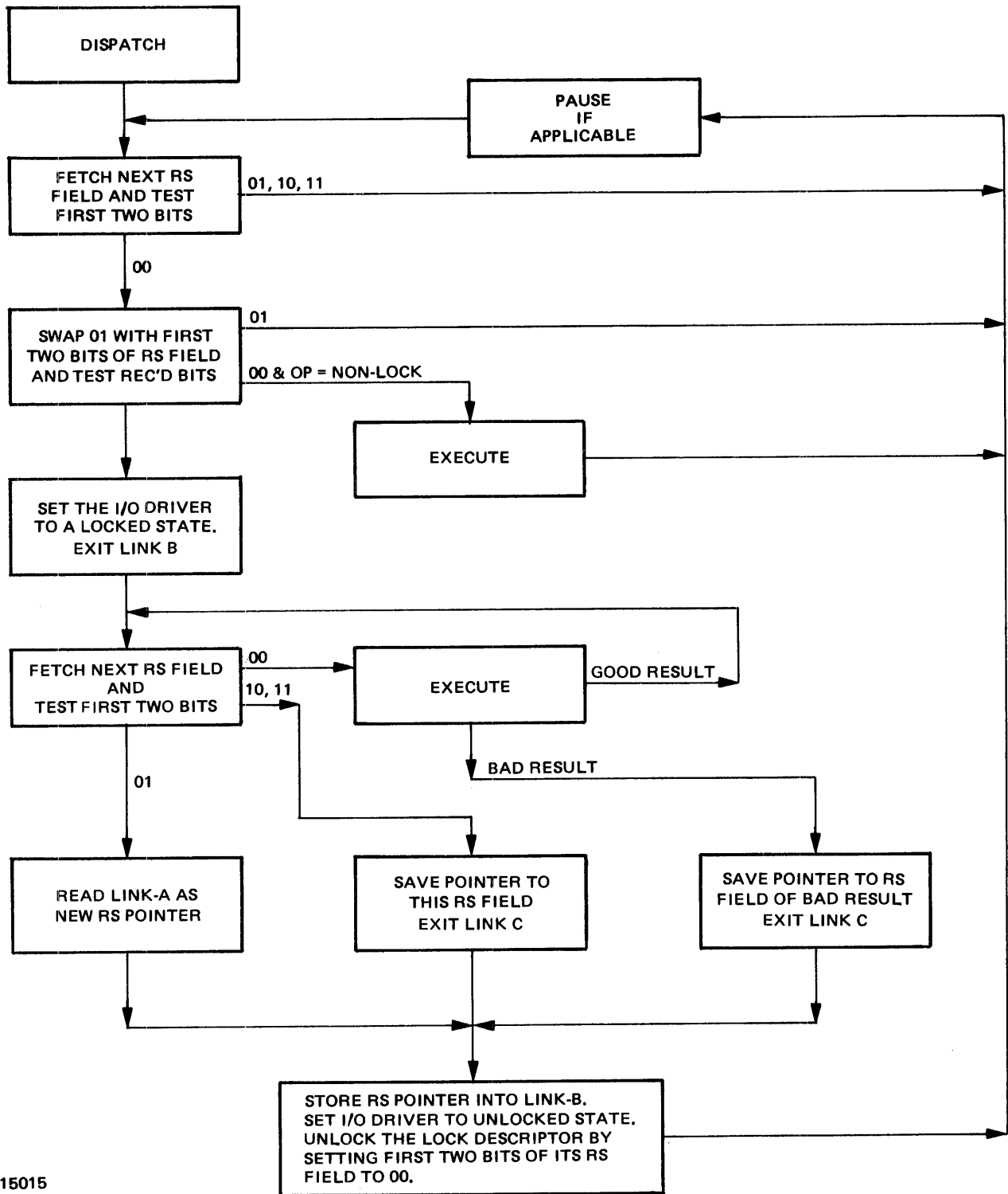
Figure 6-4. Chaining Process
