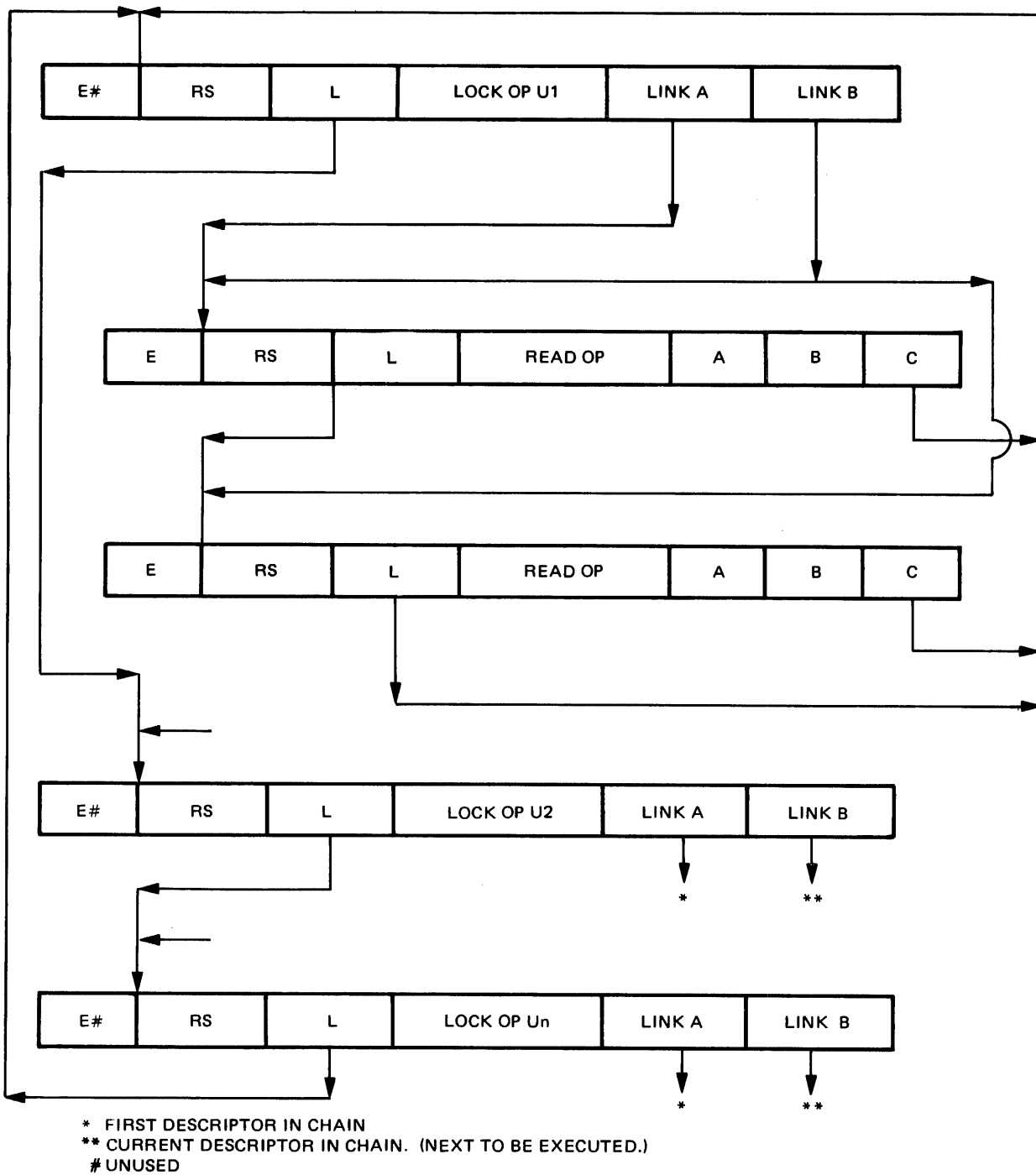
Figure 6-5. I/O Descriptors Showing Linkages
