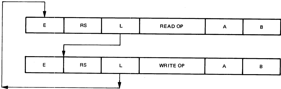
Figure 6-17. Use of Linking for Read Operation
