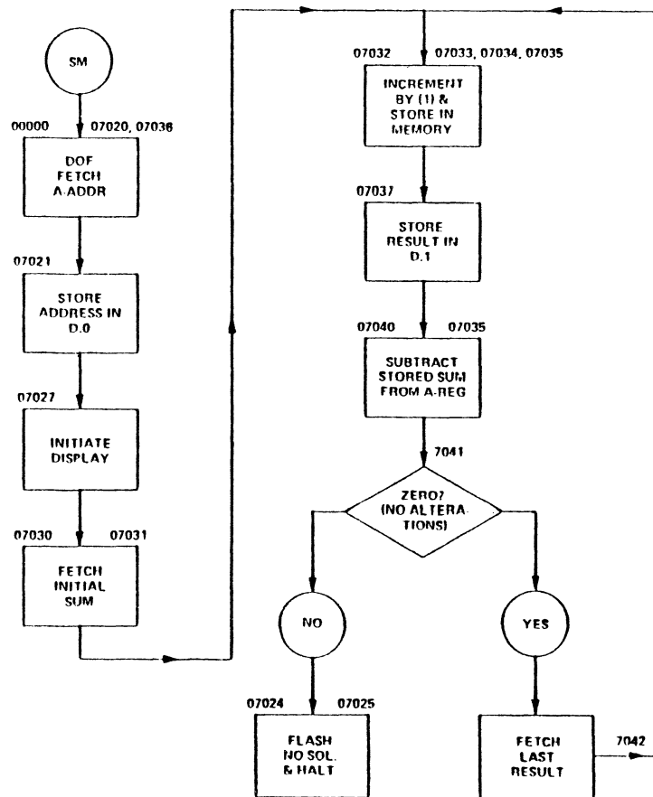
FLOW DIAGRAM, LOOP TEST
