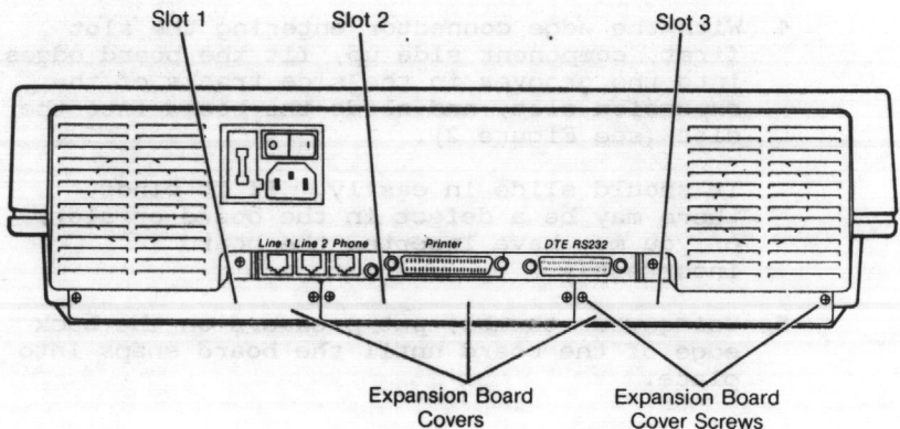
Figure 1 Rear View of UNIX PC
