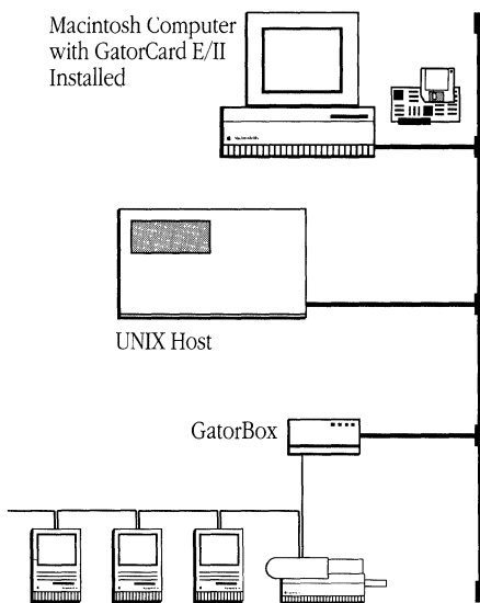
The GatorCard E/II and the GatorBox products provide connections to the Ethernet environment.
