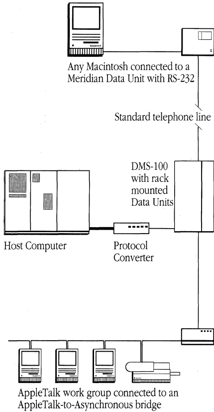
Meridian Data Services provide Macintosh connectivity to other Macintosh computers, mainframe host computers, and modem pools.
