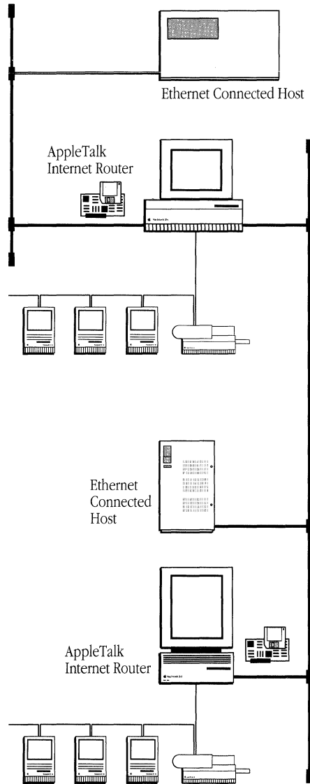
The AppleTalk Internet Router can connect up to eight networks including any combination of LocalTalk, EtherTalk, and TokenTalk interconnections.
