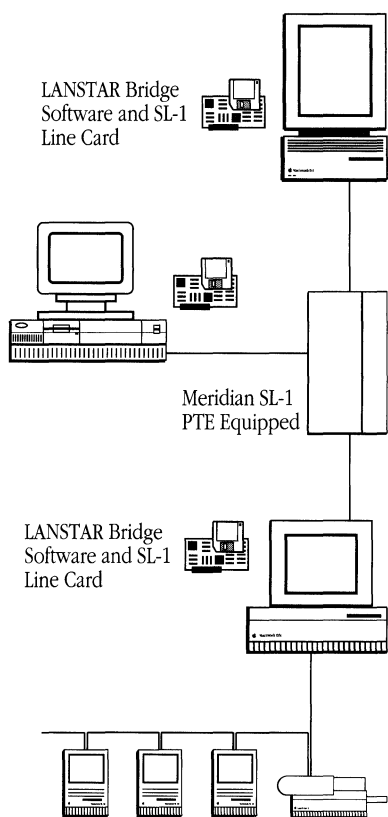
LANSTAR AppleTalk supports up to 2000 feet of twisted pair cabling to each node on the LANSTAR network at speeds up to 2.56 Mbps.
