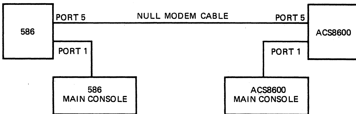
Figure C-2. Uucp Setup
