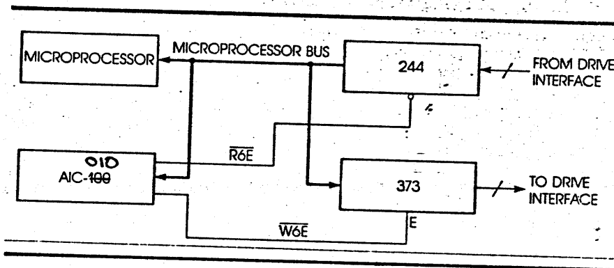
FIGURE 4. AIC-100 REGISTERS 6E AND 6F USAGE
