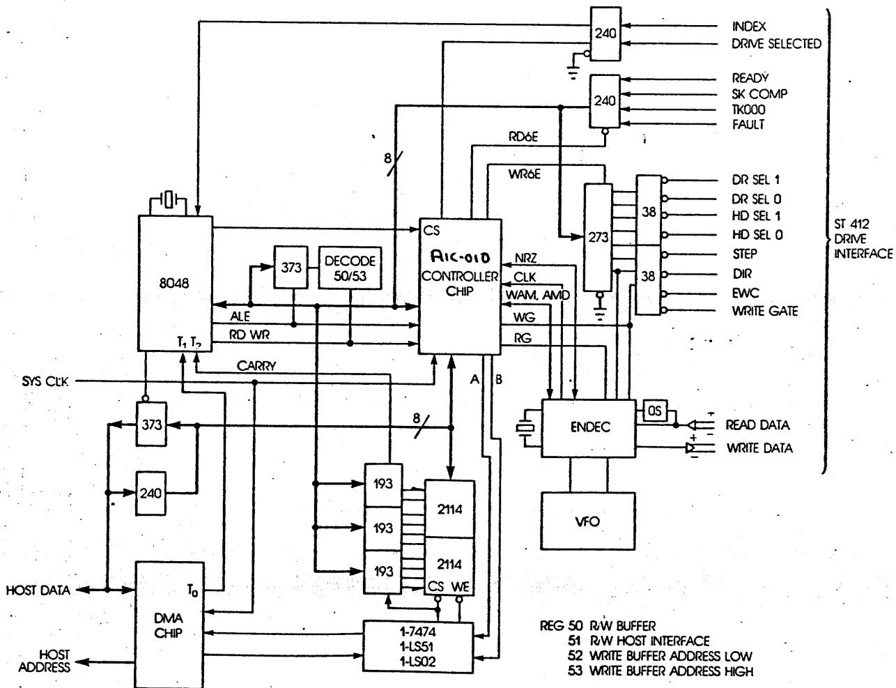
FIGURE 3. AIC-010 ST412 APPLICATION 010
