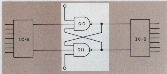
11. Another means of external control: Add gate inputs to circuits with latches.
