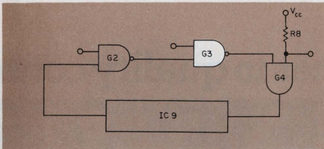
7. Break feedback loops to locate trouble spots. One way to do it is add an extra gate.
