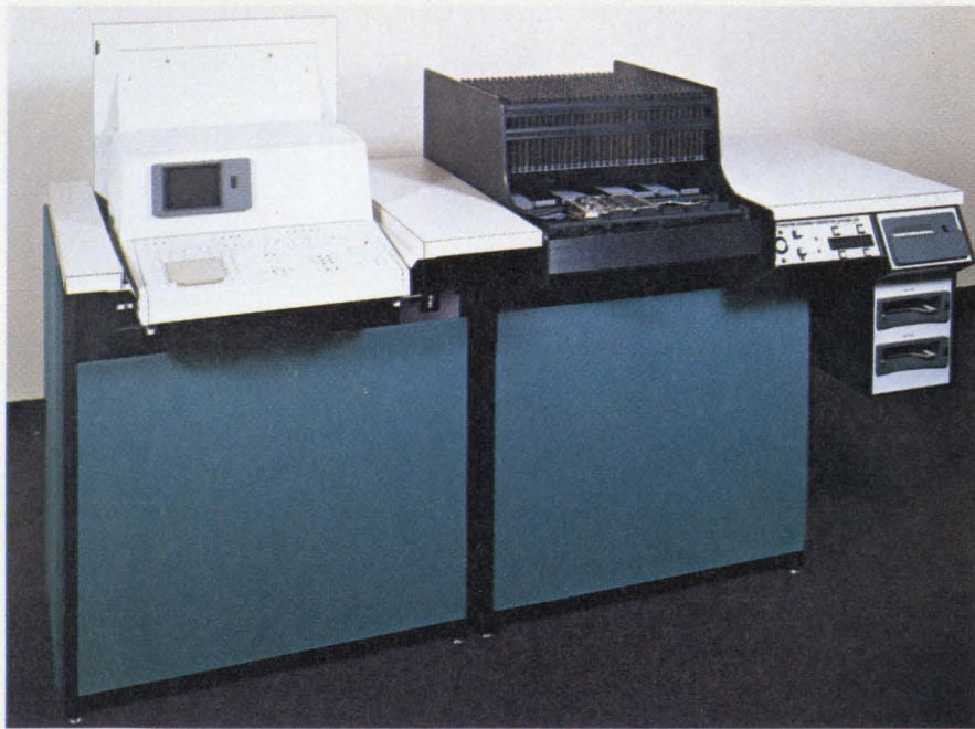
Rubber-tipped pressure rods hold PC boards in place on Teradyne's L529 tester. The system screens out workmanship errors before functional testing.
