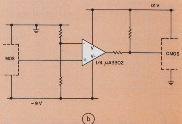
of -20 V and ground (a) or MOS to CMOS shifting for CMOS +12 V and ground levels (b).
