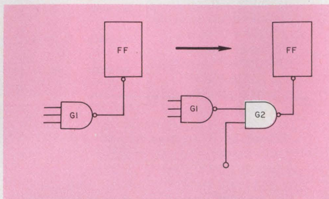
1. Getting circuits started can be a problem unless you add logic for external initialization.
