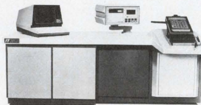
An IEEE-488 interface and 19 programming and control card slots help expand the Faultfinders FF303 in-circuit tester into a functional test system as well.
