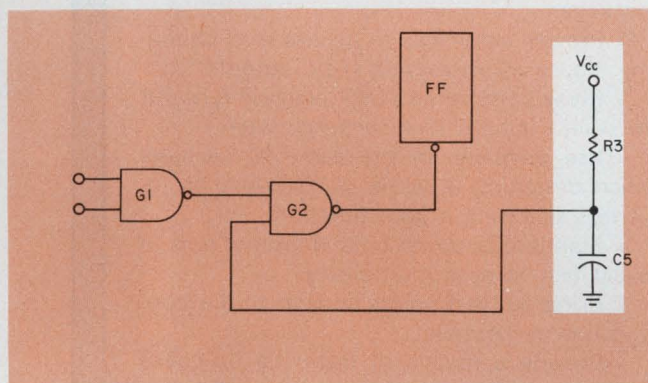
2. No external pins? Add a power-up reset to provide internal initialization.
