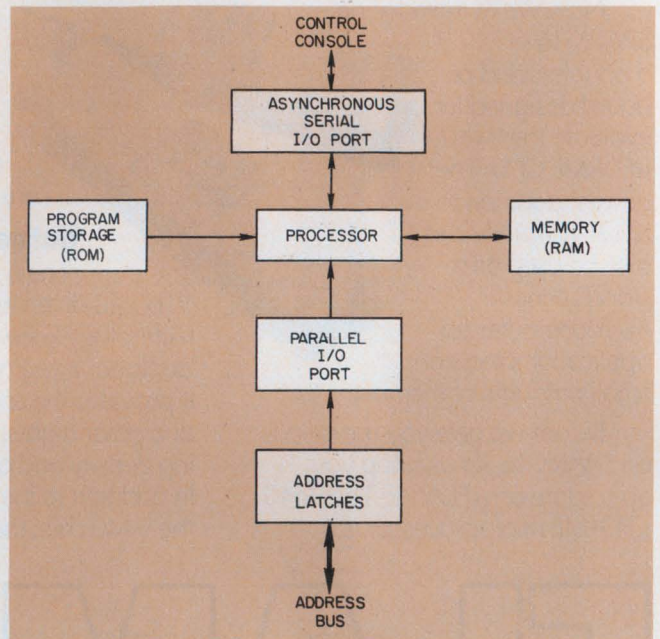
1. The system monitor , a dedicated microcomputer, uses a \mu P, memories and I/O circuits to observe and record activity on the address bus. The 12 most-significant bits of the address bus are monitored.
