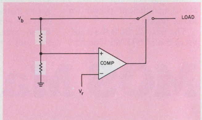
1. Popular load-cutout circuits compare the battery voltage ( V_b ) to a fixed reference voltage ( V_r ). The load is disconnected when the battery voltage gets too low.
