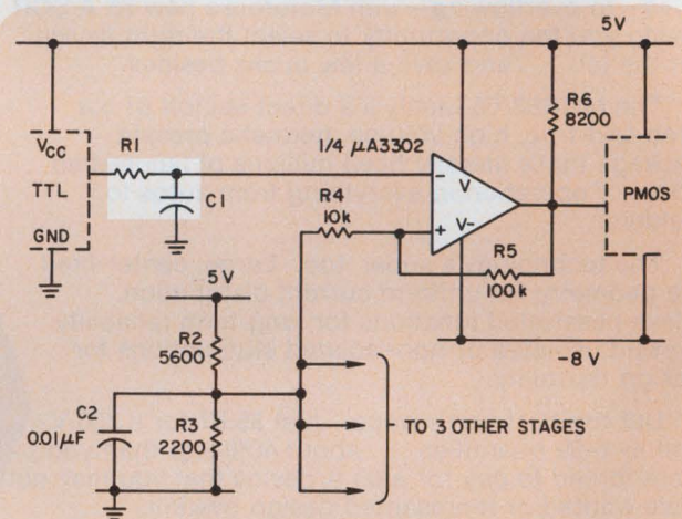
1. TTL outputs can be converted to PMOS logic levels by a \mu\text{A}3302 comparator. The quad device lets you convert four parallel TTL outputs. You can insert time delays in the data paths by selecting appropriate values for the R_1C_1 combinations.
