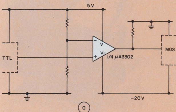
2. The versatility of a quad comparator allows you to use it for TTL to MOS-level shifting for MOS levels
