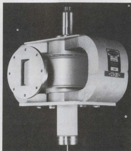
Coaxial magnetron from Raytheon has a higher efficiency and better frequency stability than regular magnetrons but is more expensive.
