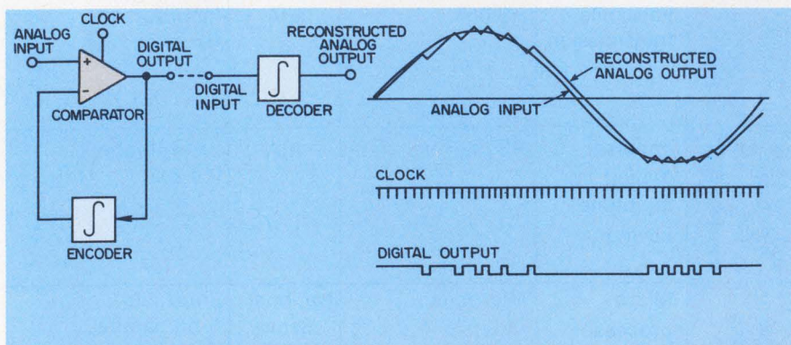
3. The human voice is digitized by this Motorola IC for binary telephone systems by using a clock to sample the instantaneous slope of the signal. ONEs indicate rising slopes, ZEROs falling slopes. At the receiver, the bit stream is integrated to reconstruct the original voice.
