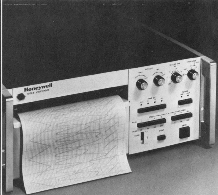
Visicorder Model 1508B
