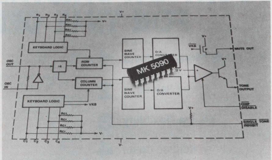
This telephone-dialer chip from Mostek uses a color-TV crystal to derive eight different audio tones. The tones are then mixed on-chip to provide standard dual-tone, multifrequency (DTMF) dialing.
