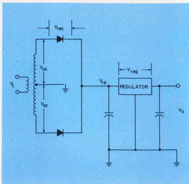
3. In this simple linear supply, the output voltage ( V_o ) is related to the transformer-secondary voltage ( V_{ac} ), the rectifier drop ( V_{rec} ), the ripple voltage ( V_{rp} ) and the voltage across the regulator section of the supply ( V_{reg} ).
