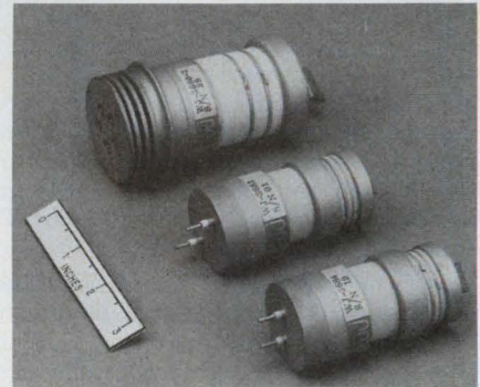
Unpackaged EBS devices from Watkins-Johnson are video amplifiers. The middle tube has 750-V, 7-A peak output.
