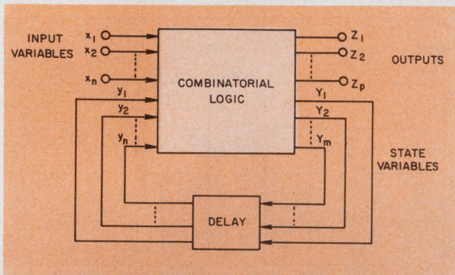
1. Any change of input variables in an asynchronous machine results in an immediate change of state or output variables. The various internal propagation delays are represented by a single delay block.
