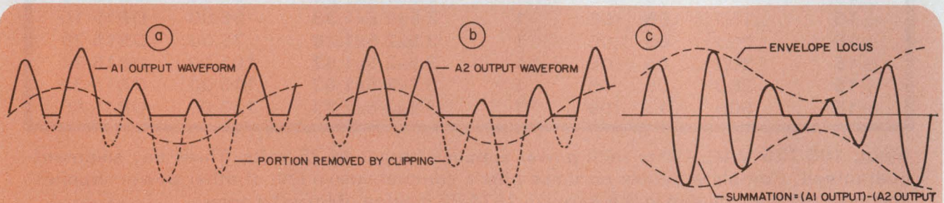
2. Amplifier A_1 clips the negative peaks of the composite input to produce half of the modulated carrier. The output from amplifier A_2 is similar to
