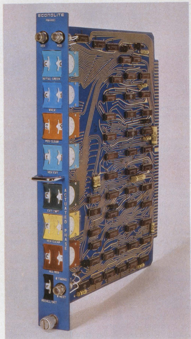
The color and PC compatibility of EECO's 800 series thumbwheel switches combine to make a compact traffic-control module.
