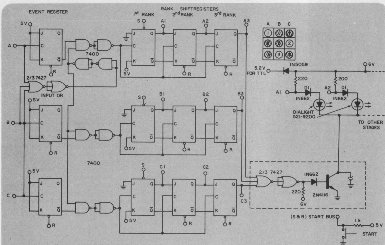
A tie-breaker circuit ranks the occurrence of event pulses with nanosecond precision. A delay in the input-OR circuit is necessary to avoid a race condition and allow the event pulses to toggle the
