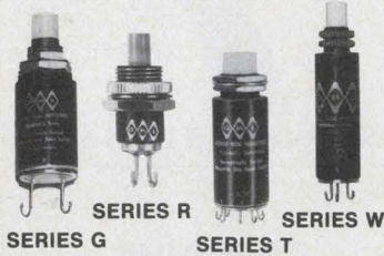
SERIES G SERIES R SERIES W SERIES T Momentary Action and Mercury-Wetted Reed
