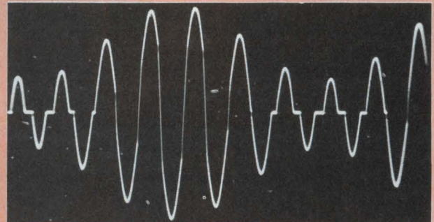
10 KHz CARRIER, 1500 CPS MODULATION, 50% MODULATION, MAX AMPLITUDE 10 V P-P
