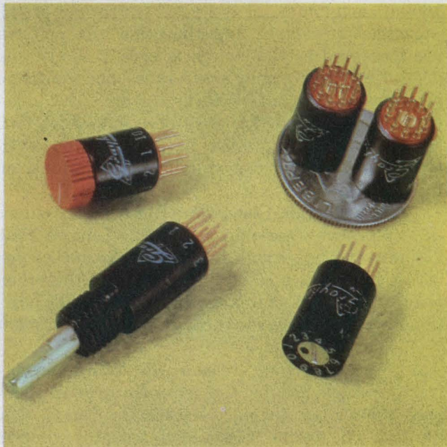
Miniature rotary switches for PC-board mounting include (upper left and clockwise) AMP 642-1 series units, the Minelco SW 37 and 67, the Edison, Daven Dip-switches and the Grayhill Series 75. Other rotary-switch manufacturers are turning out similar types in an almost endless flow.
