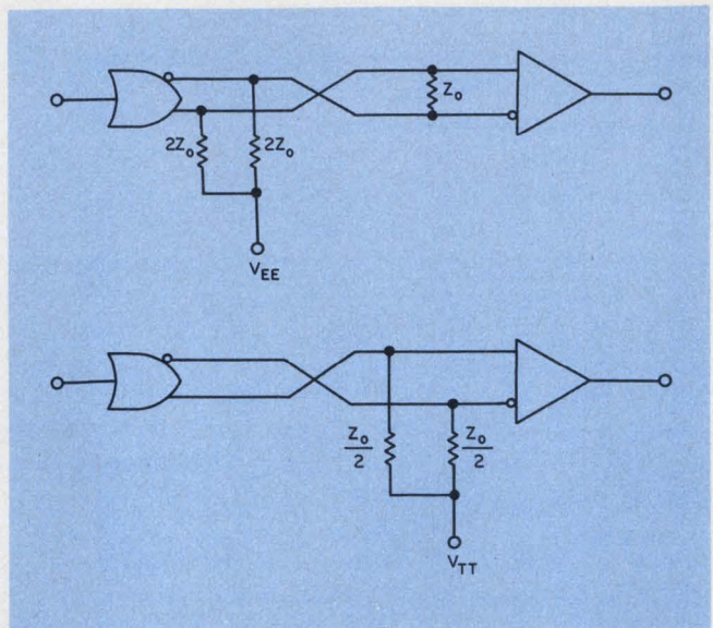
6. Twisted-pair lines should be terminated in one of two ways. Up to 50 ft of line can be driven at greater than 100 MHz.
