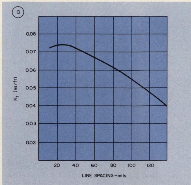
4. Rise and fall times of crosscoupled signals are drawn for the two possible cases: forward crosstalk (a)
