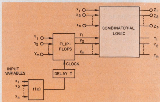
2. Use of edge-triggered flip-flops permits arbitrary state assignments with asynchronous design. Any change of input variable sets off the clock, but also allows time for the original state variables to settle.
