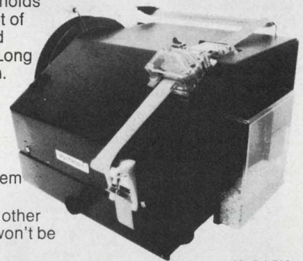
Model 518 Paper Tape Punch Station
