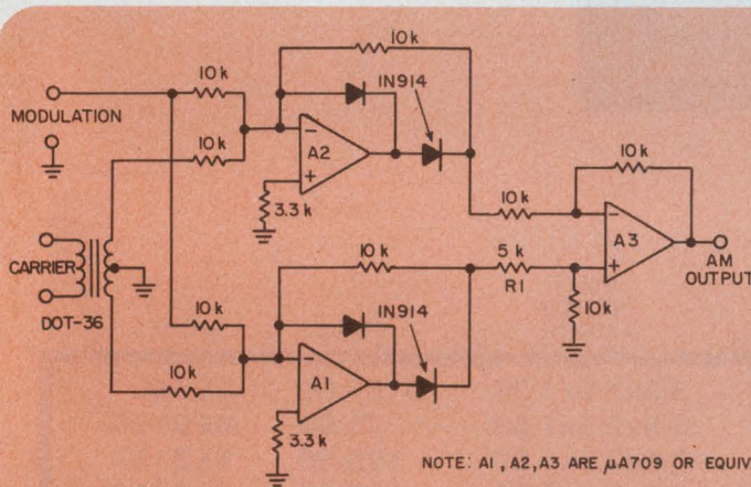
1. A simple circuit with three op amps provides amplitude modulation without distorting the output peaks.
