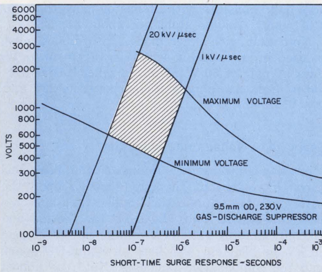
6. The firing point of a gas-discharge device depends upon the rate of voltage rise as well as the absolute voltage level.
