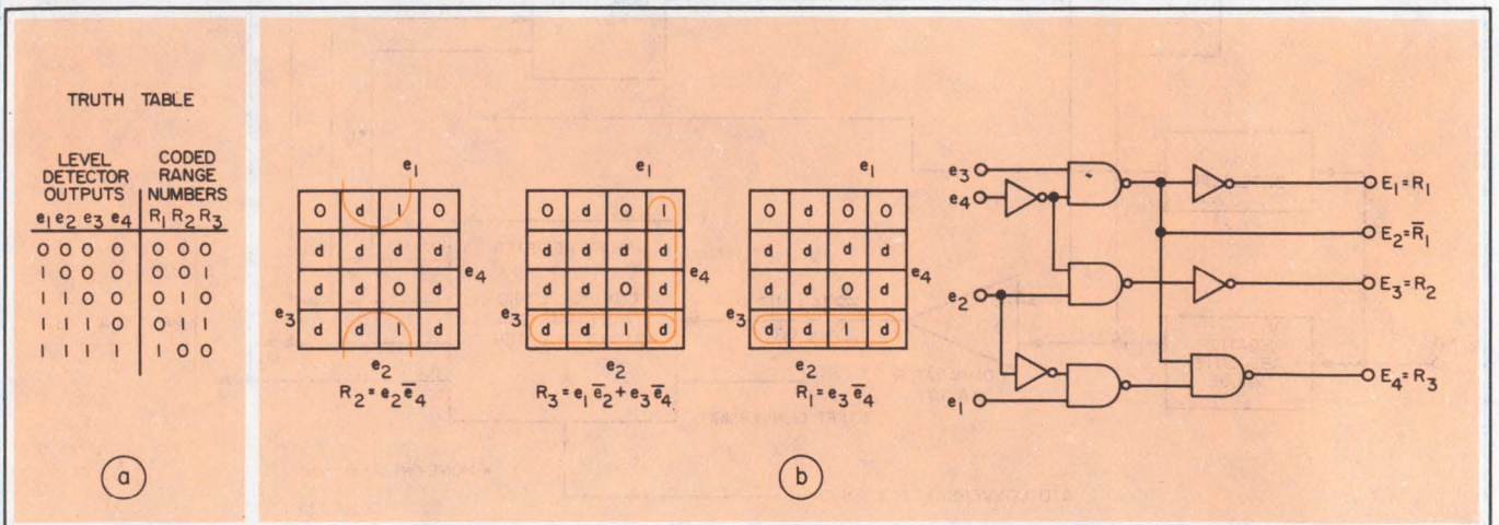
6. The truth table (a) for the exponent logic circuit can be designed using Karnaugh maps (b) to determine the circuit connections needed to set exponent magnitude.
