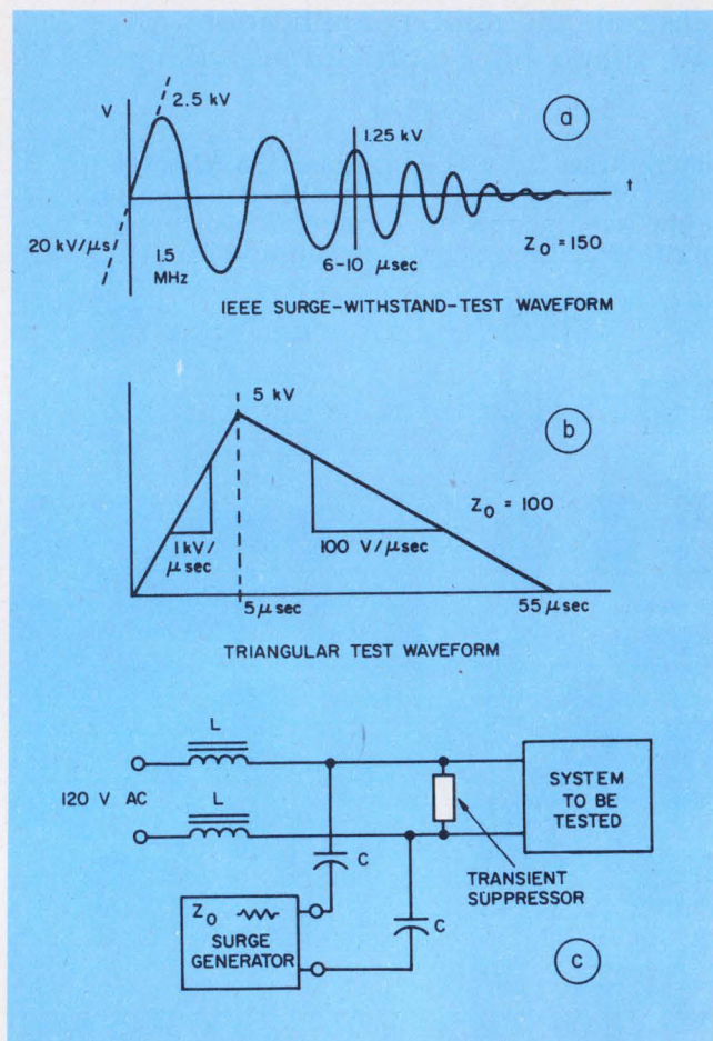
1. Standard wave shapes (a and b) test the response of electrical systems to line transients (c).
