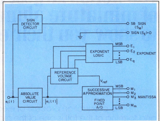
1. A floating-point a/d converter consists of a fixed-point a/d and a lot of auxiliary control circuitry.
