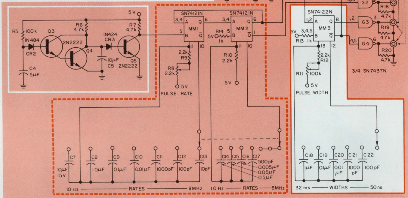
2. One-shots MM_1 and MM_2 act as a variable rate generator, and retriggerable one-shot MM_3 produces variable
