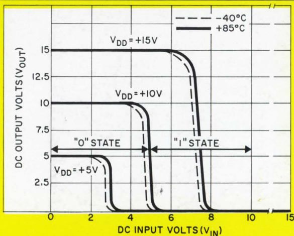
Switching Characteristics for RCA COS/MOS Devices
