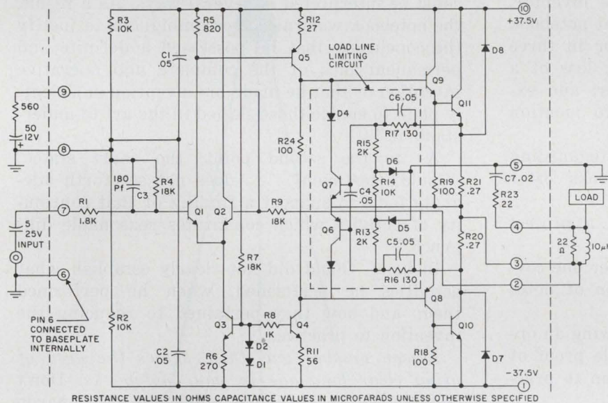
SCHEMATIC OF TA7625A HYBRID POWER MODULE.
