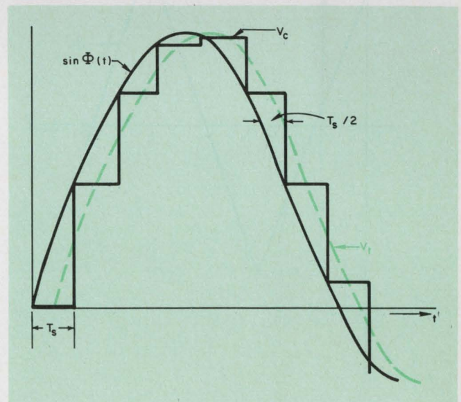
2. A time delay of T_s/2 is introduced by the sample-and-hold circuitry, if \Phi(t) is a sinusoid with f \ll f_s/2 . V_c is the staircase output of the sample-and-hold circuit; it becomes V_t after low-pass filtering.
