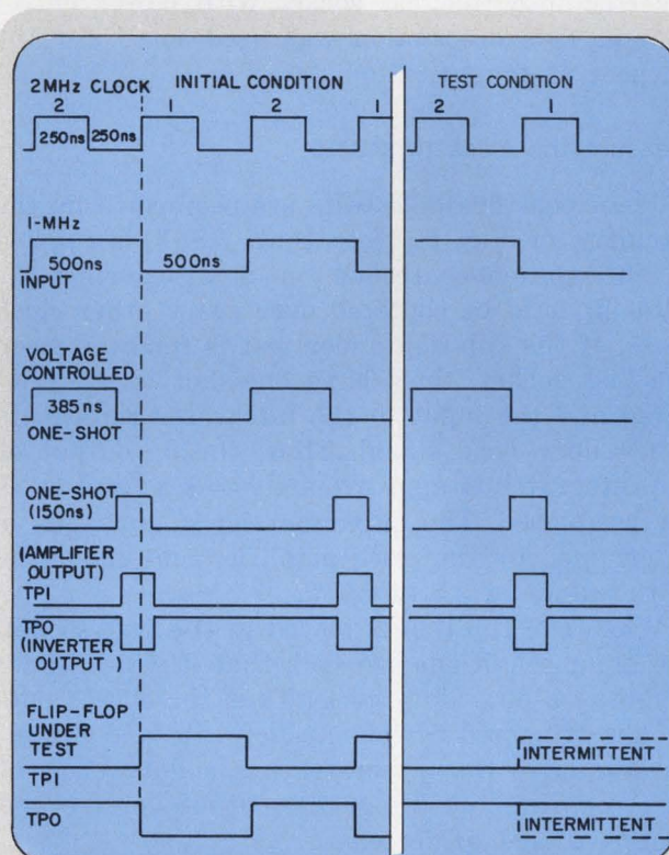
4. The preset test circuit of Fig. 1 accepts the 2-MHz clock, divides it down to 1 MHz, and applies the result to the voltage-controlled one-shot. The output of this one-shot, after inversion, triggers the 150-ns one-shot on its falling edge. Thus the rising edge of the output of the 150-ns one-shot is delayed from the 1-MHz clock by an amount determined by the voltage-controlled one-shot (VCOS). This delay is adjusted by the circuit until the flip-flop under test ceases to toggle.
