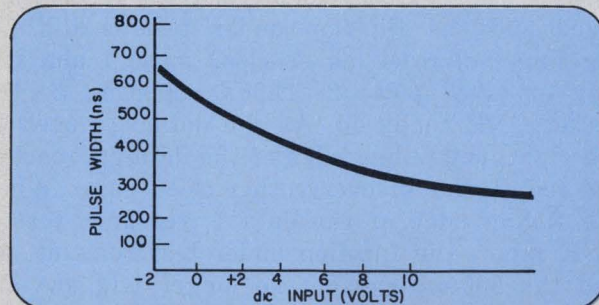
3. The voltage-controlled one-shot provides pulses with width inversely proportional to the dc voltage received from the integrator, and is essential to the operation of the feedback loop.
