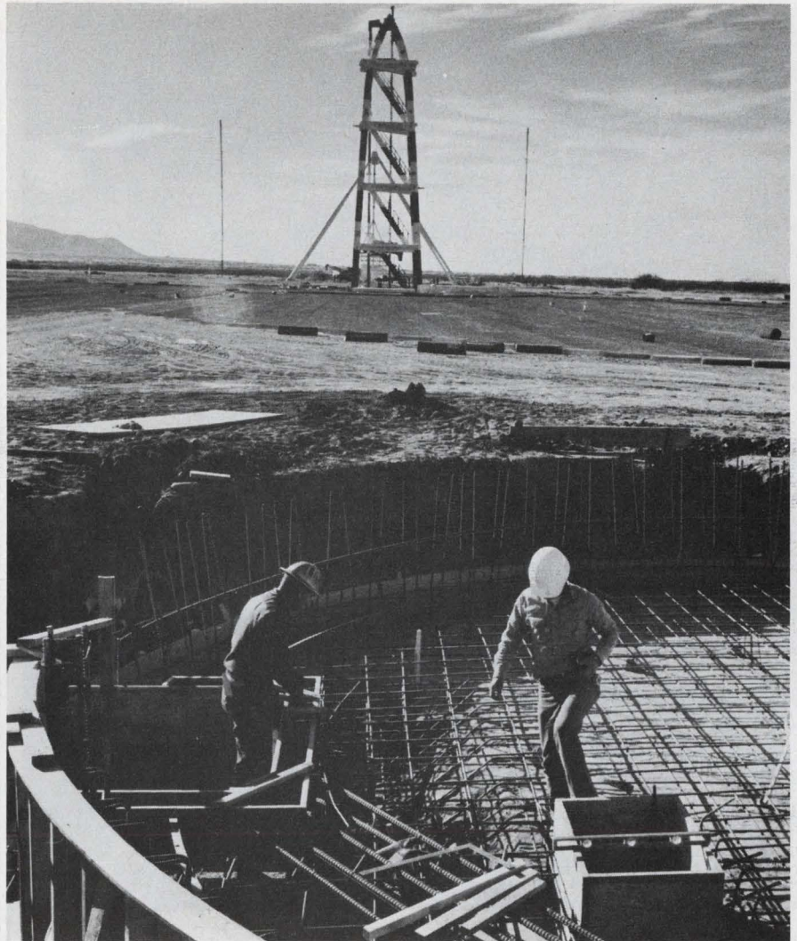
When this turntable is completed, vehicular radio antennas will transmit to five receivers in the 100-foot tower 500 feet away. Buried steel-wire mesh will provide a swamplike or saltwater environment to the transmission.
