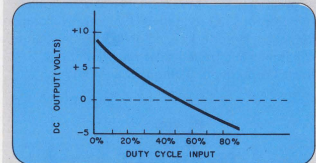
2. The integrator is a simple circuit composed of an op amp and a few discrete components. It provides an output, inversely proportional to the input duty cycle, which is used to control the pulse width of the voltage-controlled one-shot.
