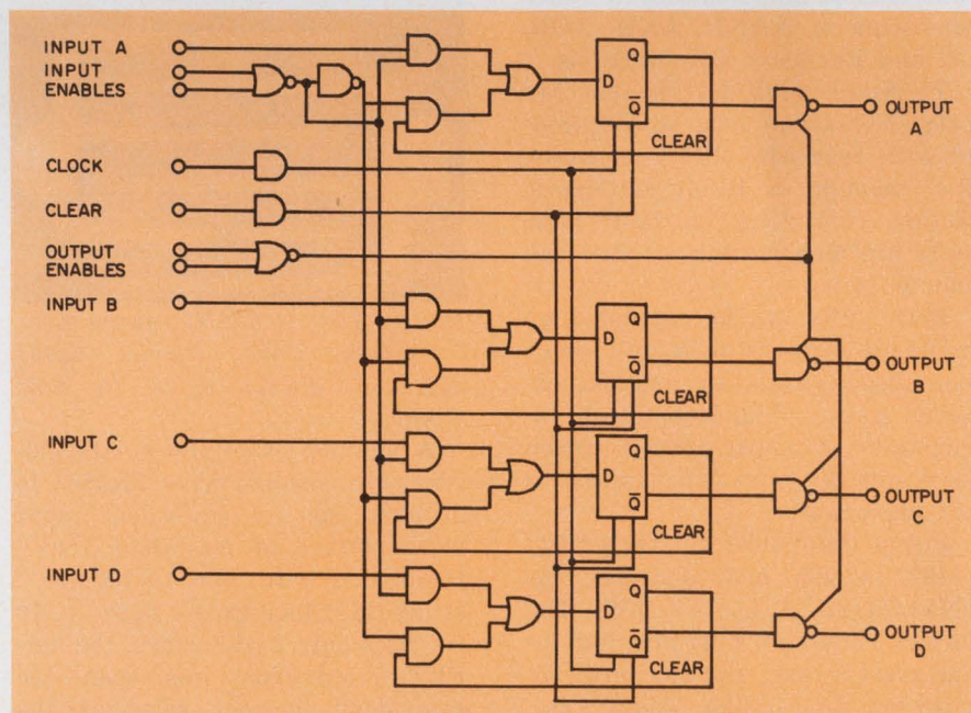
TTL quad D flip-flop with three logic states lets its outputs be tied together directly, without using an OR gate. A third transistor on each of its outputs makes possible a high-impedance state besides the conventional low-impedance ON state and low-impedance OFF state. CIRCLE NO. 250
