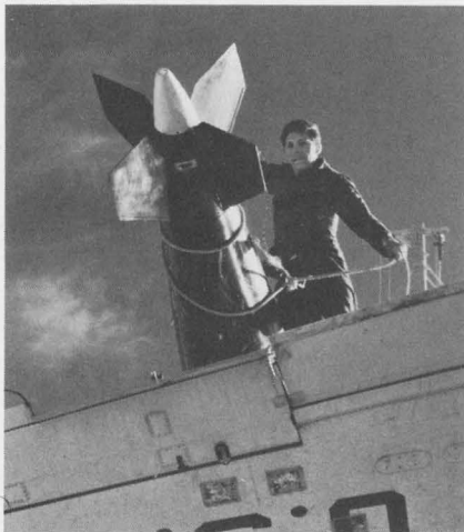
Operator straps an electronic jammer on to wing of Army's Mohawk to measure its effectiveness.
