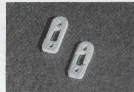
Hole .0775 \pm .0025 \times .180 \pm .002 Hole Center .329 \pm .003
