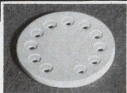
Holes .060 \pm .002
