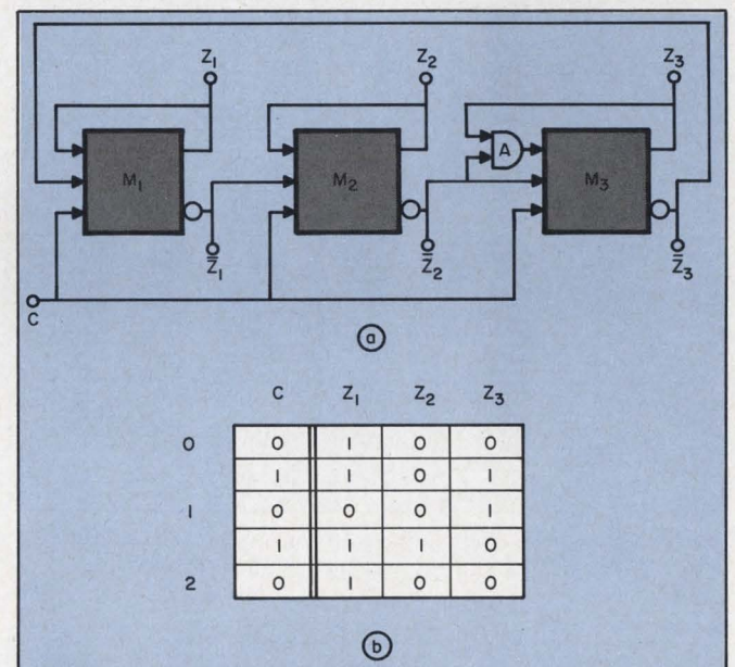
5. Binary counter uses an additional AND gate to inhibit Z_3 (a). After two counts, the output states (b) return to their original setting.
