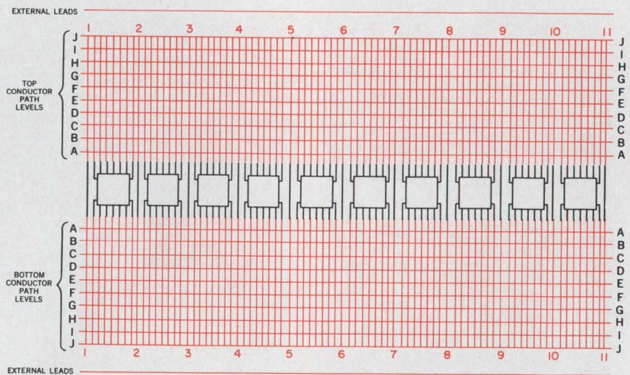
Customer designs interconnections by filling in this form. Any lead may be connected to any other. Engineered Electronics Co. then makes its stick directly from this drawing. The firm says this method holds initial design charges down to as little as $85.
