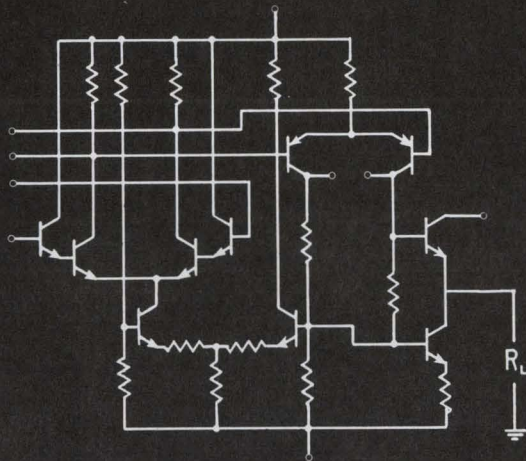
Westinghouse WS 161
