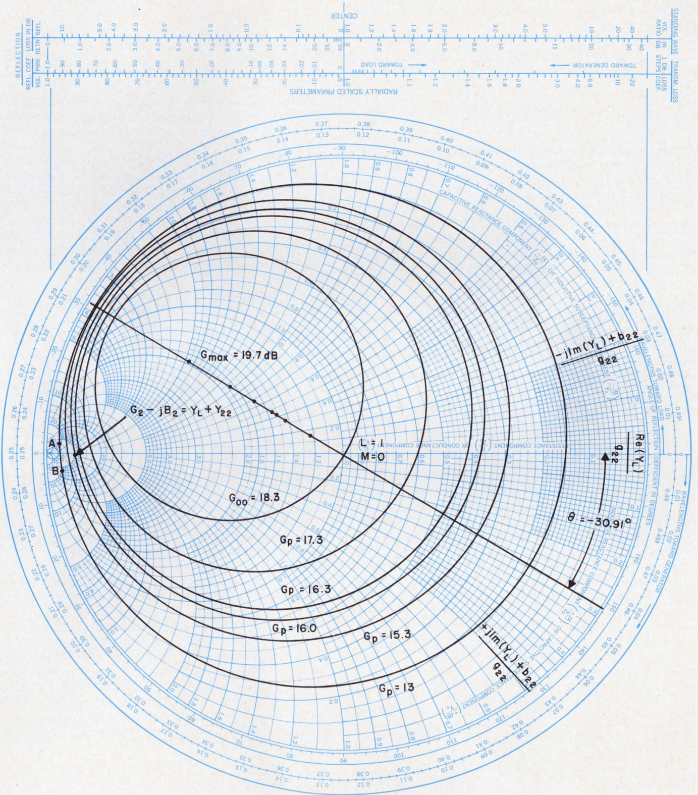
4. Smith chart with superimposed equal-gain circles relates stability, gain, bandwidth and sensitivity for amplifier analysis. Points A and B are used to find the desired load circuit for the design example.
