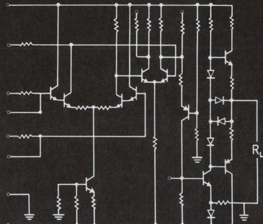
Westinghouse WM 174
