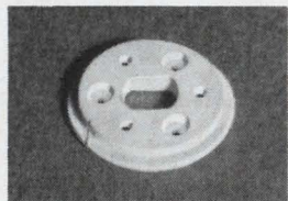
Center Pin .250 \pm .003 \times .195 \pm .003 Holes .065 \pm .002 Shoulder Thickness .068 \pm .003
