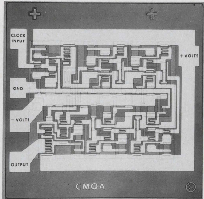
14. Completed quinary scaler is shown in this photomicrograph of the 50-by-50 mil chip.
