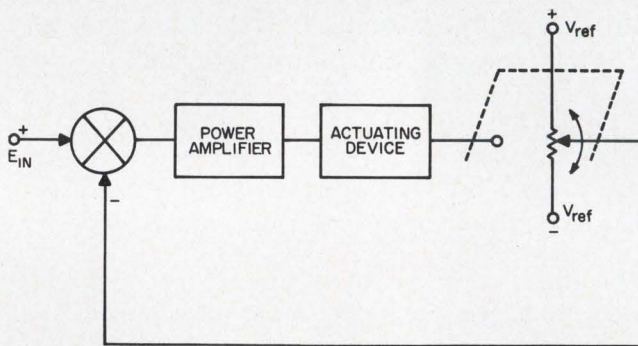
1. The feedback potentiometer in this conventional control system needs two reference voltage sources. Both sources must be precisely balanced.
