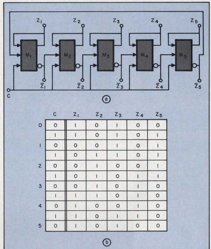
4. Quinary counter has five majority-logic gates (a). On the fifth pulse, outputs return to their initial setting (b).
