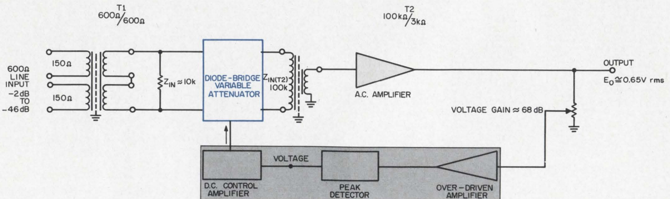
1. Use of diode-bridge attenuator in wide-range agc system compensates for signal changes at summing point.
