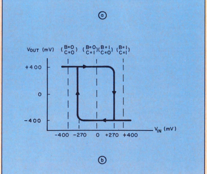
8. Majority-logic circuit is made by slightly modifying the current-mode NOR gate. Note the hysteresis in the transfer characteristic (b).
