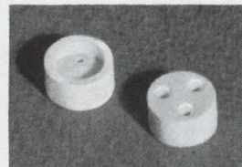
O. D. .372 \pm .002 Counter Bore Diameter .2825 \pm .0025 Holes .064 \pm .0015
