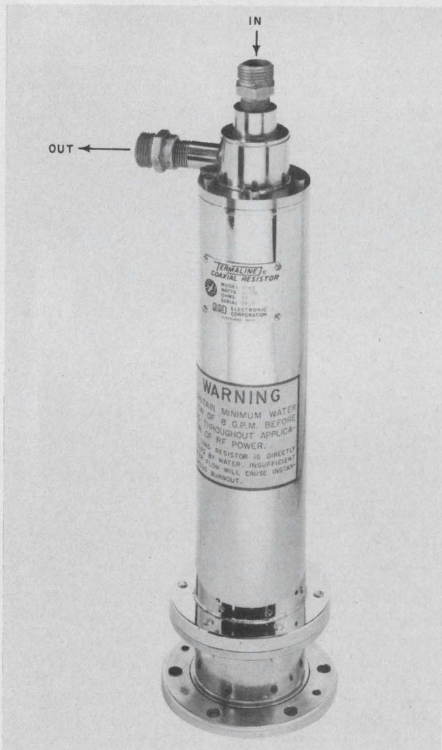
4. The power resistor inside this dummy load (a film deposited on ceramic substrate) is cooled directly with water at a rate of about 8 gallons per minute. This termination (Bird TERMALINE® Model 8762) is rated 50 kW.
