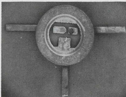
Planar stripline construction as seen without package cover.
