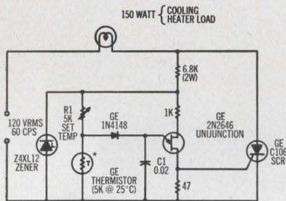
*REVERSE THERMISTOR AND R1 FOR COOLING LOAD NOTE: ALL RESISTORS 1/2 WATT EXCEPT AS NOTED
