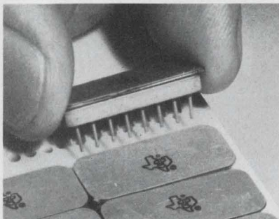
Figure 4. New plug-in flat packages for TI integrated circuits are easily handled and inserted into industrial-type PC boards.
