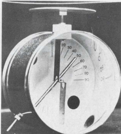
2. $3 electroscope made from a Maxwell House coffee can, by Macalaster, uses an aluminized drinking straw for the pointer.
