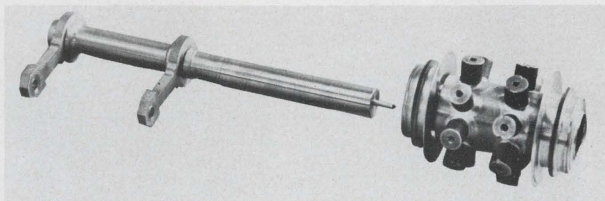
1. Heat pipe (left) and thermionic converter (right) team up to convert thermal energy directly to electricity.
