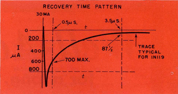
TYPICAL RECOVERY TIME TRACE FOR THE TYPE IN119
