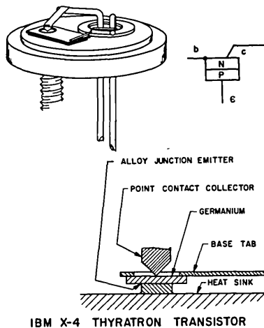
IBM X-4 THYATRON TRANSISTOR
