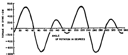
TORQUE CURVE OF APPROXIMATE (110) DISK OF \text{Fe}_3\text{O}_4 AT ROOM TEMPERATURE (SAMPLE VOLUME \approx 0.01 \text{ CC} )
