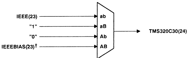
Figure 8. IEEE Bit 23 to TMS320C30 Bit 24
