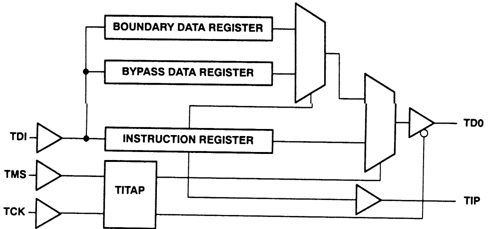
Figure 21. Scan Architecture
