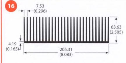
82160 9.0 lb/ft 0.48°C/W/3in Per.=145.02
