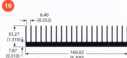
81480 3.7 lb/ft 1.30 °C/W/3in Per.=53.99
