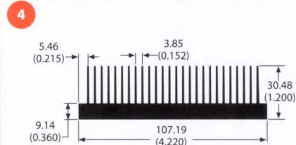
80350 2.9 lb/ft 1.35 °C/W/3in Per.=51.91
