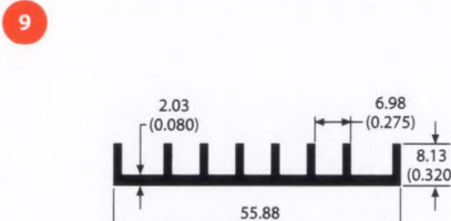
66730 0.3 lb/ft 8.38 °C/W/3in Per.=8.34
