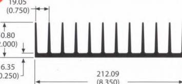
class A 60815 5.7 lb/ft 1.22 °C/W/3in Per.=57.10
