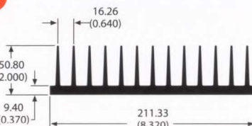
70400 6.9 lb/ft 1.22 °C/W/3in Per.=57.26
