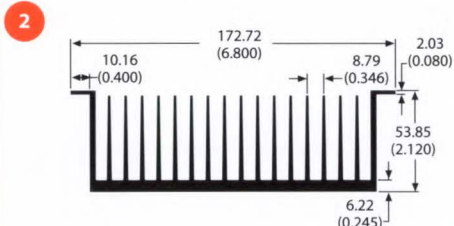
77555 4.8 lb/ft 0.91 °C/W/3in Per.=77.08
