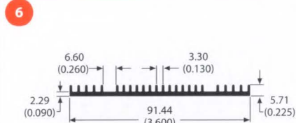
72785 0.8 lb/ft 5.18 °C/W/3in Per.=13.50
