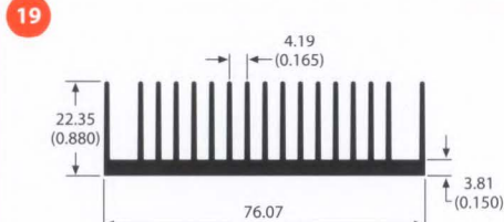
74415 1.2 lb/ft 2.29 °C/W/3in Per.=30.47
