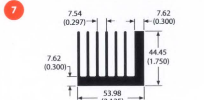
class A 63135 2.1 lb/ft 2.82 °C/W/3in Per.=24.78
