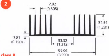
class A 60630 1.7 lb/ft 2.29 °C/W/3in Per.=30.49
