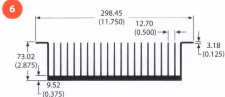
69200 10.2 lb/ft 0.56 °C/W/3in Per.=125.57
