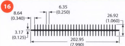
60410 2.7 lb/ft 1.51 °C/W/3in Per.=46.20
