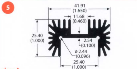
class A 63485 0.8 lb/ft 5.56 °C/W/3in Per.=12.57
