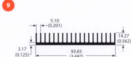
class A 64870 1.0 lb/ft 2.49 °C/W/3in Per.=28.09
