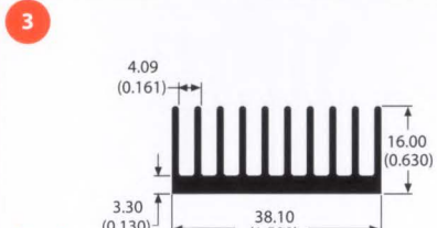
class A 66365 0.5 lb/ft 5.41 °C/W/3in Per.=12.93
