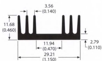
62365 0.3 lb/ft 11.01 °C/W/3in Per.=6.35
