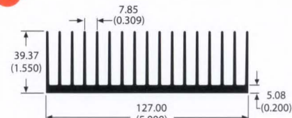
80640 3.0 lb/ft 1.27 °C/W/3in Per.=55.04
