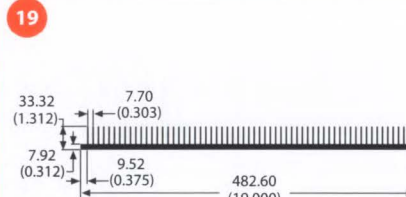
class A 62335 12.9 lb/ft 0.44 °C/W/3in Per.=157.72
