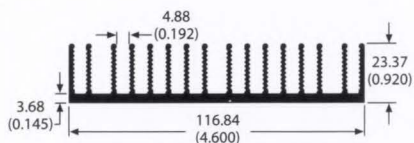
69945 1.8 lb/ft 1.78 °C/W/3in Per.=39.24
