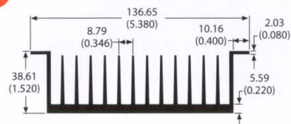
77920 2.8 lb/ft 1.58 °C/W/3in Per.=44.23
