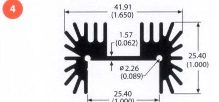
class A 78915 0.7 lb/ft 5.09 °C/W/3in Per.=13.75
