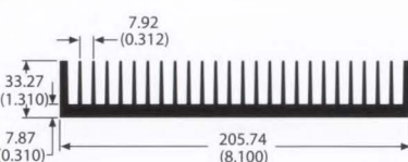
80580 6.5 lb/ft 0.90 °C/W/3in Per.=77.32
