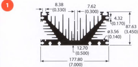
64730 10.9 lb/ft 0.75 °C/W/3in Per.=93.19
