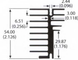
78075 1.1 lb/ft 3.03 °C/W/3in Per.=23.07
