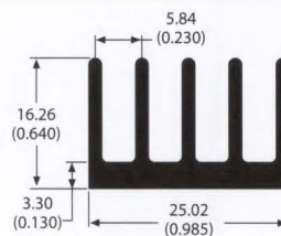
63240 0.3 lb/ft 9.86 °C/W/3in Per.=7.09
