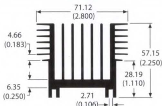
81255 2.4 lb/ft 1.72 °C/W/3in Per.=40.73
