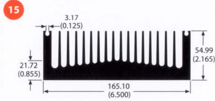
69180 9.1 lb/ft 1.07 °C/W/3in Per.=65.60
