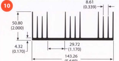
62410 2.8 lb/ft 1.38 °C/W/3in Per.=50.72
