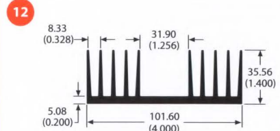
60905 2.2 lb/ft 2.22 °C/W/3in Per.=31.43
