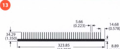
72225 8.8 lb/ft 0.69 °C/W/3in Per.=101.82
