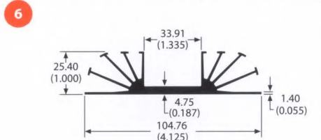
class A 60080 1.2 lb/ft 2.91 °C/W/3in Per.=24.04
