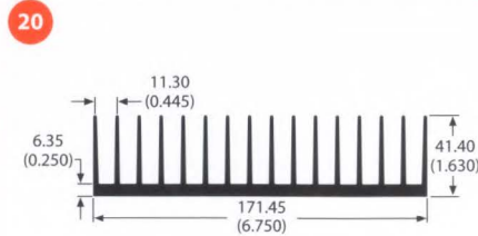
62060 4.3 lb/ft 1.23 °C/W/3in Per.=56.84
