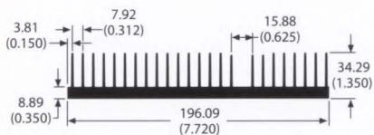
61880 5.1 lb/ft 1.13 °C/W/3in Per.=62.06
