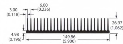
class A 64500 3.3 lb/ft 1.33 °C/W/3in Per.=52.60
