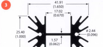
class A 63130 0.6 lb/ft 5.54 °C/W/3in Per.=12.62
