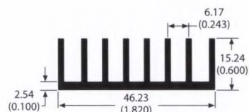
75925 0.5 lb/ft 5.97 °C/W/3in Per.=11.70
