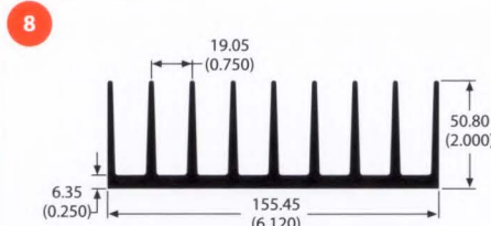
64225 4.3 lb/ft 1.64 °C/W/3in Per.=42.71
