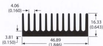
64635 0.7 lb/ft 4.67 °C/W/3in Per.=14.96
