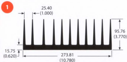
class A 61785 16.2 lb/ft 0.79 °C/W/3in Per.=88.30
