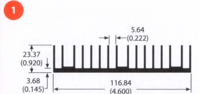
65555 1.7 lb/ft 2.08 °C/W/3in Per.=33.55
