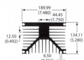
73110 18.99 lb/ft 0.50 °C/W/3in Per.=129.00
