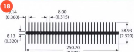
76960 2.9 lb/ft 1.24 °C/W/3in Per.=56.58
