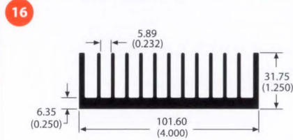
76620 2.5 lb/ft 2.06 °C/W/3in Per.=33.87
