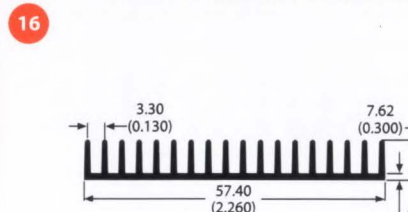
80615 0.4 lb/ft 5.34 °C/W/3in Per.=13.11
