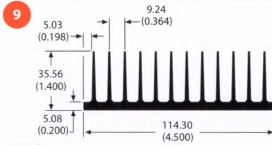
class A 61075 2.3 lb/ft 1.90 °C/W/3in Per.=36.83
