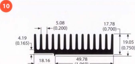
70945 1.2 lb/ft 3.59 °C/W/3in Per.=19.45
