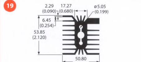
61960 2.2 lb/ft 2.00 °C/W/3in Per.=34.89
