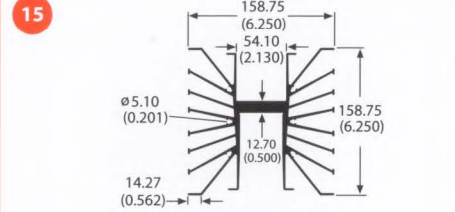
60265 7.7 lb/ft 0.67 °C/W/3in Per.=104.01
