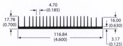
77370 1.3 lb/ft 1.96 °C/W/3in Per.=35.73
