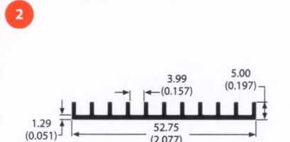
74815 0.2 lb/ft 9.61 °C/W/3in Per.=7.27
