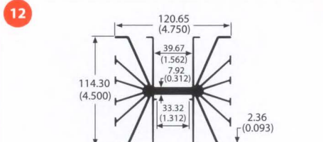
60060 4.0 lb/ft 0.98 °C/W/3in Per.=71.03
