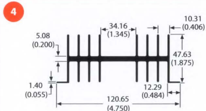
60065 2.2 lb/ft 1.98 °C/W/3in Per.=35.39
