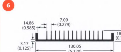
78950 2.7 lb/ft 1.76 °C/W/3in Per.=39.78
