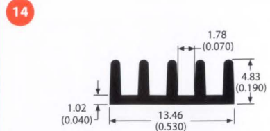
class A 61945 0.1 lb/ft 27.86 °C/W/3in Per.=2.51
