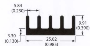
65715 0.3 lb/ft 15.23 °C/W/3in Per.=4.59
