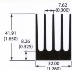
class A 65245 1.1 lb/ft 4.43 °C/W/3in Per.=15.79
