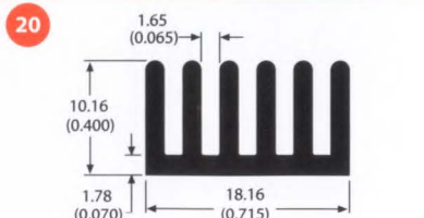
63840 0.3 lb/ft 12.14 °C/W/3in Per.=5.76
