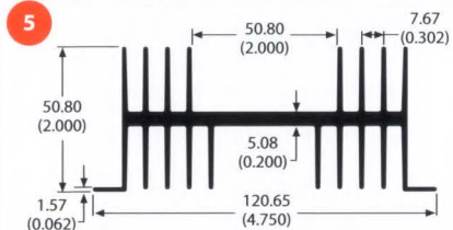
79075 2.3 lb/ft 1.73 °C/W/3in Per.=40.53
