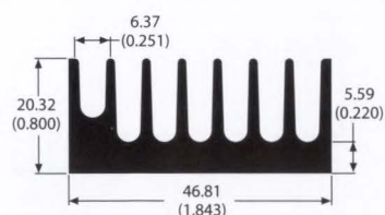
64660 0.9 lb/ft 5.73 °C/W/3in Per.=12.21
