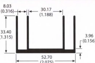
62355 0.7 lb/ft 5.10 °C/W/3in Per.=13.71
