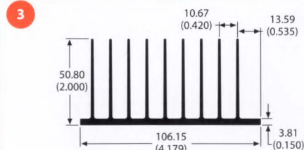
72145 2.1 lb/ft 1.70 °C/W/3in Per.=41.05
