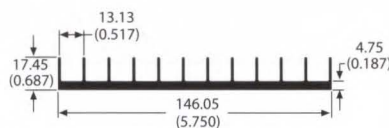
class A 61790 1.7 lb/ft 3.00 °C/W/3in Per.=23.28
