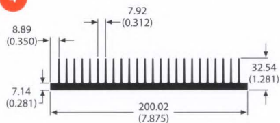
63745 4.6 lb/ft 1.13 °C/W/3in Per.=61.98
