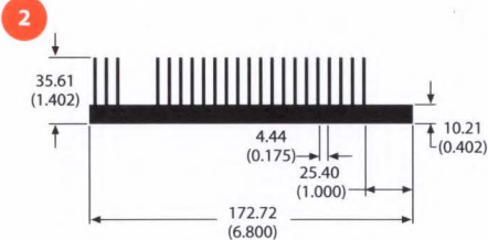
79455 4.8 lb/ft 1.21 °C/W/3in Per.=57.91
