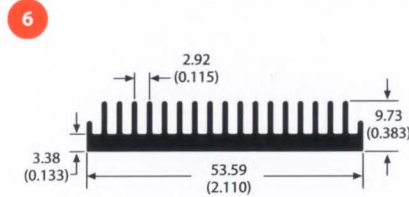
82755 0.5 lb/ft 5.42 °C/W/3in Per.=12.90
