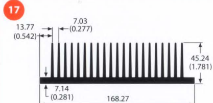
69800 5.9 lb/ft 0.94 °C/W/3in Per.=74.58
