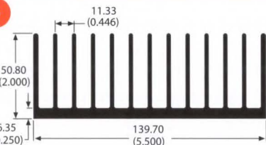
64315 4.3 lb/ft 1.25 °C/W/3in Per.=56.10
