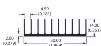
82715 0.4 lb/ft 5.28 °C/W/3in Per.=13.24
