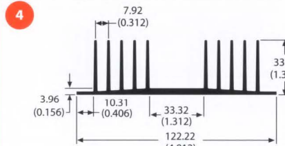
60840 1.8 lb/ft 2.12 °C/W/3in Per.=32.97
