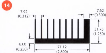
class A 61895 1.7 lb/ft 2.94 °C/W/3in Per.=23.82
