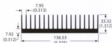
class A 61085 3.4 lb/ft 1.52 °C/W/3in Per.=46.12
