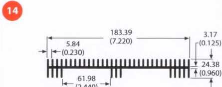
66340 2.8 lb/ft 1.47 °C/W/3in Per.=47.63
