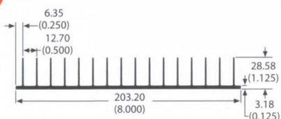
71235 2.2 lb/ft 1.48 °C/W/3in Per.=47.15
