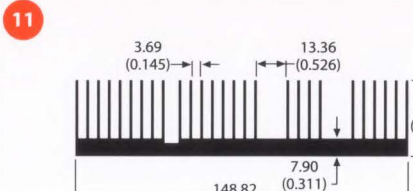
81880 3.6 lb/ft 1.03 °C/W/3in Per.=67.99
