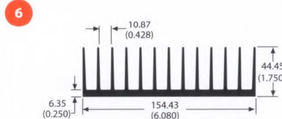
class A 60140 4.0 lb/ft 1.39 °C/W/3in Per.=50.26
