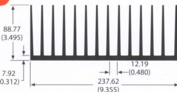
77335 11.9 lb/ft 0.66 °C/W/3in Per.=105.92
