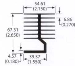
61775 2.0 lb/ft 1.99 °C/W/3in Per.=35.06
