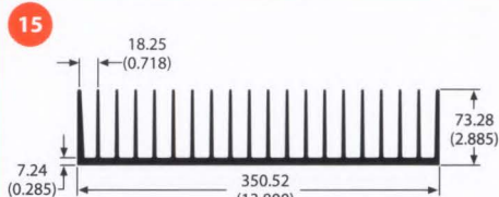
62645 8.3 lb/ft 0.97 °C/W/3in Per.=71.76
