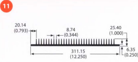
class A 61155 6.8 lb/ft 0.94 °C/W/3in Per.=74.46
