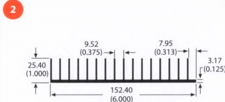
62440 1.9 lb/ft 1.76 °C/W/3in Per.=39.69
