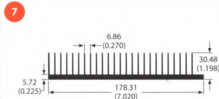
82555 3.4 lb/ft 1.12 °C/W/3in Per.=62.68
