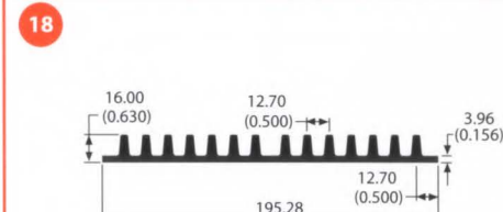
60910 3.0 lb/ft 2.58 °C/W/3in Per.=27.07
