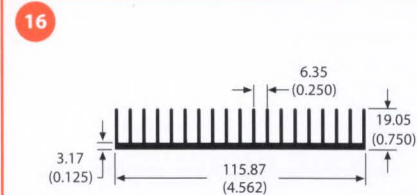
class A 60585 1.5 lb/ft 2.15 °C/W/3in Per.=32.46
