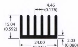
67605 0.3 lb/ft 8.74 °C/W/3in Per.=8.00
