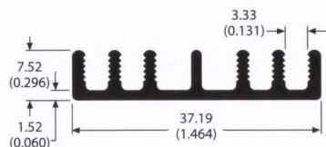
80725 0.2 lb/ft 10.55 °C/W/3in Per.=6.63
