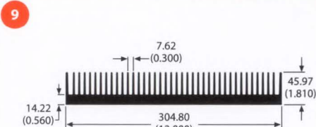
70165 11.8 lb/ft 0.61 °C/W/3in Per.=113.86
