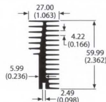
class A 78080 1.1 lb/ft 2.94 °C/W/3in Per.=23.78
