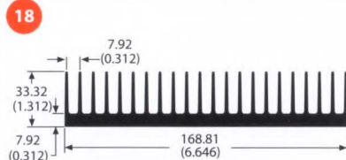
class A 62155 4.6 lb/ft 1.26 °C/W/3in Per.=55.49
