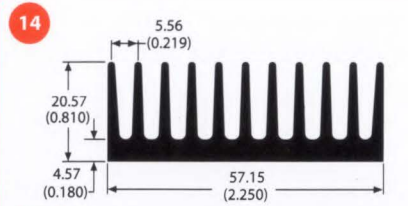
class A 64690 1.1 lb/ft 3.97 °C/W/3in Per.=17.60
