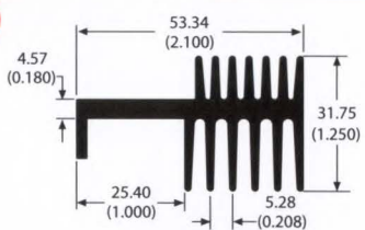
63005 1.1 lb/ft 3.93 °C/W/3in Per.=17.80
