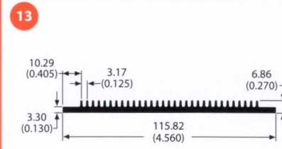
70665 1.0 lb/ft 4.27 °C/W/3in Per.=16.36
