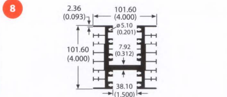
61270 5.1 lb/ft 1.13 °C/W/3in Per.=61.84
