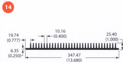
62645 8.3 lb/ft 0.97 °C/W/3in Per.=71.76
