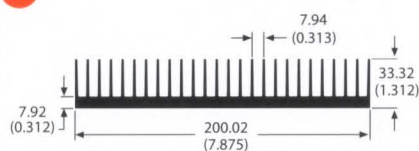
class A 63925 5.1 lb/ft 1.05 °C/W/3in Per.=66.44
