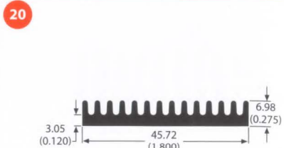
79930 0.4 lb/ft 9.51 °C/W/3in Per.=7.35
