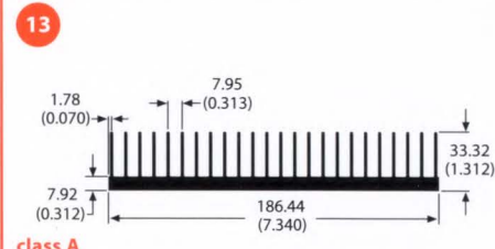
class A 65445 4.6 lb/ft 1.12 °C/W/3in Per.=62.27
