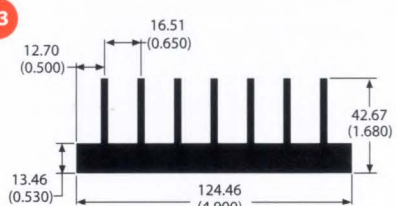
80965 4.2 lb/ft 2.61 °C/W/3in Per.=26.82
