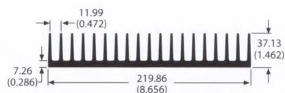
65515 6.2 lb/ft 1.18 °C/W/3in Per.=59.38
