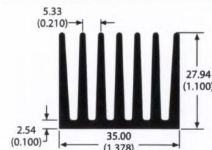
75450 0.9 lb/ft 4.31 °C/W/3in Per.=16.23
