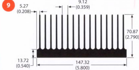
82395 7.5 lb/ft 0.85 °C/W/3in Per.=82.08
