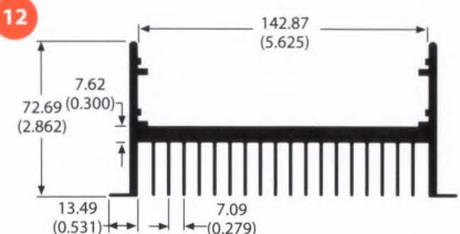
61350 4.4 lb/ft 1.19 °C/W/3in Per.=59.00
