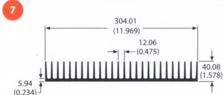
80345 8.3 lb/ft 0.78 °C/W/3in Per.=90.07
