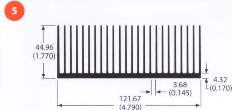
74925 3.4 lb/ft 0.82 °C/W/3in Per.=85.37
