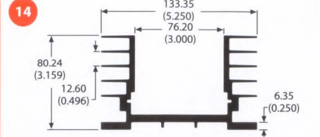
64160 3.8 lb/ft 1.69 °C/W/3in Per.=41.43
