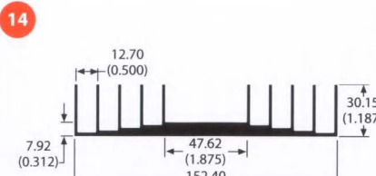
61690 2.6 lb/ft 1.64 °C/W/3in Per.=42.51
