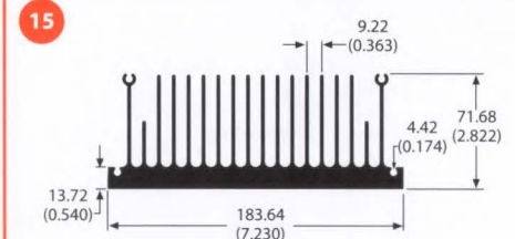
76560 8.7 lb/ft 0.76 °C/W/3in Per.=91.74
