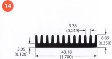
79920 0.5 lb/ft 8.38 °C/W/3in Per.=8.34
