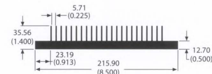
71390 6.8 lb/ft 1.20 °C/W/3in Per.=58.07
