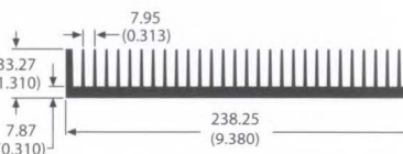
80575 6.5 lb/ft 0.90 °C/W/3in Per.=77.32
