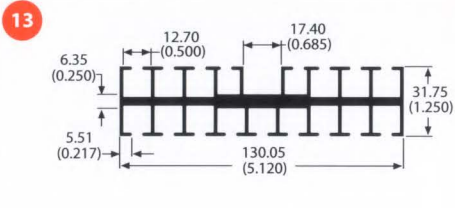
64375 2.2 lb/ft 1.71 °C/W/3in Per.=40.82
