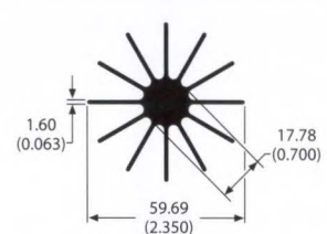
61925 1.2 lb/ft 3.30 °C/W/3in Per.=21.20
