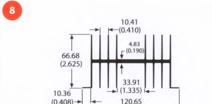
class A 60055 2.2 lb/ft 1.45 °C/W/3in Per.=48.15
