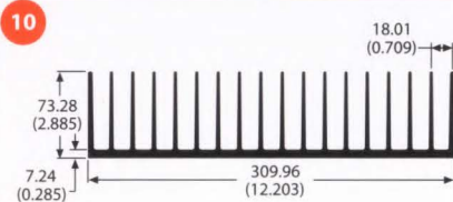
class A 65535 11.3 lb/ft 0.60 °C/W/3in Per.=115.65
