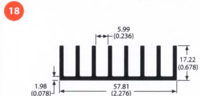
class A 60975 0.7 lb/ft 4.95 °C/W/3in Per.=14.12
