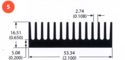
80120 0.9 lb/ft 4.31 °C/W/3in Per.=16.21
