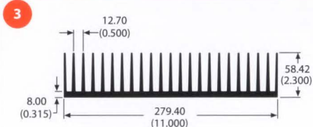
75890 7.4 lb/ft 0.74 °C/W/3in Per.=94.73
