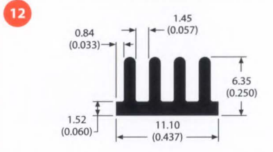
68265 0.1 lb/ft 29.13 °C/W/3in Per.=2.40
