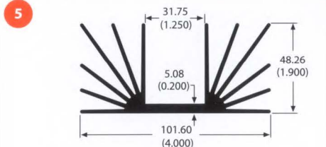
62720 2.2 lb/ft 1.88 °C/W/3in Per.=37.10
