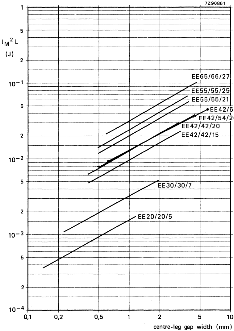
Choke core selection chart for EE cores.
