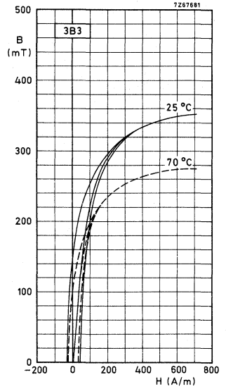
ballistic curves
