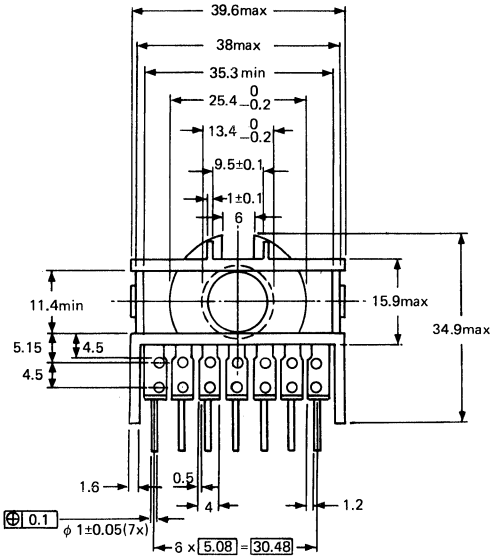
Pin arrangement
