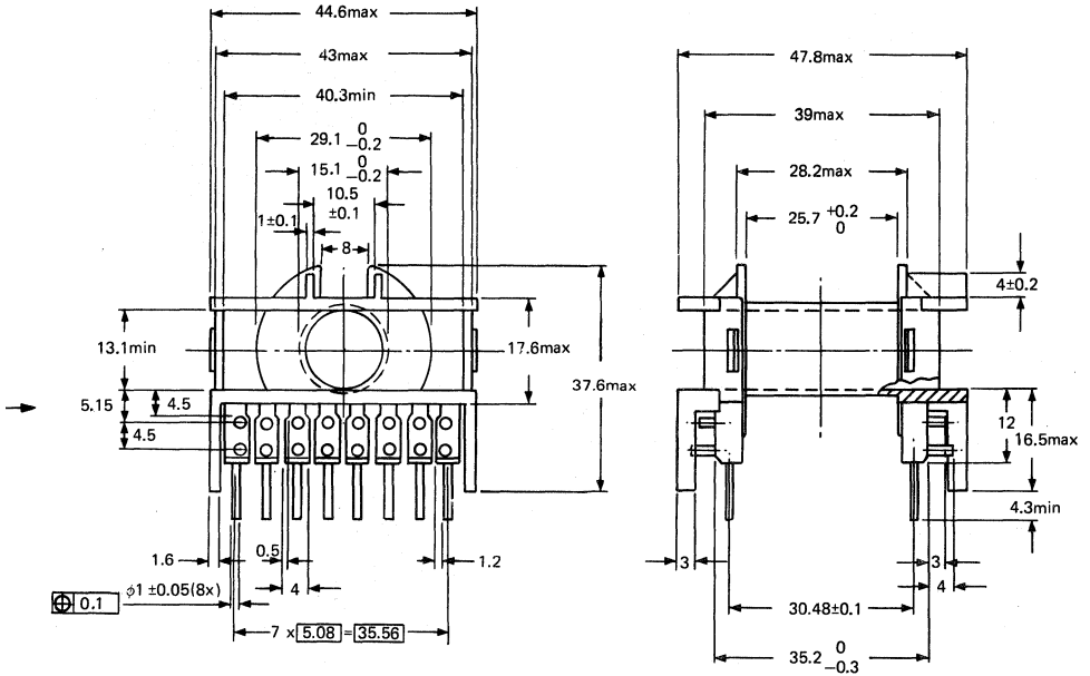
Pin arrangement
