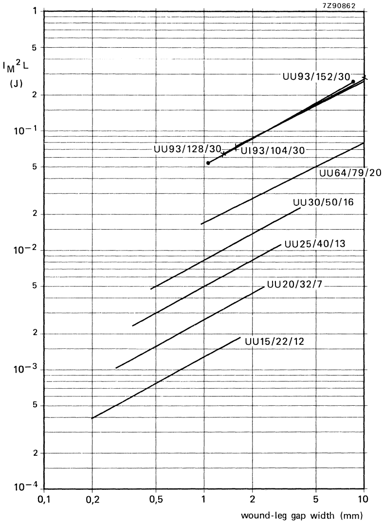
Choke core selection chart for UU/UI cores.
