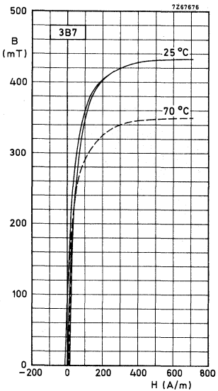
ballistic curves
