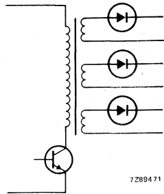
Fig. 4 Multiple output flyback converter circuit.
