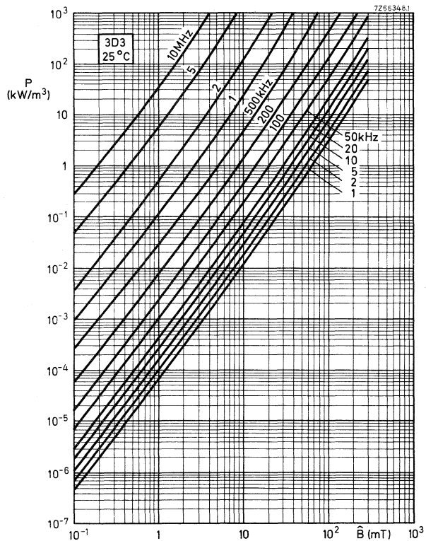
Power loss as a function of the induction
