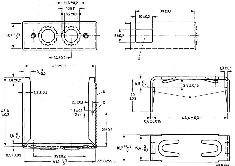
Clasp 4322 021 31910 Material: chromium nickel steel.
