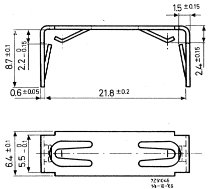
(2). Spring 4322 021 20220. Material: phosphor-bronze, tin-plated.
