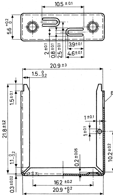
(1). Clasp 4322 021 20160. Material: brass, tin-plated.
