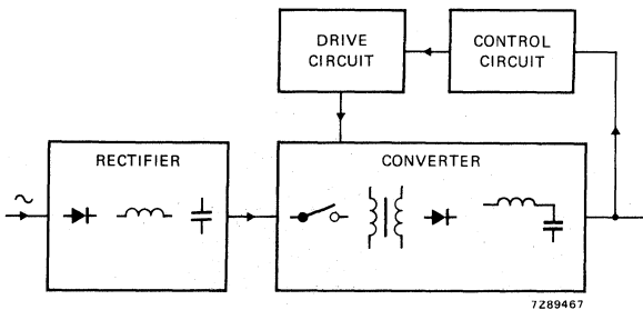
Fig. 1 Block diagram of switched-mode power supply.
