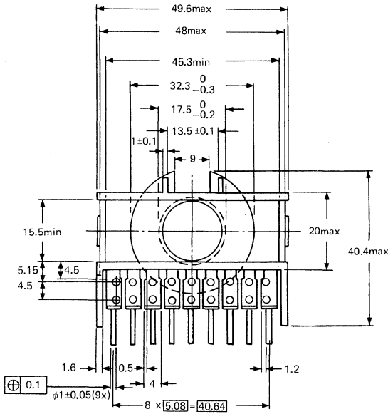
Pin arrangement
