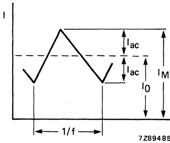
Fig. 14 Choke waveform showing symbols for currents are full load.
