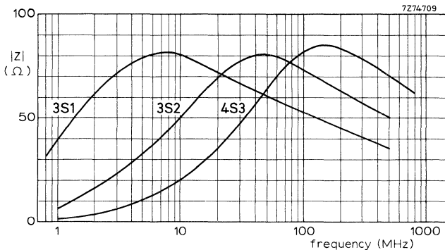
Fig. 1 Impedance of Ferroxcube grades as a function of frequency. The curves are typical for a bead size of 5 \times 2 \times 10 mm.
