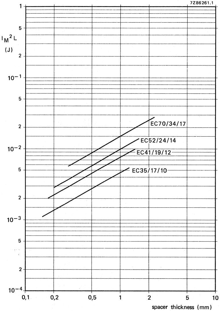
Choke core selection chart for EC cores.
