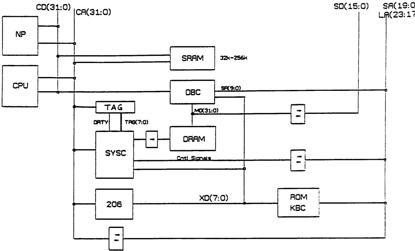
BLOCK DIAGRAM
