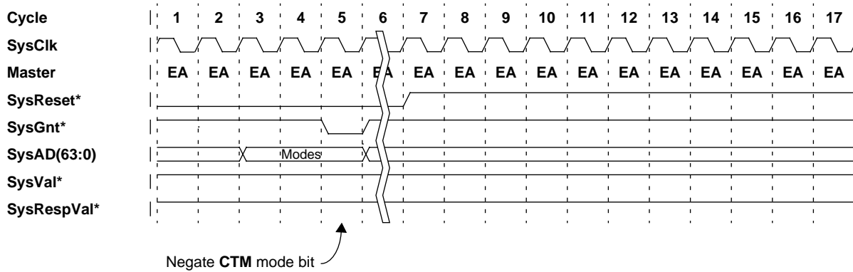
Figure 17-2 Cache Test Mode Exit Sequence
