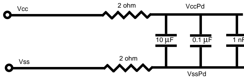
Figure 11-2 Decoupling VccPd and VssPd
