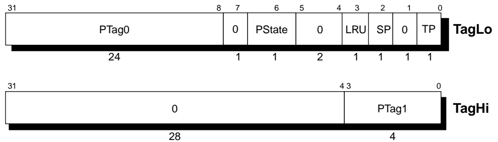
Figure 13-28 TagHi/Lo Register Fields in Primary Instruction Cache When CacheOp is Index Load/Store Tag
