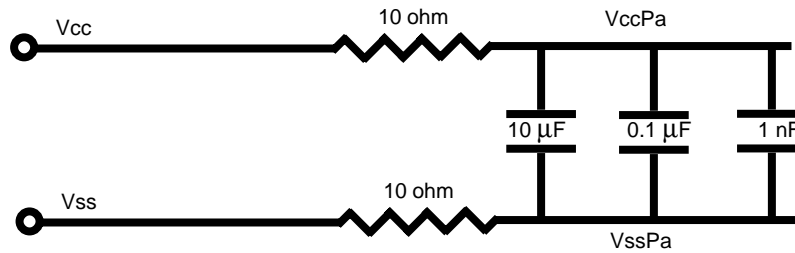
Figure 11-1 Decoupling VccPa and VssPa
