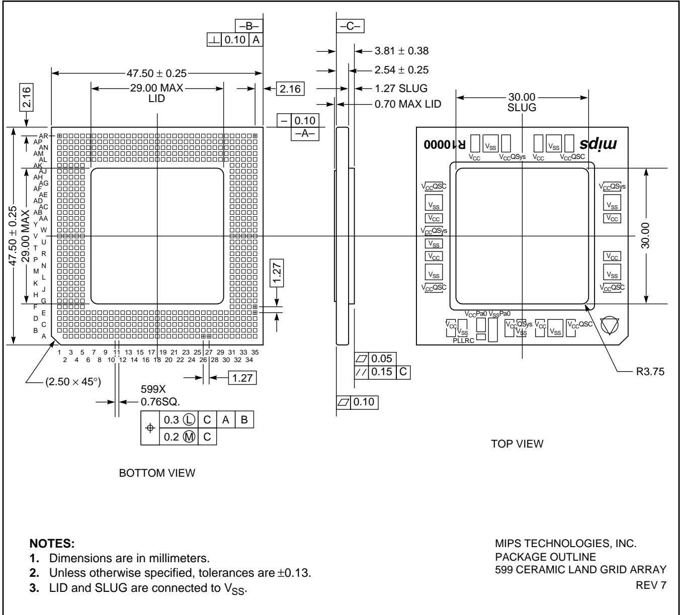
Figure 12-1 R10000 599CLGA Package Outline
