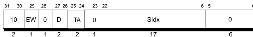
Figure 13-26 CacheErr Register Format for Secondary Cache Errors
