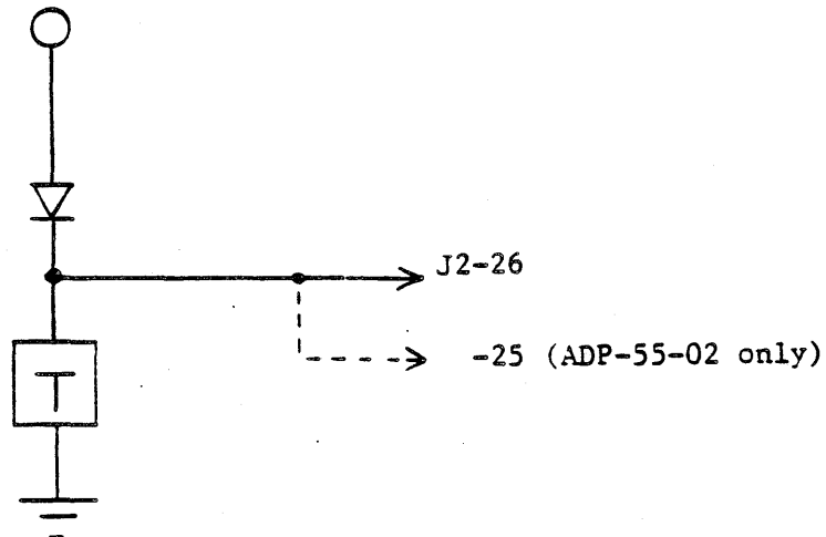
SCSI BUS TERMINATION
