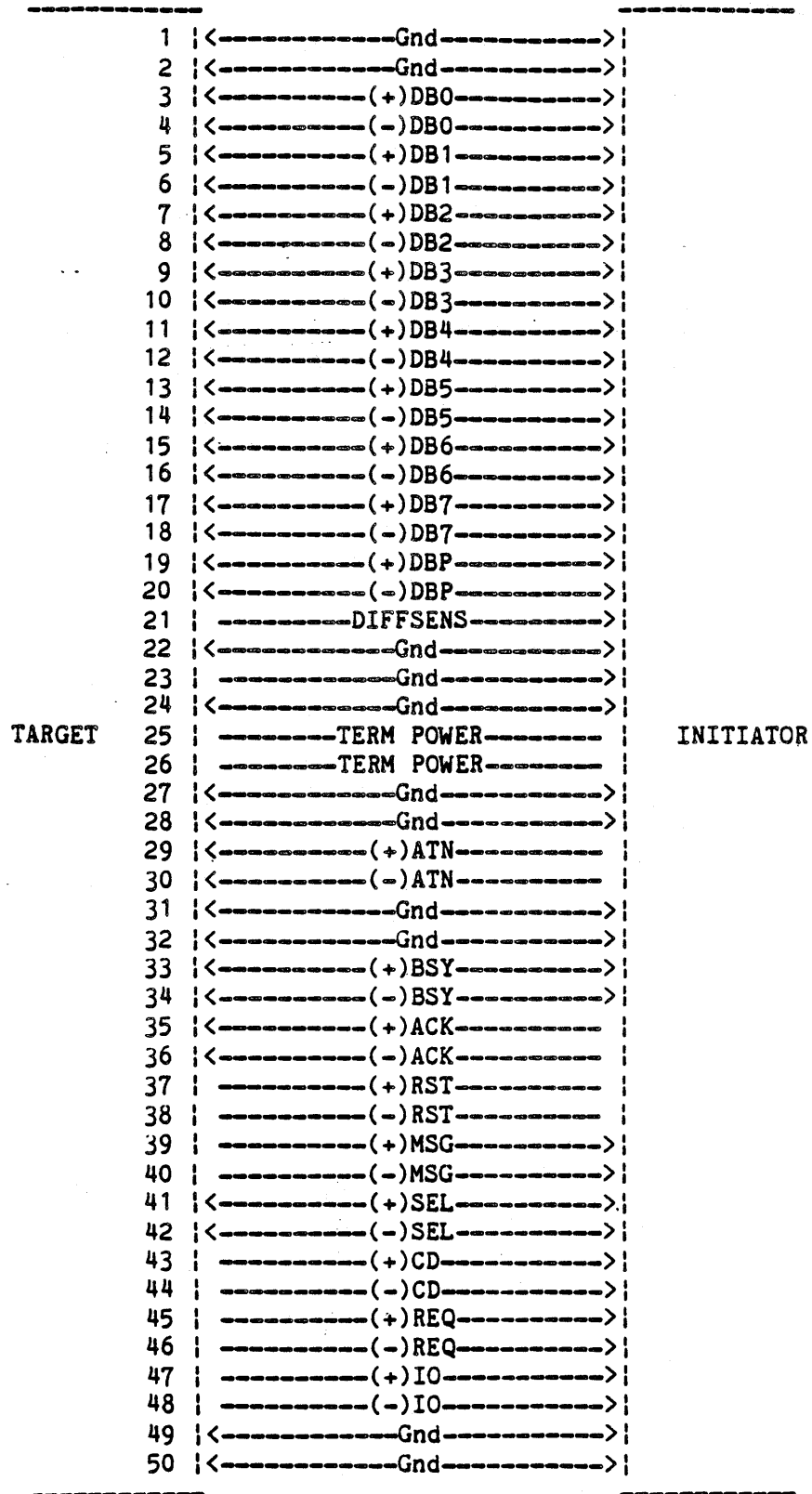
Figure 2. Differential pin assignments
