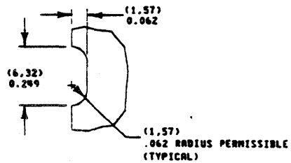
DETAIL B (2 PLACES) DETAIL C ROTATED 180° (2 PLACES) (NO SCALE)
