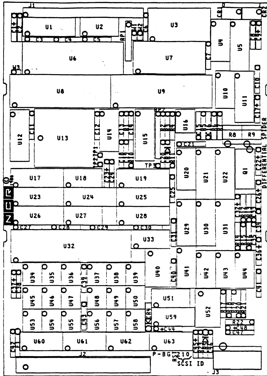
Figure 8. Component locations on differential version
