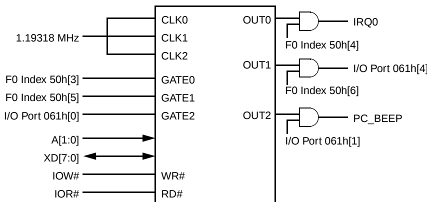
Figure 4-14. PIT Timer
