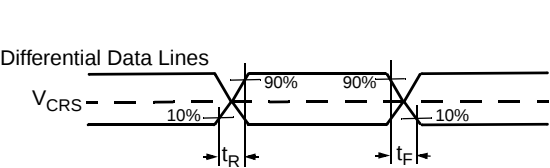
Figure 6-9. USB Timing
