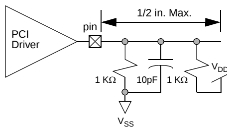
Figure 6-5. PCI Slew Rate Test Circuit
