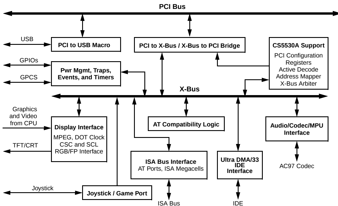
Figure 1-1. Block Diagram
