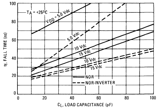
FIGURE 15 – TYPICAL FALL TIME versus LOAD CAPACITANCE
