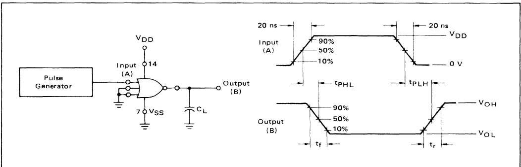
FIGURE 9 – SWITCHING TIME TEST CIRCUIT AND WAVEFORMS
