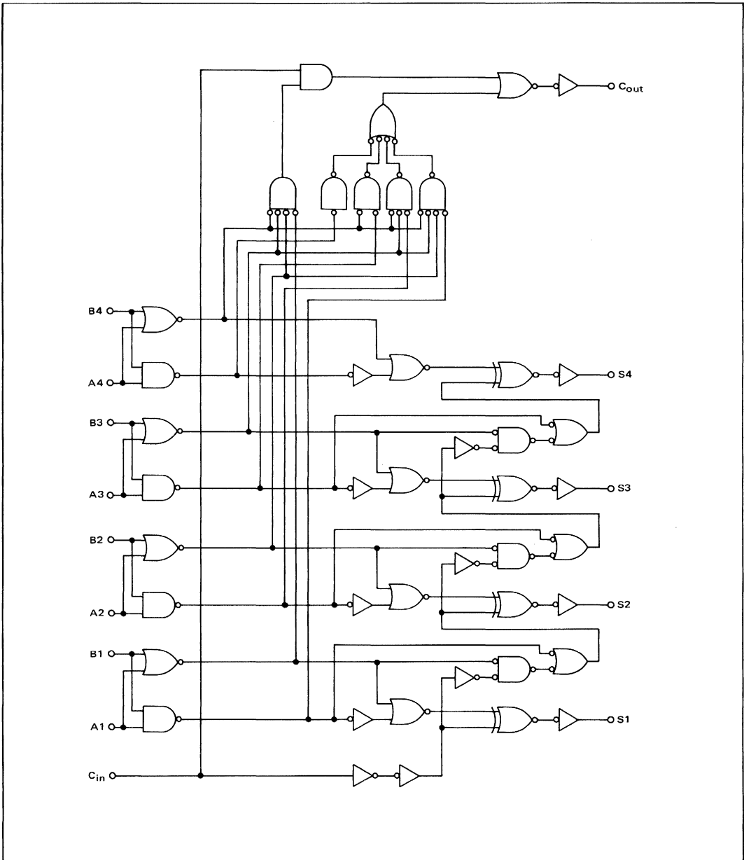
FIGURE 6 - LOGIC DIAGRAM
