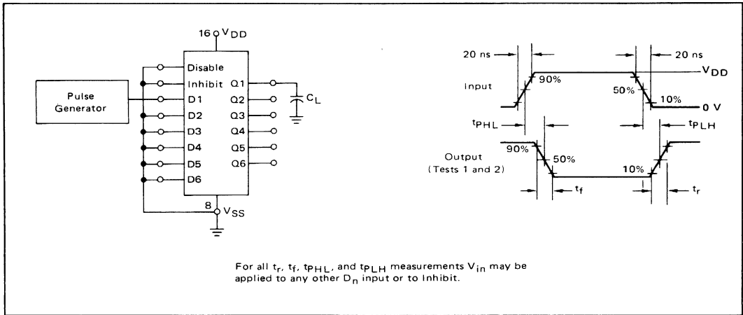
FIGURE 8 – AC TEST CIRCUIT AND WAVEFORMS ( t_r , t_f , t_{PHL} , and t_{PLH} )
