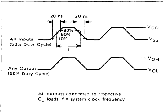
FIGURE 1 – DYNAMIC POWER DISSIPATION SIGNAL WAVEFORMS
