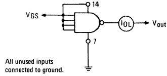
FIGURE 2 – TYPICAL OUTPUT SINK CHARACTERISTICS TEST CIRCUIT
