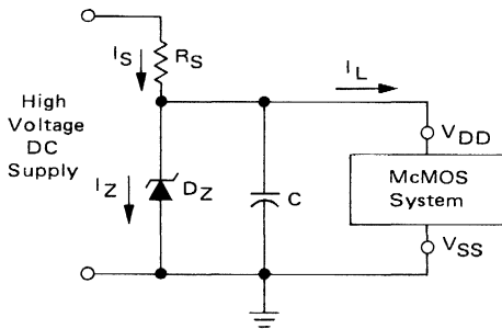
FIGURE 2-9 — DERIVING CMOS POWER FROM HIGH VOLTAGE DC SOURCE
