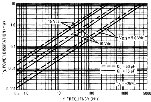
FIGURE 6 - POWER DISSIPATION CHARACTERISTICS
