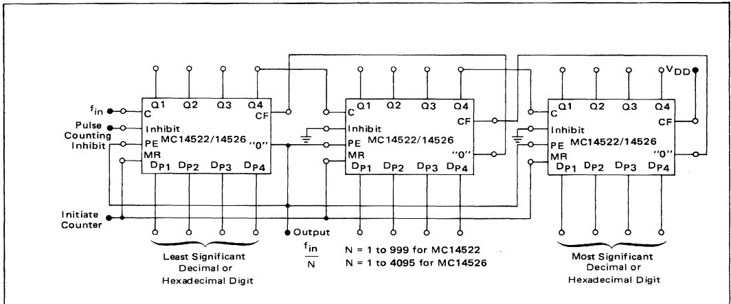
FIGURE 10 – 3-STAGE PROGRAMMABLE FREQUENCY DIVIDER
