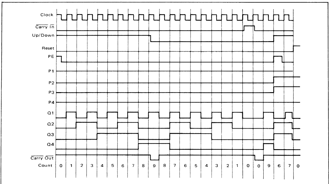
TIMING DIAGRAM
