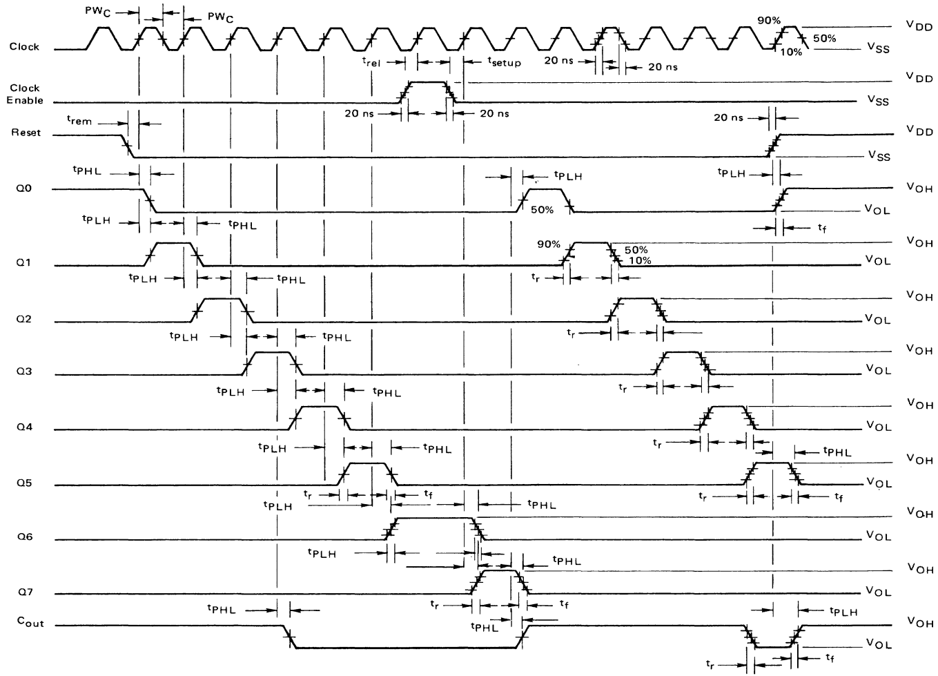
FIGURE 3 — AC MEASUREMENT DEFINITION AND FUNCTIONAL WAVEFORMS
