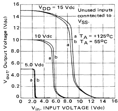
FIGURE 5-8 – VOLTAGE TRANSFER CHARACTERISTICS versus TEMPERATURE
