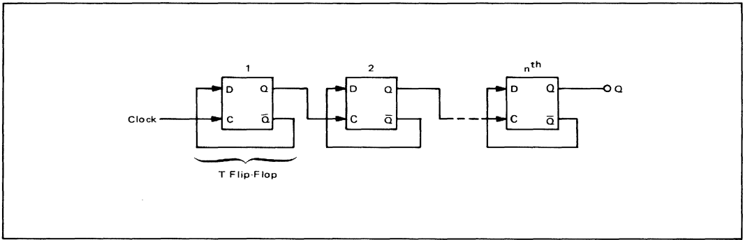
BINARY RIPPLE UP-COUNTER (Divide-by- 2^n )
