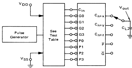
FIGURE 3 – SWITCHING TIME TEST CIRCUIT AND WAVEFORMS
