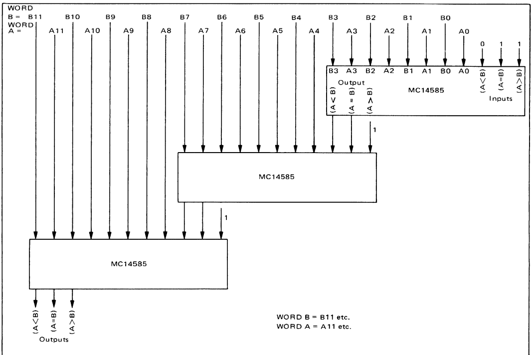
FIGURE 3 – CASCADING COMPARATORS
