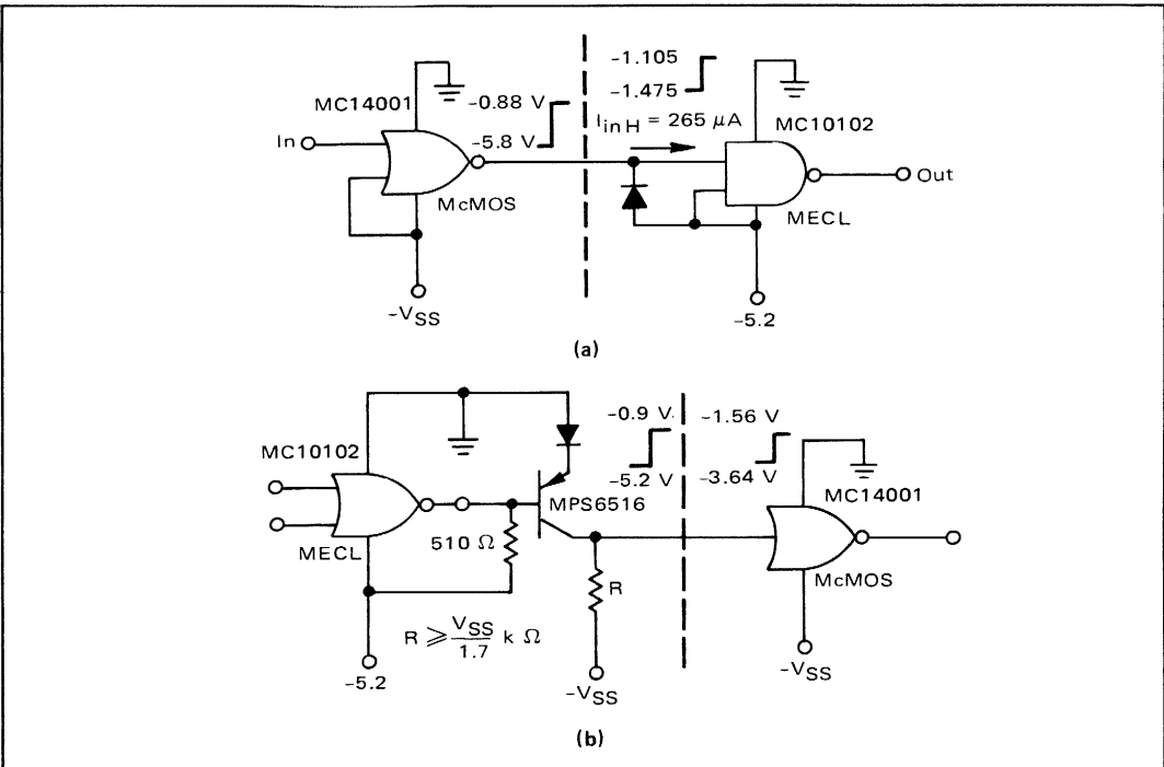
FIGURE 2-24—McMOS—MECL AND MECL—McMOS INTERFACE SYSTEMS
