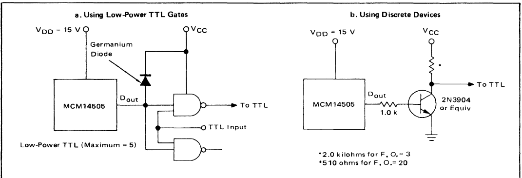
FIGURE 14 – CMOS-TO-TTL INTERFACE FOR V_{DD} = 15\text{ V}
