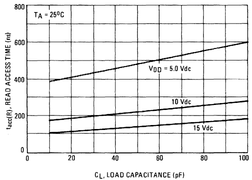
FIGURE 4 – TYPICAL READ ACCESS TIME versus LOAD CAPACITANCE
