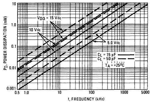
FIGURE 2 – POWER DISSIPATION CHARACTERISTICS
