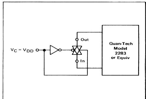
FIGURE 15 – NOISE VOLTAGE TEST CIRCUIT
