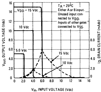
FIGURE 4 – TYPICAL VOLTAGE AND CURRENT TRANSFER CHARACTERISTICS
