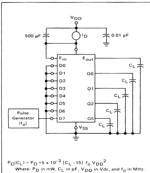
FIGURE 2 – TYPICAL POWER DISSIPATION TEST CIRCUIT
