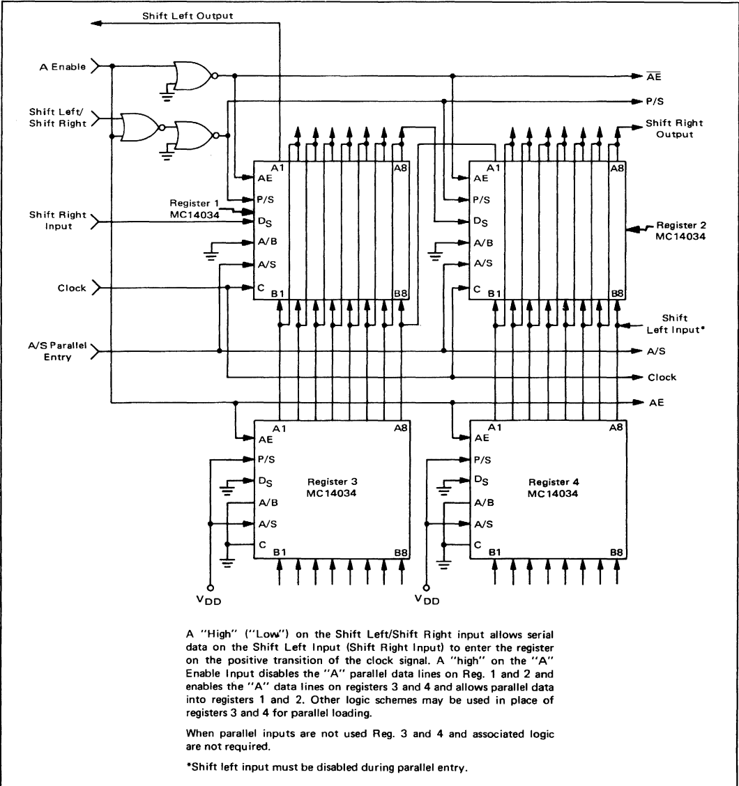
FIGURE 7 – SHIFT RIGHT/SHIFT LEFT WITH PARALLEL INPUTS
