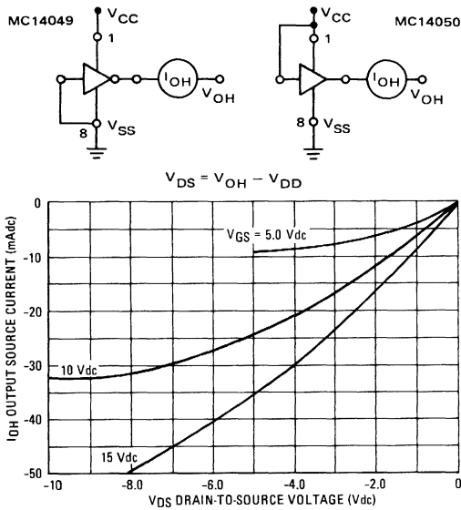
FIGURE 3 – TYPICAL OUTPUT SOURCE CHARACTERISTICS
