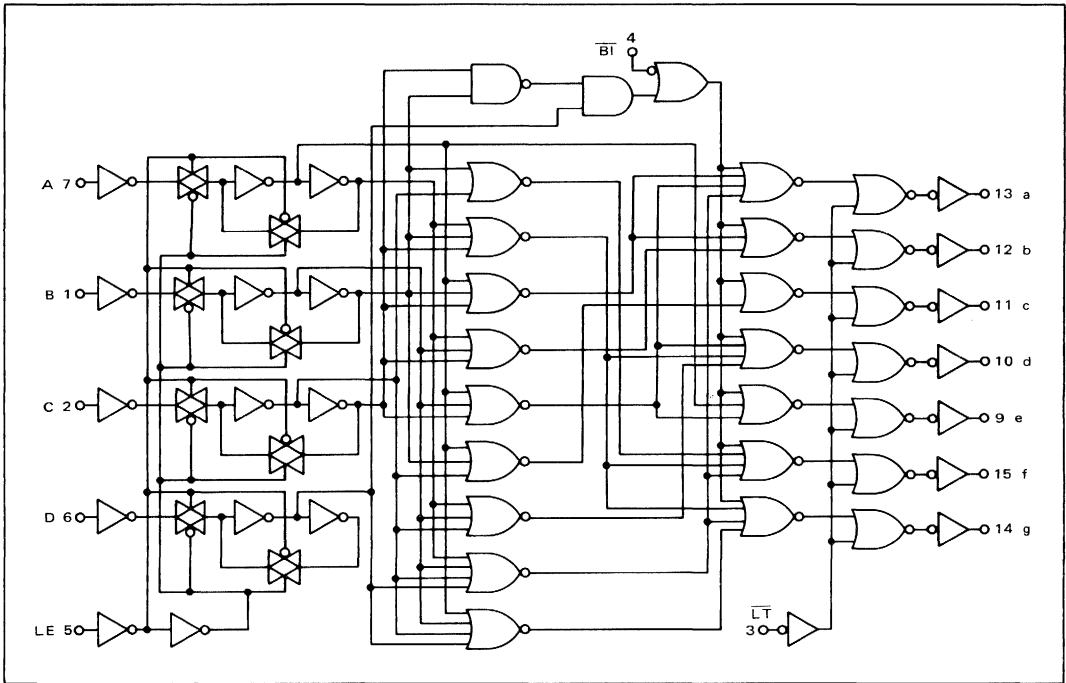
LOGIC DIAGRAM
