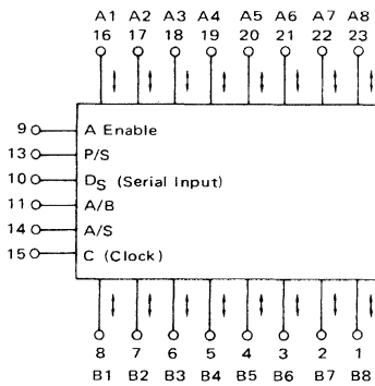
MC14034 8-Bit Universal Bus Register
