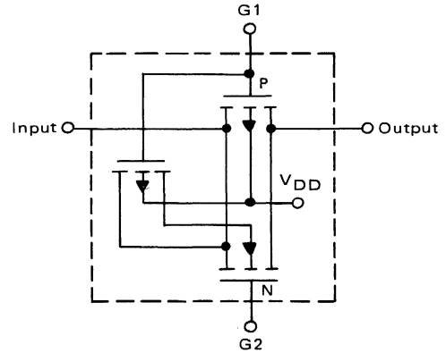
FIGURE 2-38 – MODIFIED McMOS TRANSMISSION GATE
