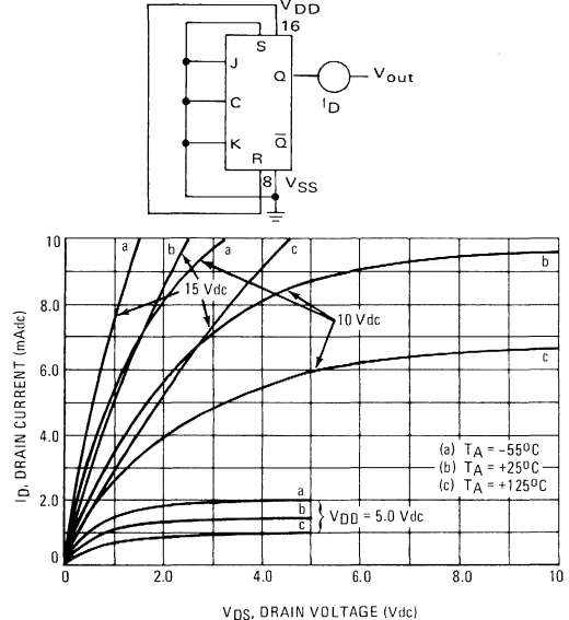
FIGURE 5 – TYPICAL OUTPUT SINK CHARACTERISTICS
