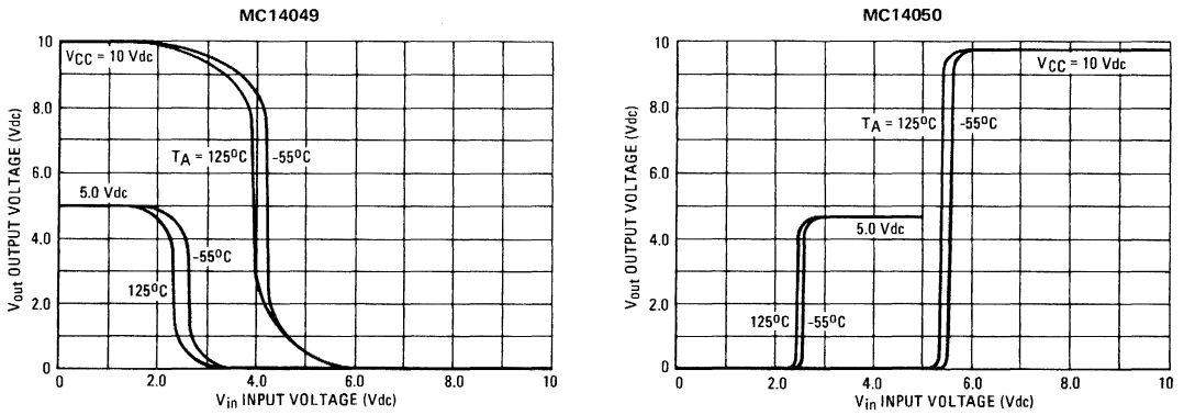
FIGURE 2 – TYPICAL VOLTAGE TRANSFER CHARACTERISTICS versus TEMPERATURE
