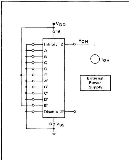
FIGURE 2 – TYPICAL OUTPUT SOURCE CHARACTERISTICS TEST CIRCUIT
