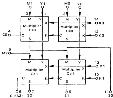
LOGIC DIAGRAM
