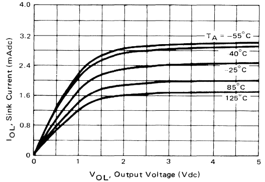
FIGURE 5-4 – V_{GS} = 5.0 \text{ Vdc} , V_{DD} = 5.0 \text{ Vdc}
