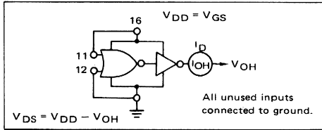
FIGURE 6 – TYPICAL OUTPUT SOURCE CHARACTERISTICS
