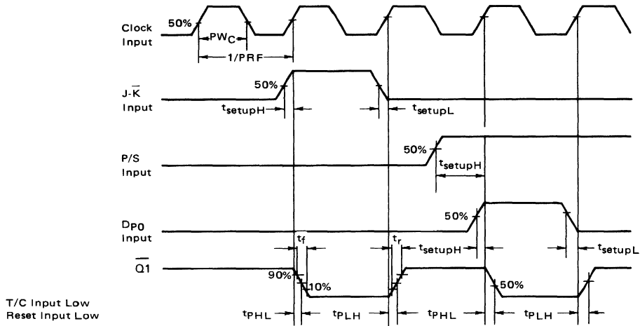
FIGURE 1 – TIMING DIAGRAM
