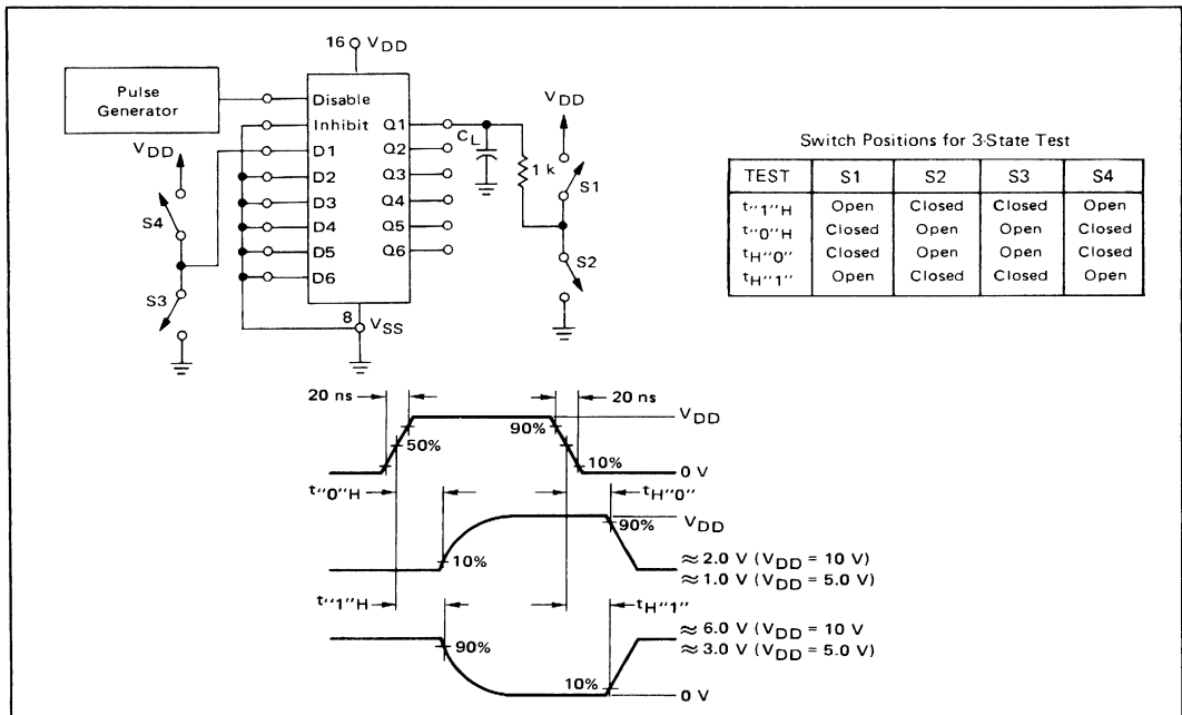
FIGURE 9 – 3-STATE AC TEST CIRCUIT AND WAVEFORMS ( t_{r1}''H , t_{H1}''1 , t_{r0}''H , and t_{H0}''0 )
