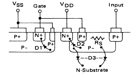
FIGURE 2-14(a) – PHYSICAL DIAGRAM, DIODE-RESISTOR INPUT PROTECTION METHOD
