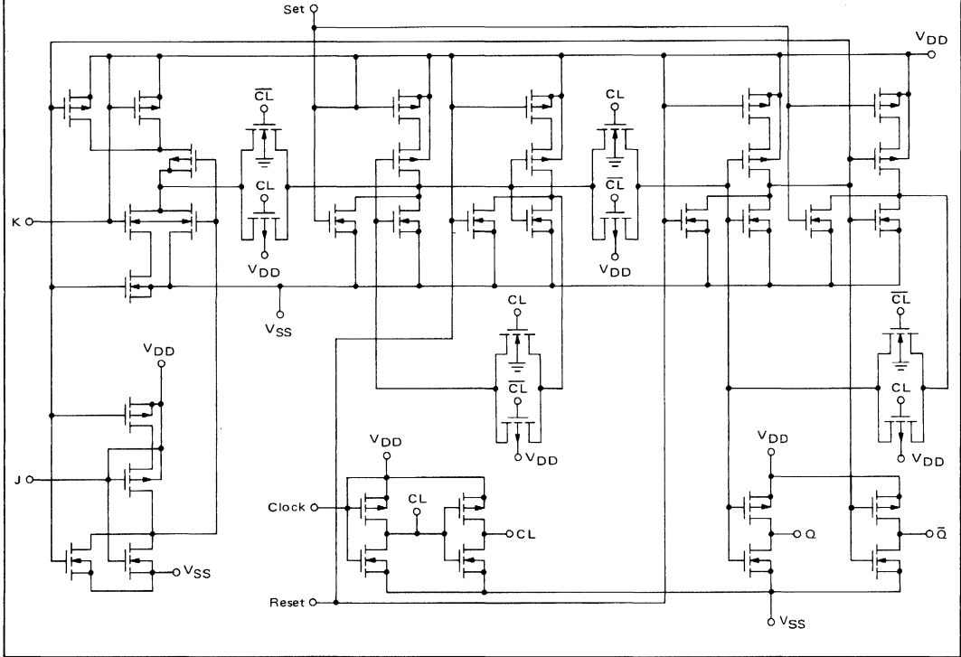
LOGIC DIAGRAM (1/2 OF CIRCUIT SHOWN)
