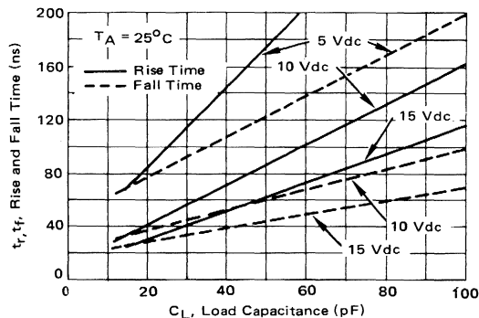
FIGURE 5-10 – RISE AND FALL TIME versus LOAD CAPACITANCE
