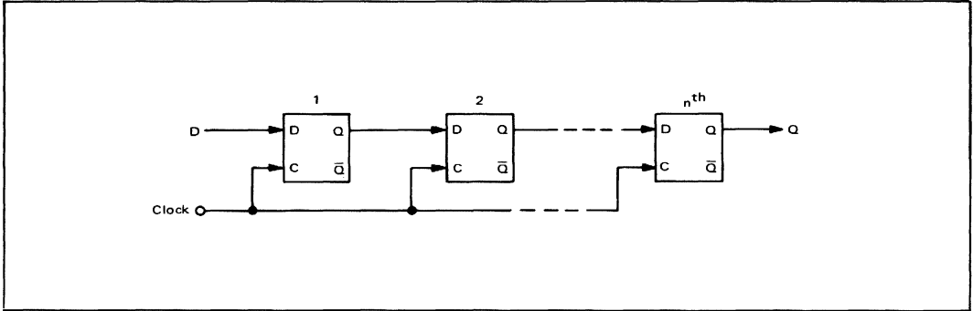
n-STAGE SHIFT REGISTER
