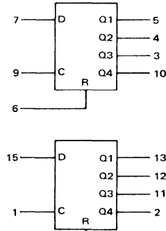
MC14015 Dual 4-Bit Static Shift Register
