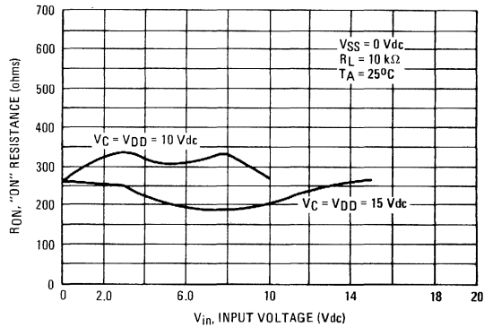
FIGURE 7 – V_{SS} = 0 V
