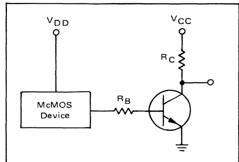
FIGURE 2-28 – CMOS TO DISCRETE INTERFACE
