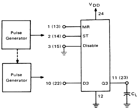
TEST CONNECTIONS
