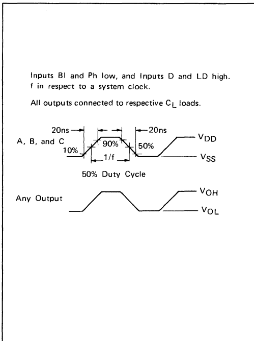
FIGURE 3 – DYNAMIC POWER DISIPATION SIGNAL WAVEFORMS
