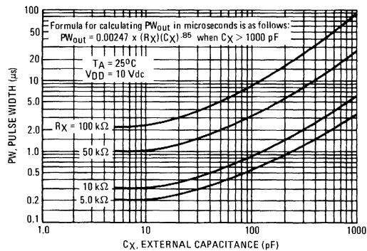
FIGURE 8 - C_X versus PULSE WIDTH @ V_{DD} = 10 \text{ V}
