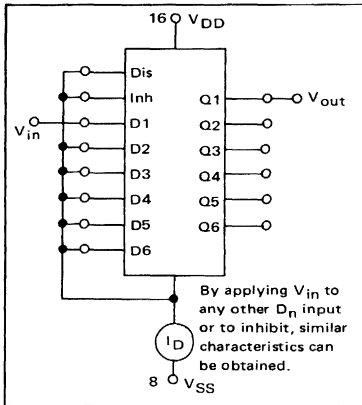
FIGURE 4 – TYPICAL OUTPUT SOURCE CHARACTERISTICS
