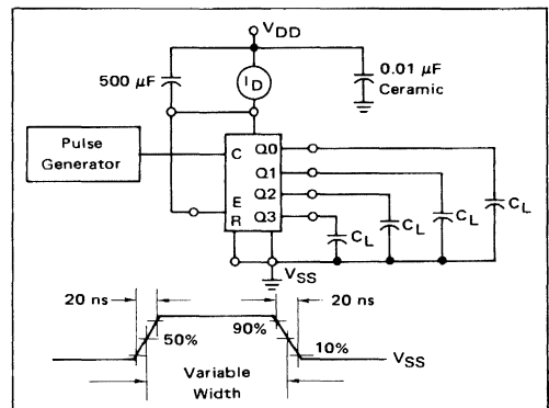
FIGURE 4 – POWER DISSIPATION TEST CIRCUIT AND WAVEFORM
