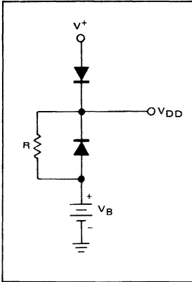
FIGURE 10 – STAND BY BATTERY CIRCUIT
