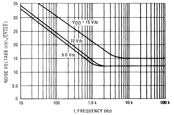
FIGURE 11 – TYPICAL NOISE CHARACTERISTICS
