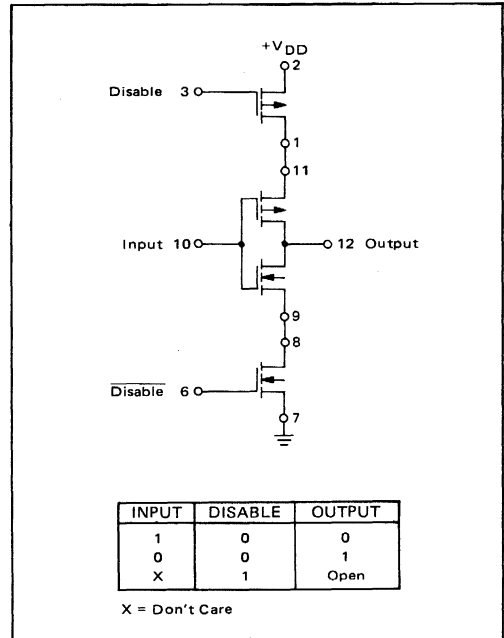
FIGURE 6 – 3-STATE BUFFER
