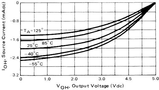
FIGURE 5-1 – V_{GS} = -5.0 \text{ Vdc} , V_{DD} = 5.0 \text{ Vdc}
