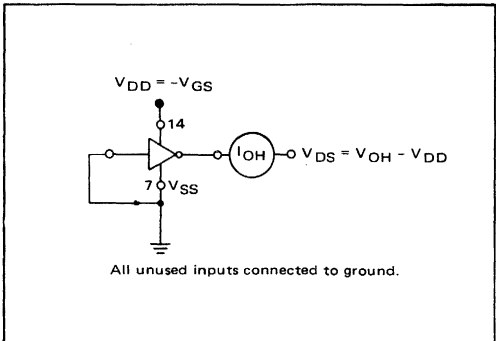
FIGURE 2 – TYPICAL OUTPUT SOURCE CHARACTERISTICS
