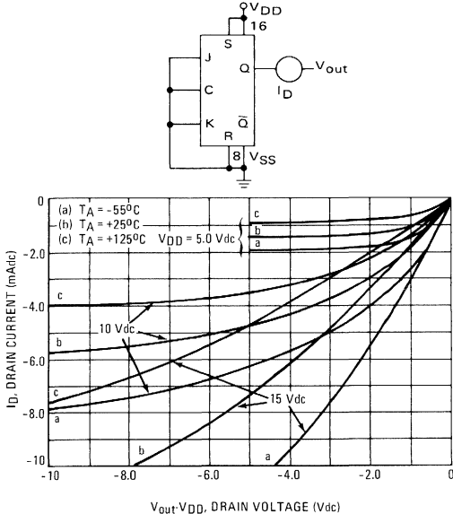
FIGURE 4 – TYPICAL OUTPUT SOURCE CHARACTERISTICS
