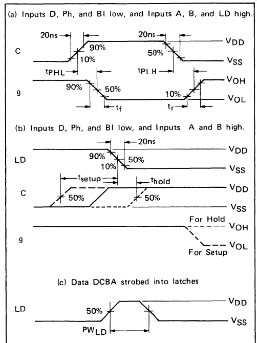
FIGURE 4 – DYNAMIC SIGNAL WAVEFORMS
