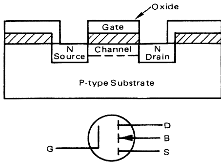
FIGURE 1-2 – N-CHANNEL TRANSISTOR (NMOS)
