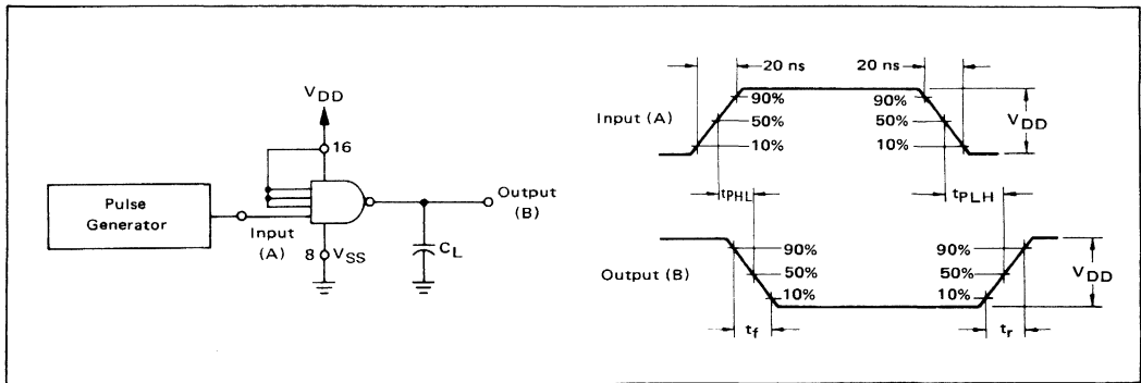
FIGURE 12 — SWITCHING TIME TEST CIRCUIT AND WAVEFORMS
