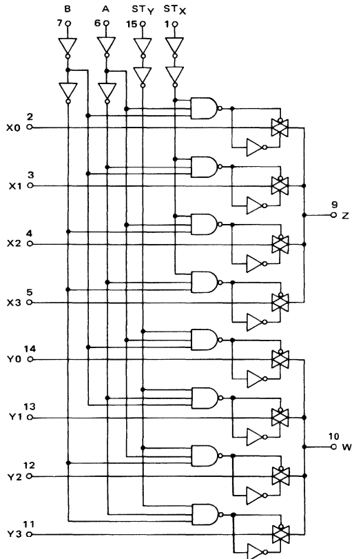
LOGIC DIAGRAM
