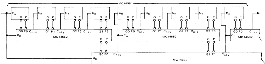
64 Bit ALU, Full Carry Look-Ahead in Three Levels.
