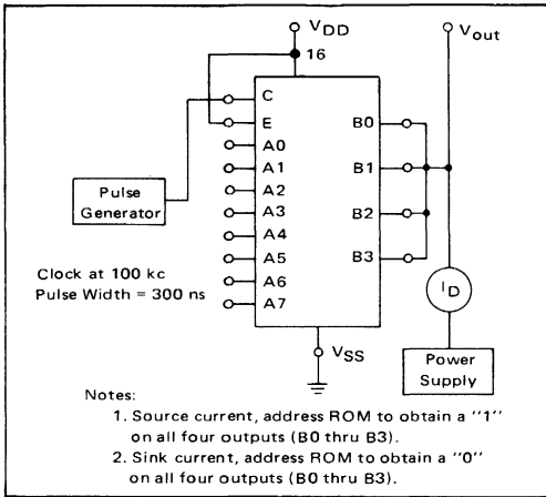
FIGURE 1 – OUTPUT DRIVE CURRENT TEST CIRCUIT
