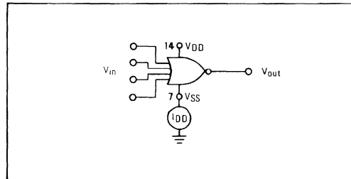
FIGURE 1 – CURRENT AND VOLTAGE TRANSFER CHARACTERISTICS TEST CIRCUIT
