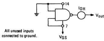
FIGURE 1 – TYPICAL OUTPUT SOURCE CHARACTERISTICS TEST CIRCUIT
