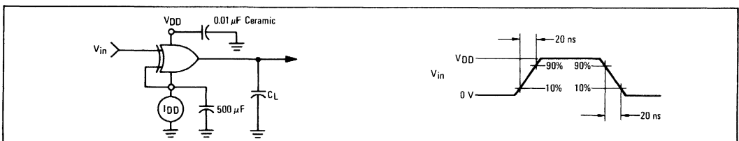
FIGURE 10 – POWER DISSIPATION TEST CIRCUIT AND WAVEFORM
