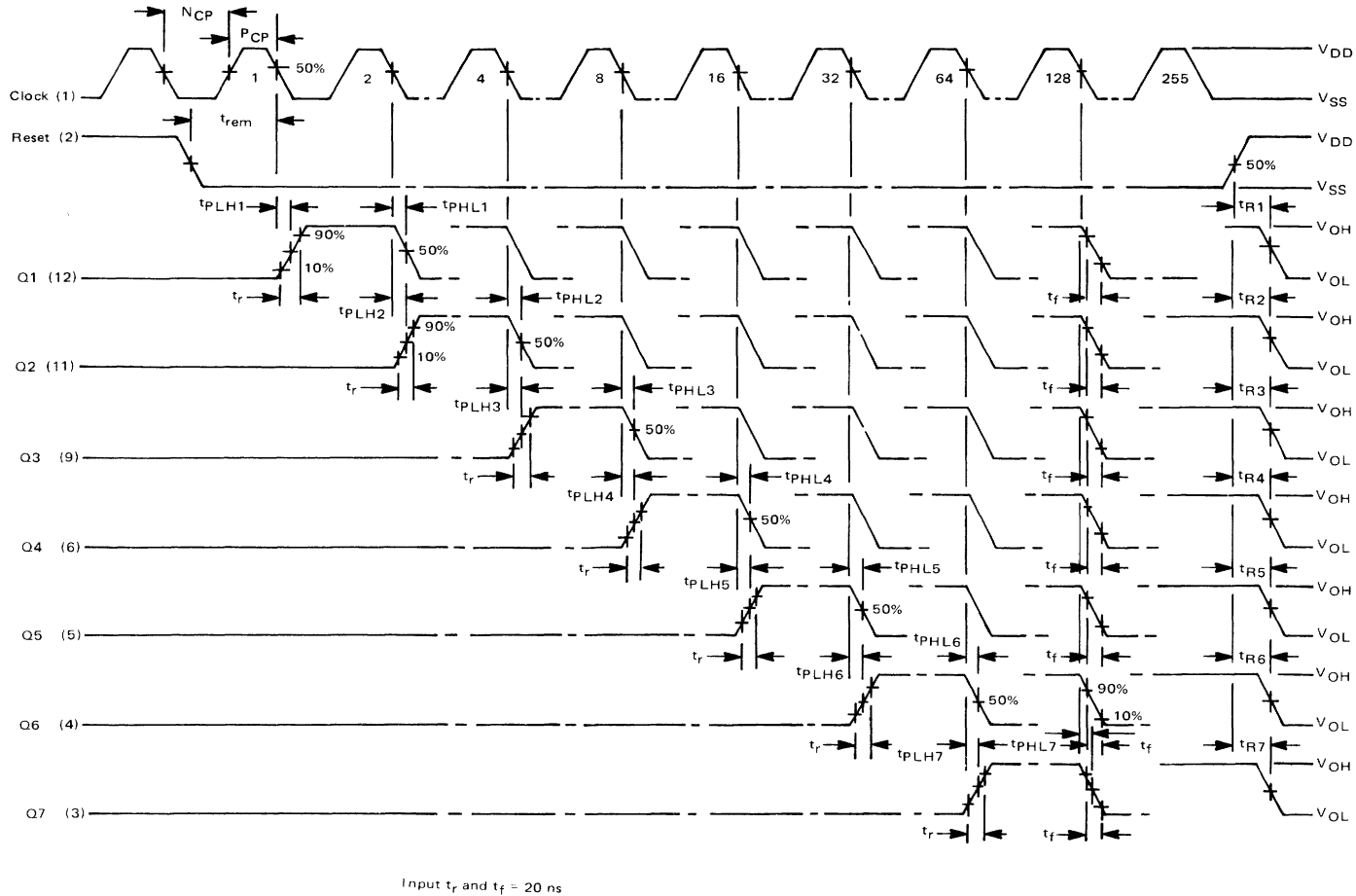
FIGURE 4 – FUNCTIONAL WAVEFORMS
