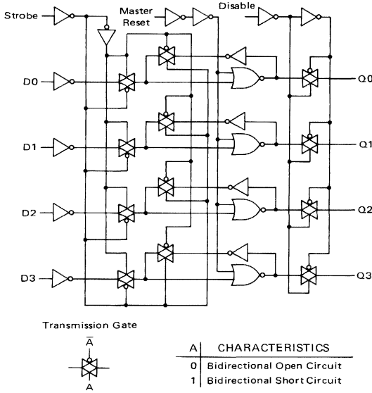
LOGIC DIAGRAM
