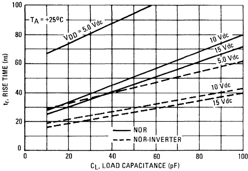
FIGURE 14 – TYPICAL RISE TIME versus LOAD CAPACITANCE
