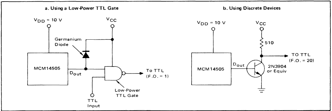
FIGURE 13 – CMOS-TO-TTL INTERFACE FOR V_{DD} = 10\text{ V}
