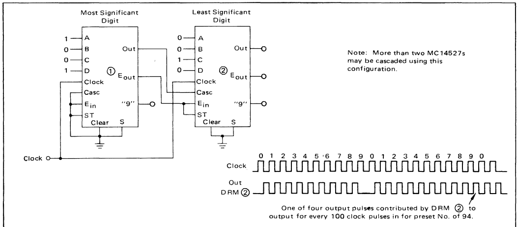
FIGURE 3 — TWO MC14527s IN CASCADE WITH PRESET NO. OF 94
