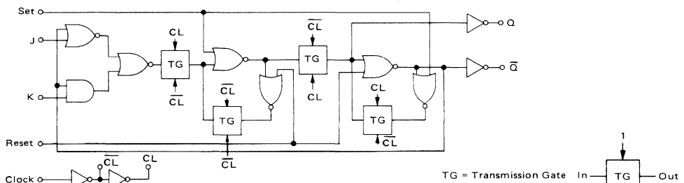
LOGIC DIAGRAM (1/2 OF CIRCUIT SHOWN)
