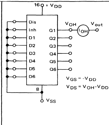
FIGURE 4 – TYPICAL OUTPUT SOURCE CHARACTERISTICS
