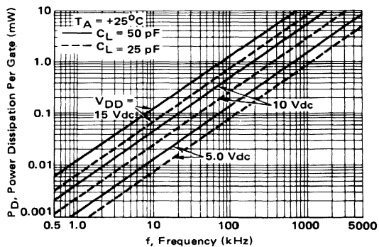
FIGURE 5-9 – GATE POWER DISSIPATION CHARACTERISTICS
