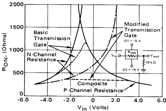
FIGURE 2-37 – McMOS TRANSMISSION GATES R_{ON} versus V_{in}
