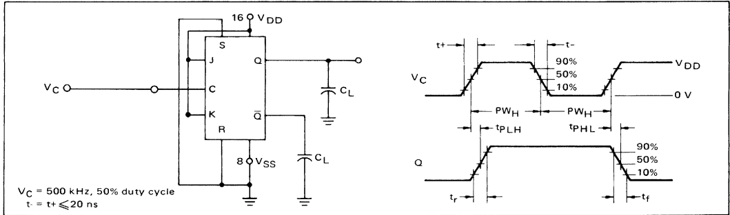
FIGURE 6 – SWITCHING TIME TEST CIRCUIT AND WAVEFORMS
