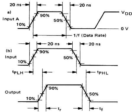
FIGURE 1 – DYNAMIC SIGNAL WAVEFORMS
