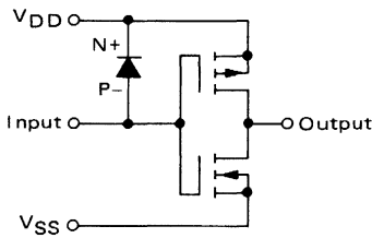
FIGURE 2-13(b) – SCHEMATIC DIAGRAM, SINGLE DIODE PROTECTION METHOD
