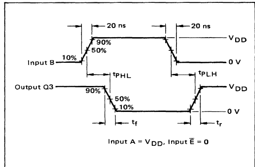
FIGURE 3 – DYNAMIC SIGNAL WAVEFORMS (MC14556)
