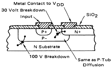
FIGURE 2-13(a) – PHYSICAL DIAGRAM, SINGLE DIODE PROTECTION METHOD
