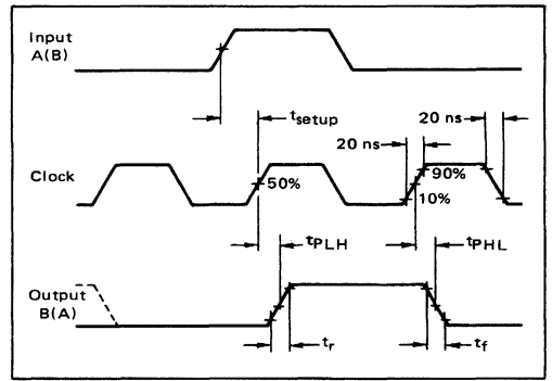
FIGURE 3 – PROPAGATION DELAY AND TRANSITION TIMES WAVEFORMS
