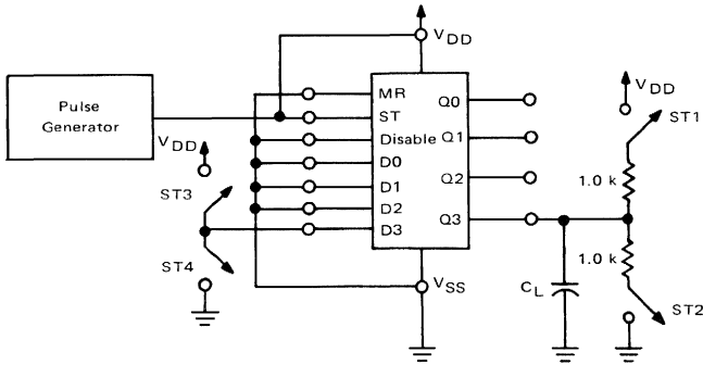
FIGURE 6 – 3-STATE AC TEST CIRCUIT
