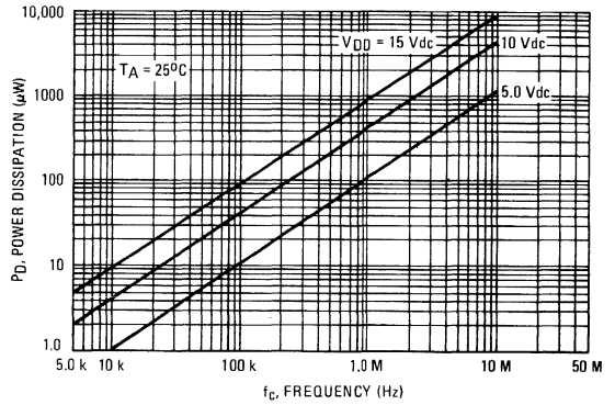
FIGURE 5 – TYPICAL POWER DISSIPATION PER CIRCUIT (1/4 OF DEVICE SHOWN)
