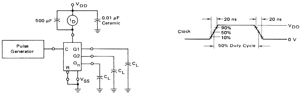
FIGURE 1 – POWER DISSIPATION TEST CIRCUIT AND WAVEFORM
