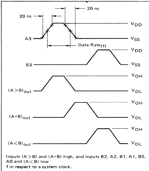
FIGURE 3 – CASCADING COMPARATORS
