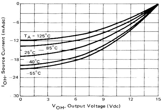
FIGURE 5-3 – V_{GS} = -15 \text{ Vdc} , V_{DD} = 15 \text{ Vdc}
