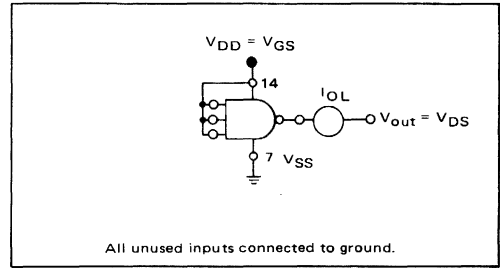
FIGURE 2 – TYPICAL OUTPUT SINK CHARACTERISTICS
