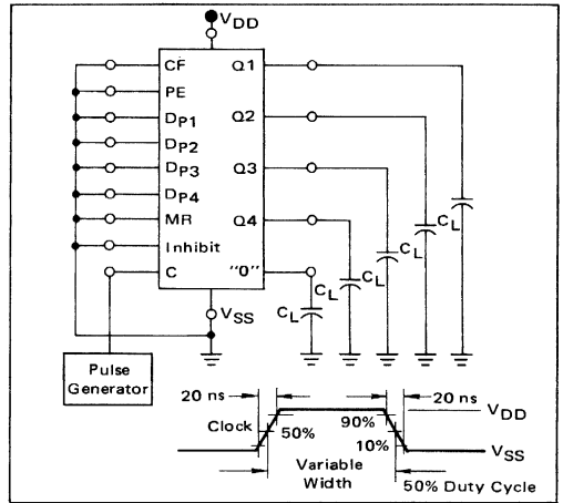
FIGURE 4 – POWER DISSIPATION
