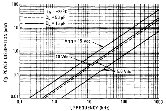
FIGURE 7 – POWER DISSIPATION CHARACTERISTICS
