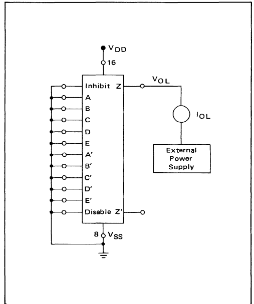
FIGURE 3 – TYPICAL OUTPUT SINK CHARACTERISTICS TEST CIRCUIT
