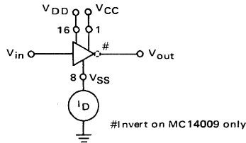
FIGURE 1 – CURRENT AND VOLTAGE TRANSFER CHARACTERISTICS TEST CIRCUIT
