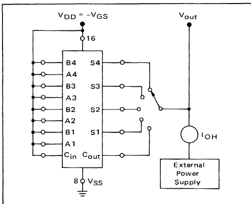
FIGURE 1 – TYPICAL SOURCE CURRENT CHARACTERISTICS TEST CIRCUIT
