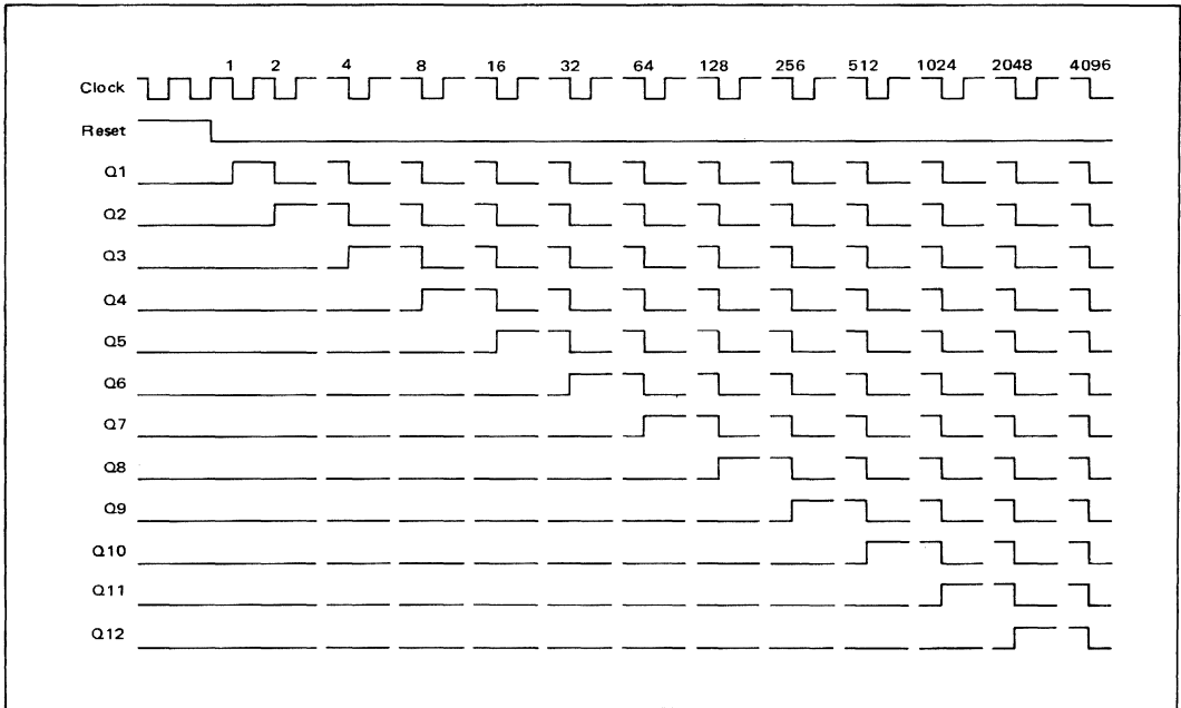
FIGURE 3 – TIMING DIAGRAM
