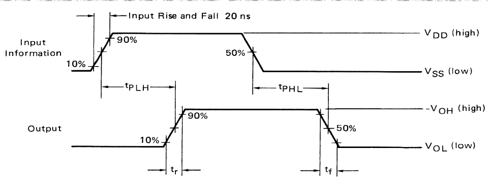
FIGURE 5-14 – NON-SYNCHRONOUS CIRCUIT WAVESHAPES AND TIMING PARAMETERS
