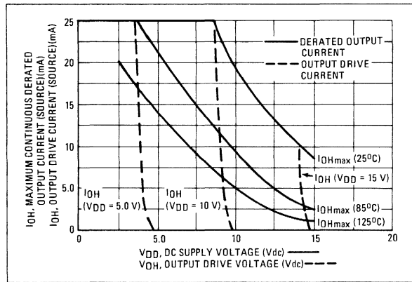
FIGURE 1 – DERATING AND OUTPUT DRIVE CURVES PER OUTPUT
