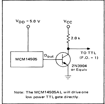
FIGURE 12 – CMOS-TO-TTL INTERFACE FOR V_{DD} = 5.0\text{ V}
