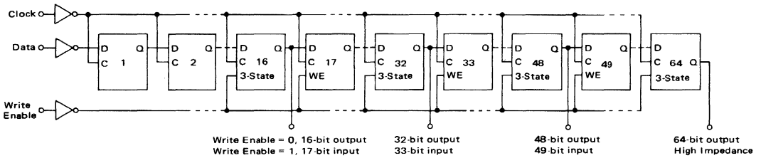
EXPANDED BLOCK DIAGRAM (1/2 OF DEVICE SHOWN)
