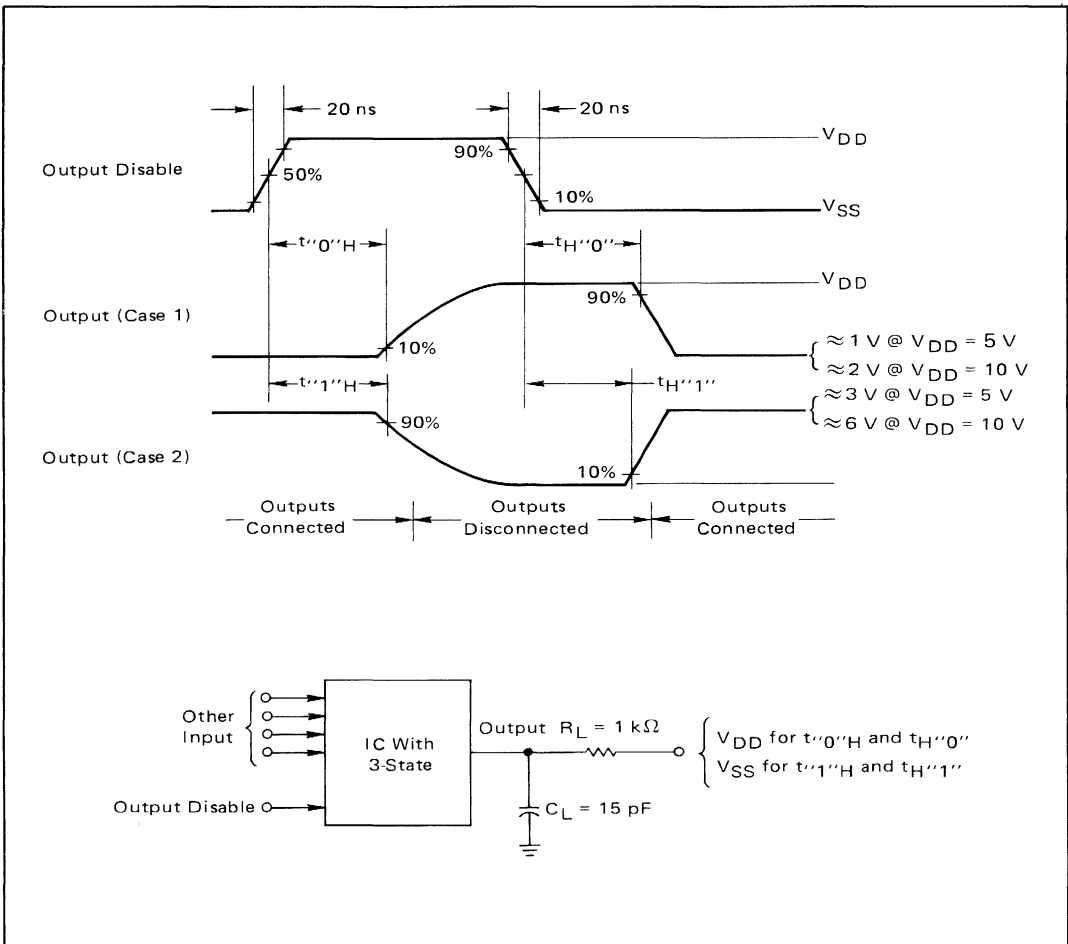
FIGURE 5-16 – THREE-STATE PROPAGATION DELAY WAVESHAPES AND CIRCUIT
