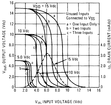
FIGURE 2 – TYPICAL VOLTAGE AND CURRENT TRANSFER CHARACTERISTICS
