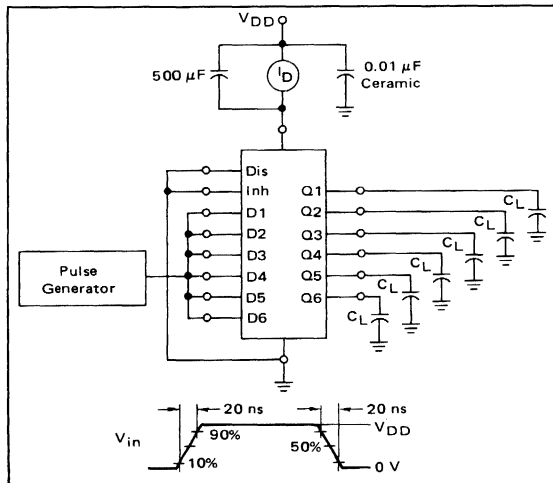
FIGURE 6 – POWER DISSIPATION TEST CIRCUIT AND WAVEFORM
