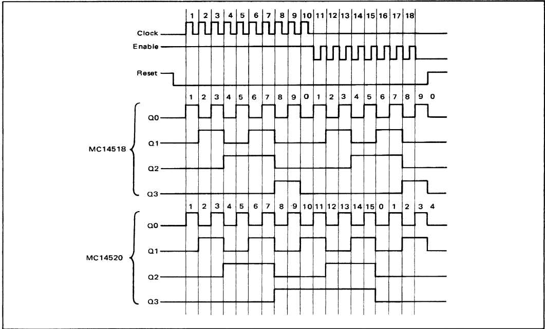
FIGURE 8 – TIMING DIAGRAM
