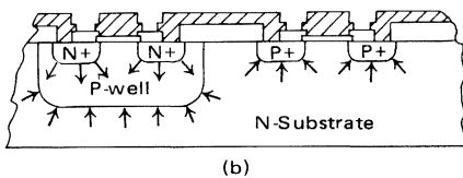
FIGURE 2-3 – LEAKAGE CURRENTS OF P-N DIODE JUNCTIONS
