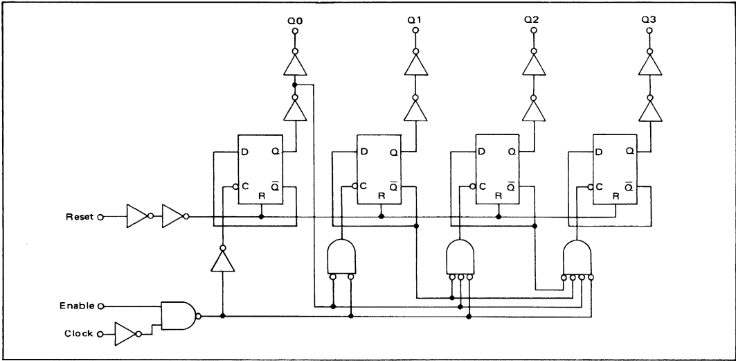
FIGURE 10 – BINARY COUNTER (MC14520) LOGIC DIAGRAM (1/2 OF DEVICE SHOWN)
