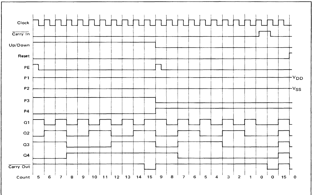
TIMING DIAGRAM
