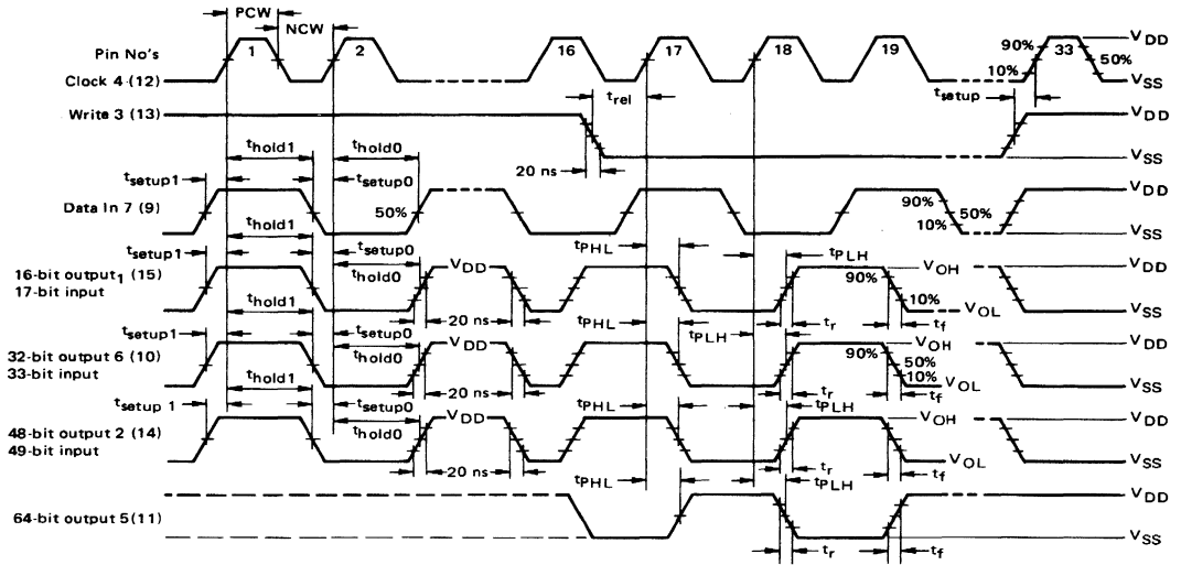
FIGURE 4 – AC TEST WAVEFORMS
