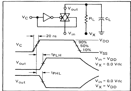
FIGURE 9 – TURN-ON DELAY TIME TEST CIRCUIT AND WAVEFORMS
