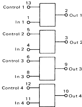
MC14016 Quad Analog Switch Quad Multiplexer
