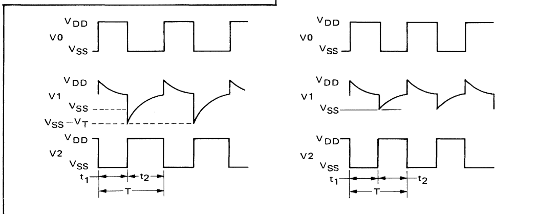
FIGURE 2-15 – WAVEFORM COMPARISON OF INPUT METHODS
