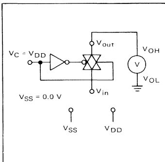
FIGURE 1 – OUTPUT VOLTAGE TEST CIRCUIT
