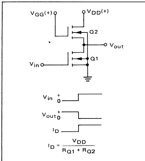
FIGURE 1-3 – TYPICAL N-CHANNEL INVERTER
