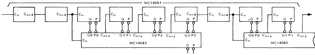
Combined two-level look-ahead and ripple-carry ALU
