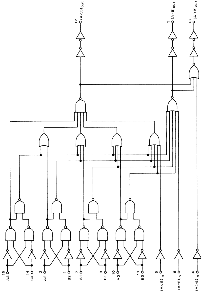
LOGIC DIAGRAM
