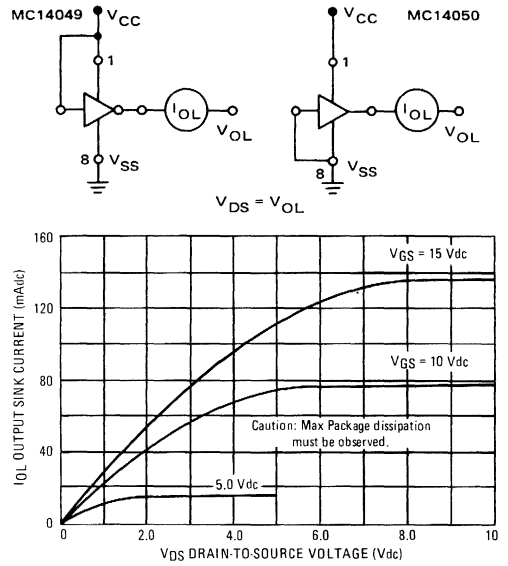
FIGURE 4 – TYPICAL OUTPUT SINK CHARACTERISTICS
