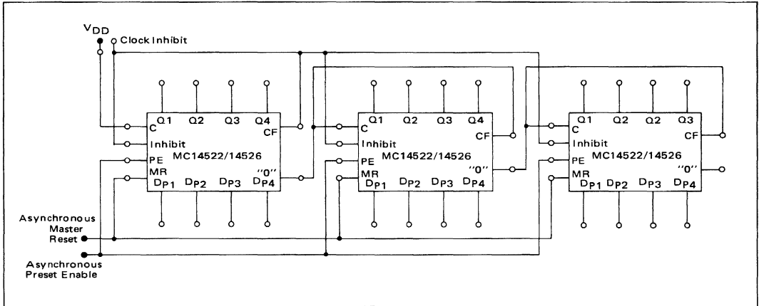
FIGURE 9 – SYNCHRONOUS PROGRAMMABLE DOWN COUNTER
