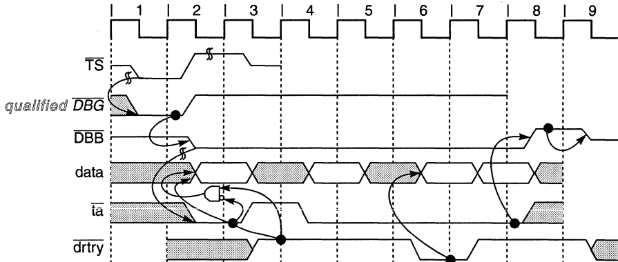
Figure 3-13. Read Burst with \overline{\text{TA}} Wait States and \overline{\text{DRTRY}}
