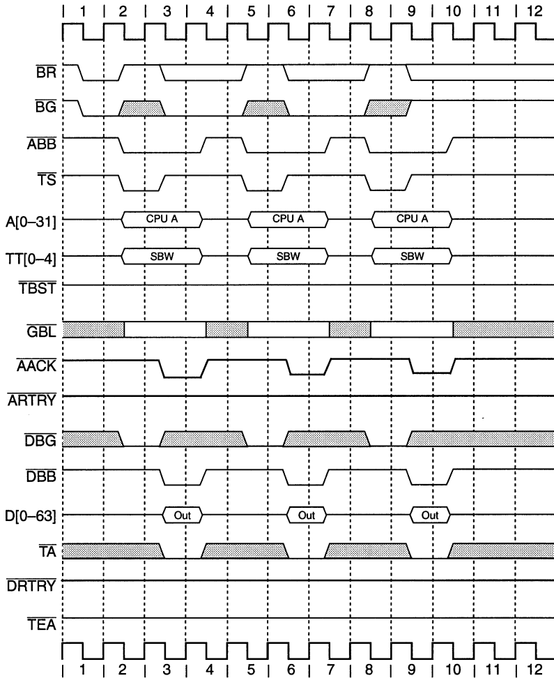
Figure 3-15. Fastest Single-Beat Writes
