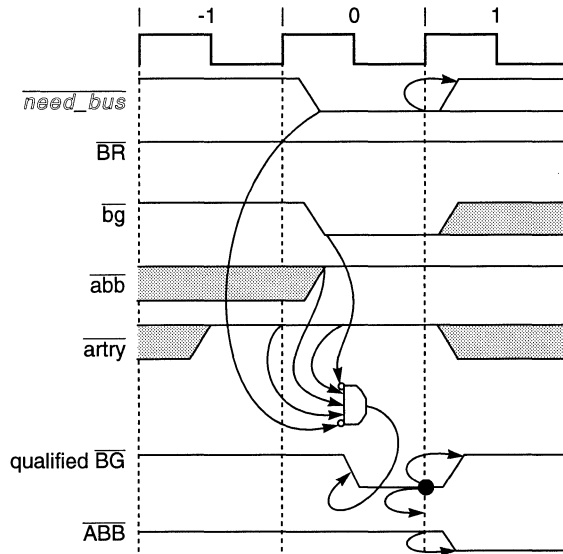
Figure 3-4. Address Bus Arbitration Showing Bus Parking
