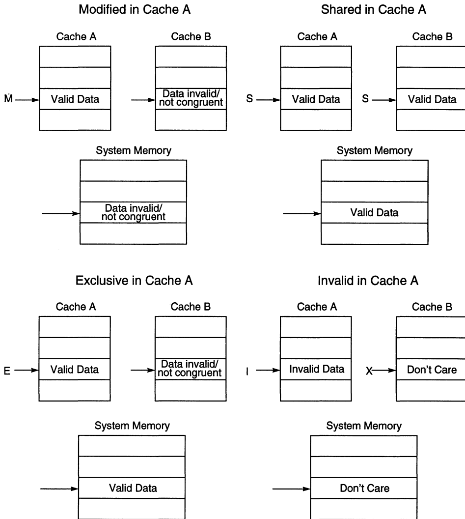
Figure 4-5. MESI States
