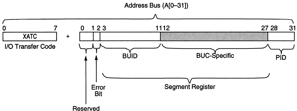
Figure 7-4. I/O Reply Operation
