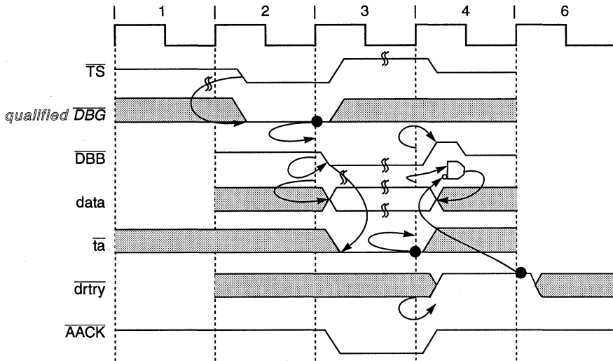
Figure 3-9. Normal Single-Beat Read Termination
