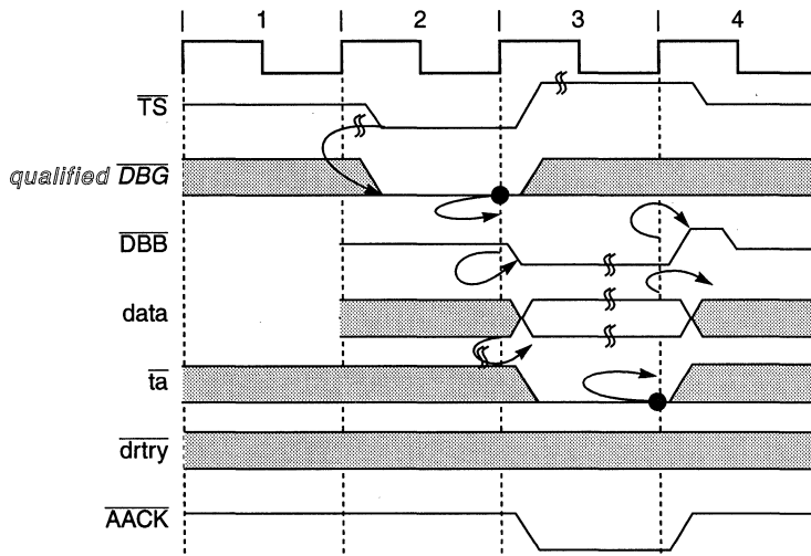
Figure 3-10. Normal Single-Beat Write Termination
