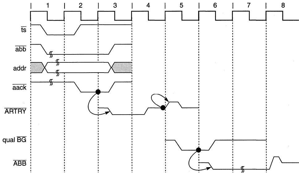
Figure 3-6. Snoop Address Cycle with \overline{ARTRY}
