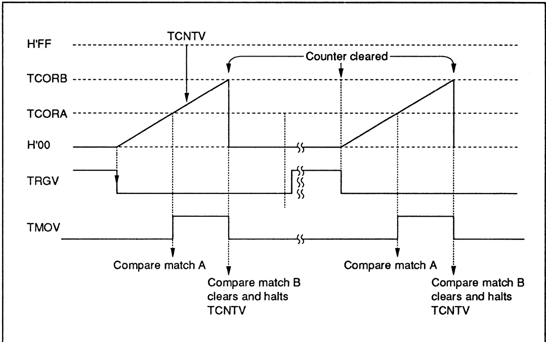
Figure 9-12 Pulse Output Synchronized to TRGV Input
