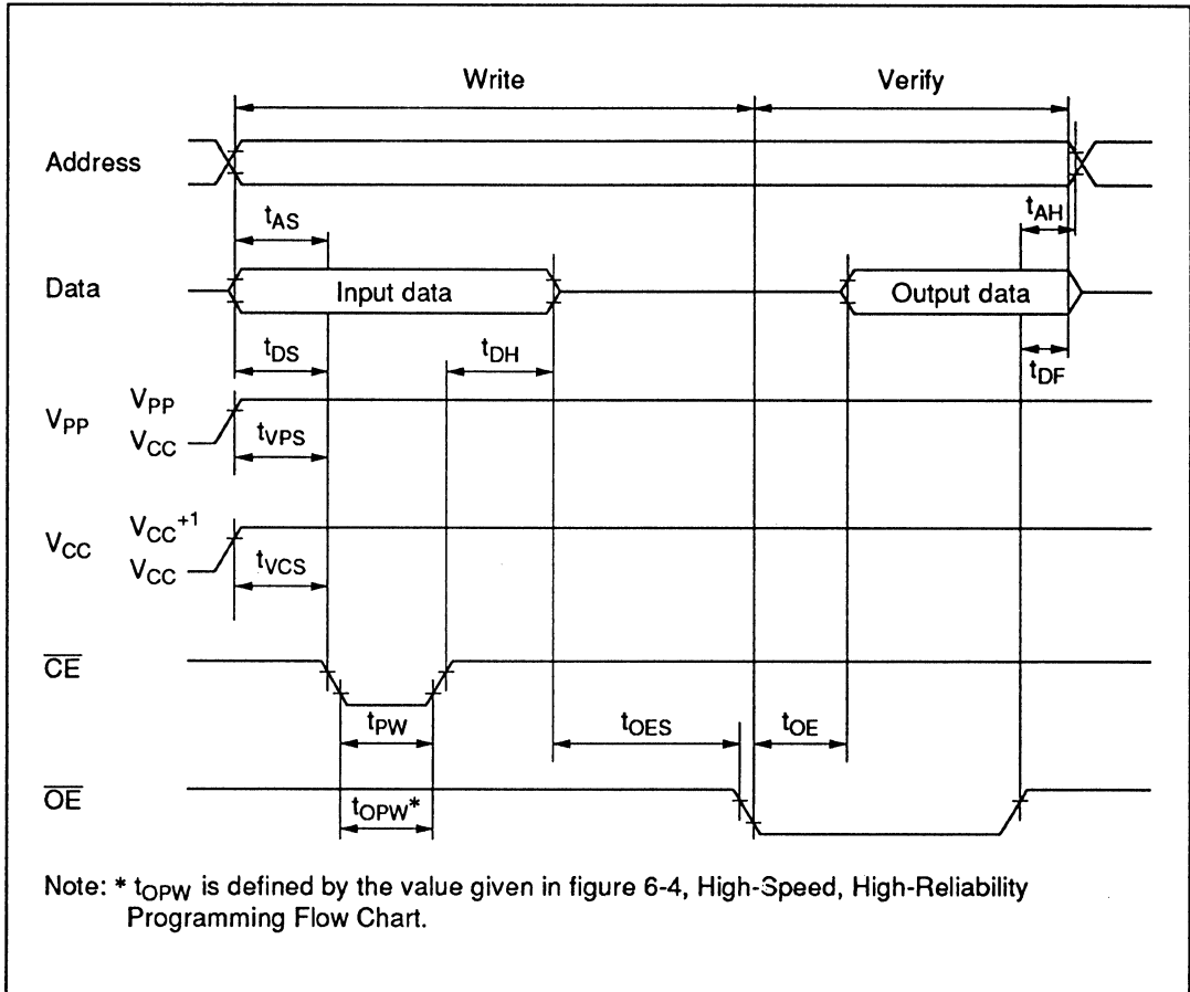
Figure 6-5 PROM Write/Verify Timing
