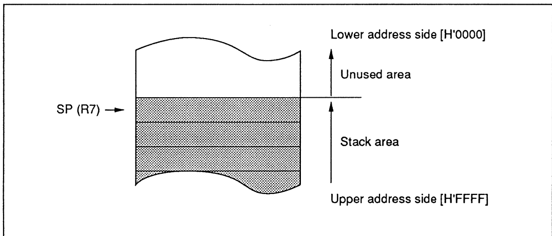
Figure 2-2 Stack Pointer
