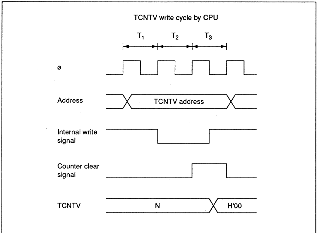
Figure 9-13 Contention between TCNTV Write and Clear
