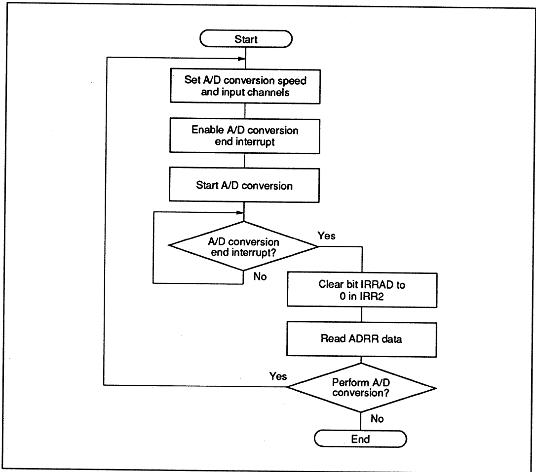
Figure 12-5 Flow Chart of Procedure for Using A/D Converter (2) (Interrupts Used)
