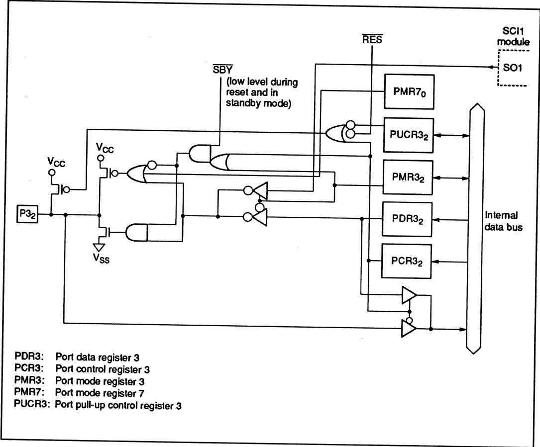
Figure C-3 (a) Port 3 Block Diagram (Pin P3 2 )
