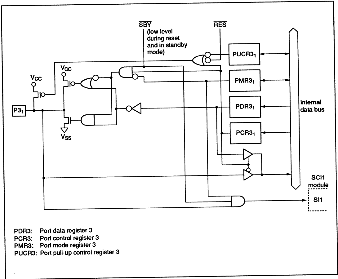
Figure C-3 (b) Port 3 Block Diagram (Pin P3 1 )
