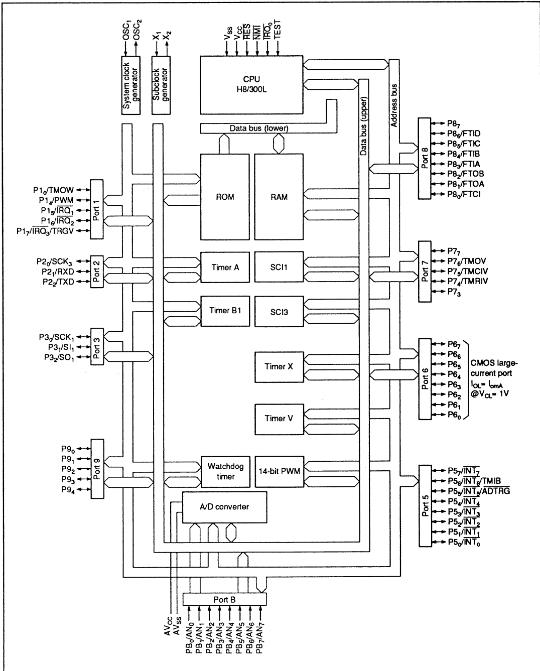
Figure 1-1 Block Diagram
