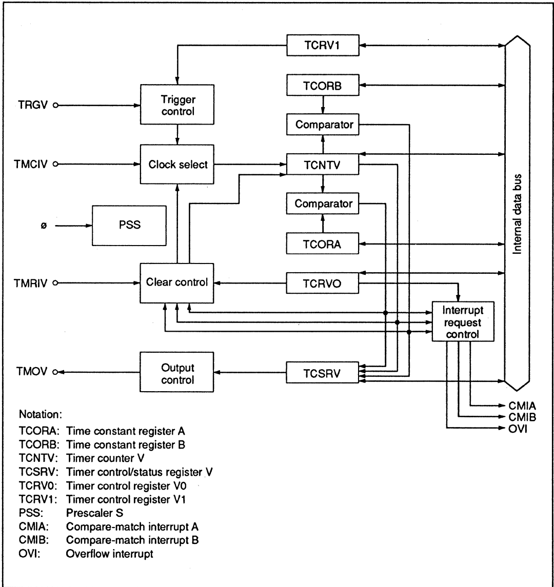
Figure 9-3 Block Diagram of Timer V
