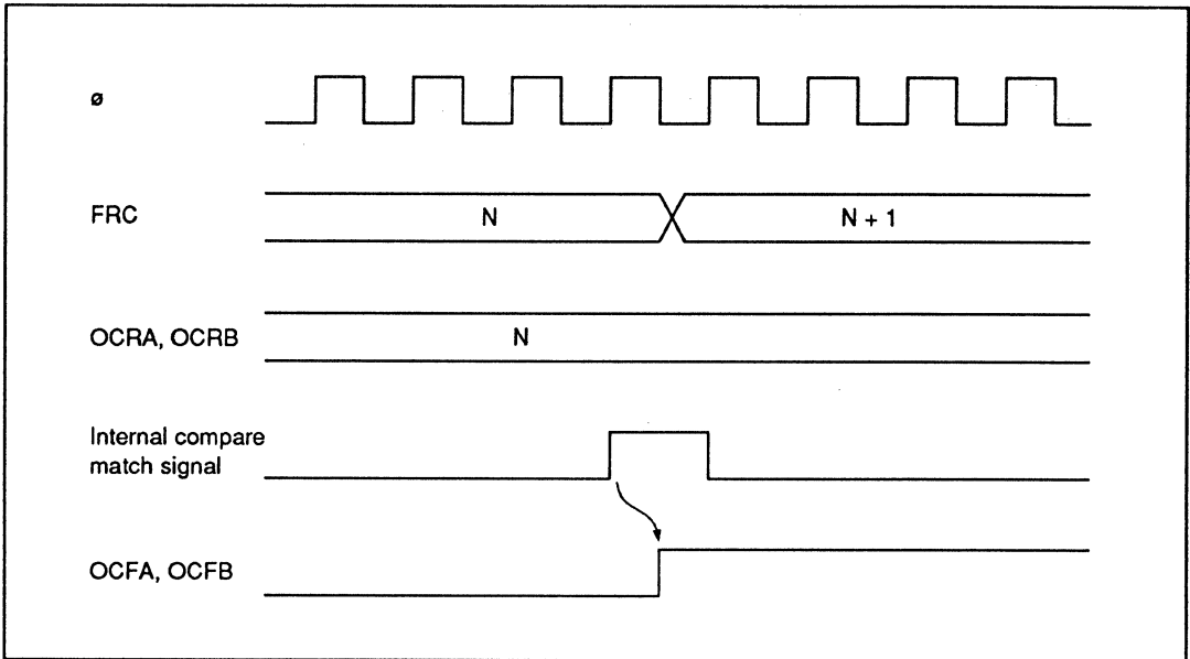
Figure 9-29 OCFA and OCFB Set Timing
