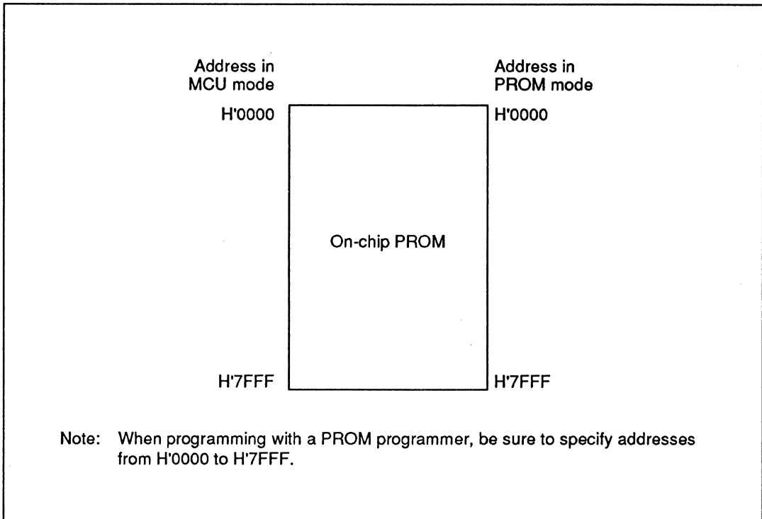
Figure 6-3 H8/3644 Memory Map in PROM Mode
