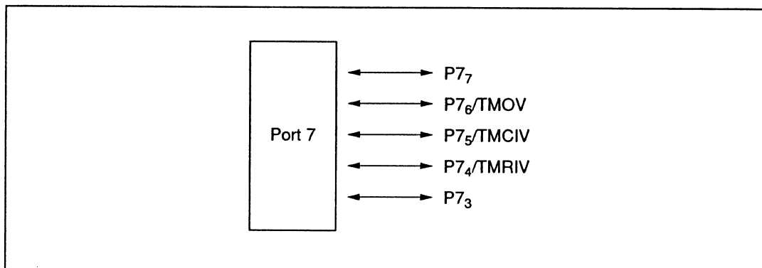
Figure 8-6 Port 7 Pin Configuration
