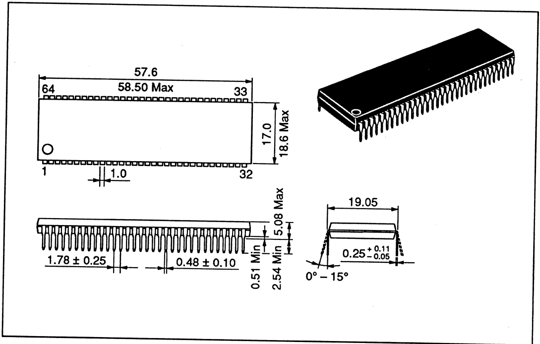
Figure F-2 DP-64S Package Dimensions
