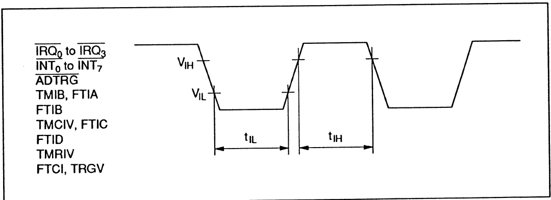
Figure 13-3 Input Timing
