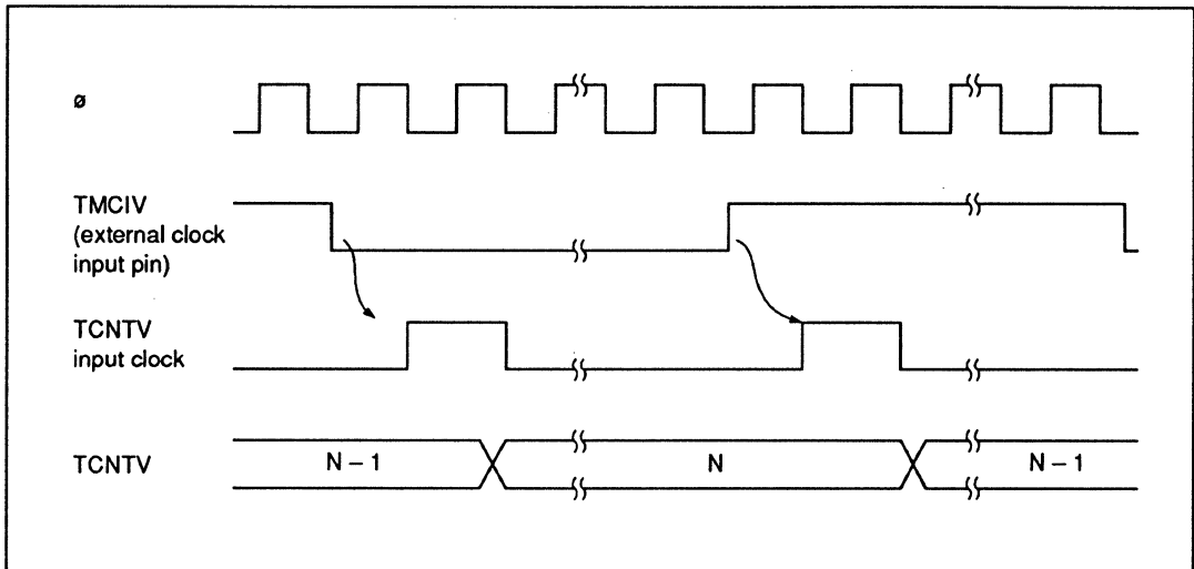
Figure 9-5 Increment Timing with External Clock
