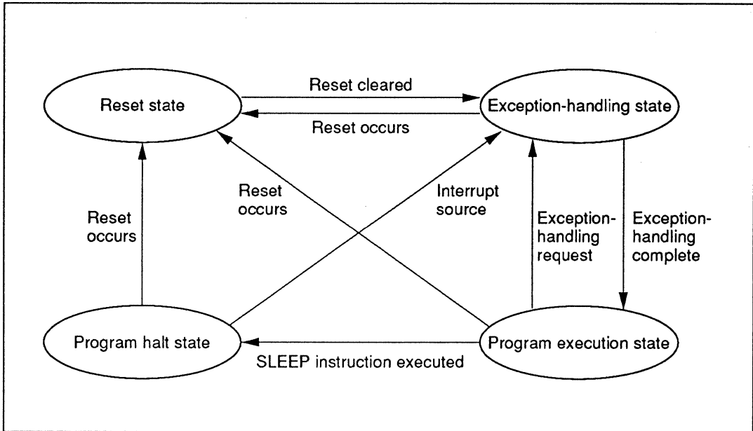
Figure 2-15 State Transitions
