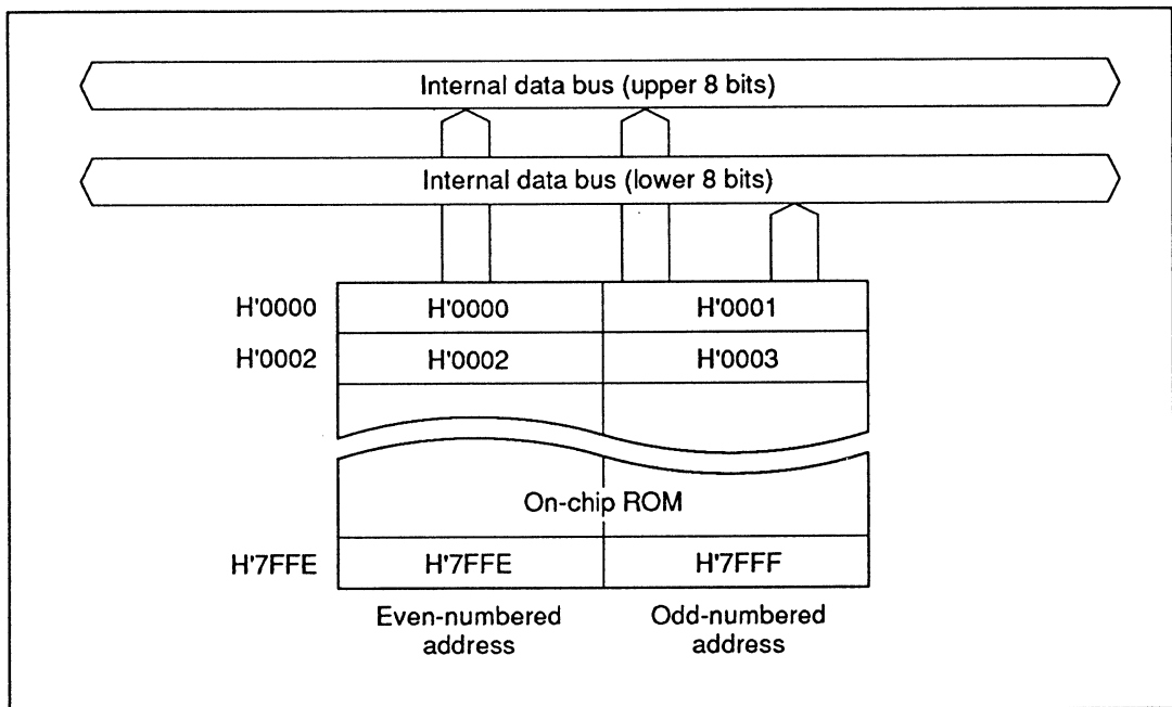
Figure 6-1 ROM Block Diagram (H8/3644)
