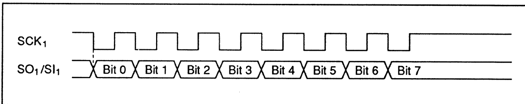
Figure 10-2 Transfer Format
