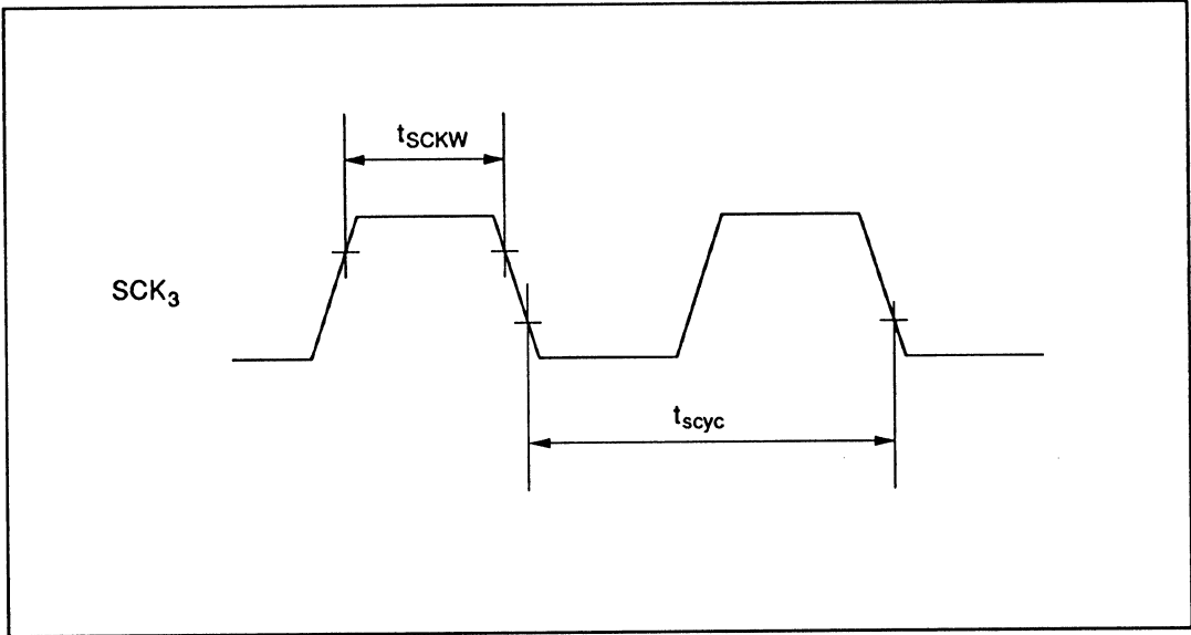
Figure 13-5 SCK_3 Input Clock Timing
