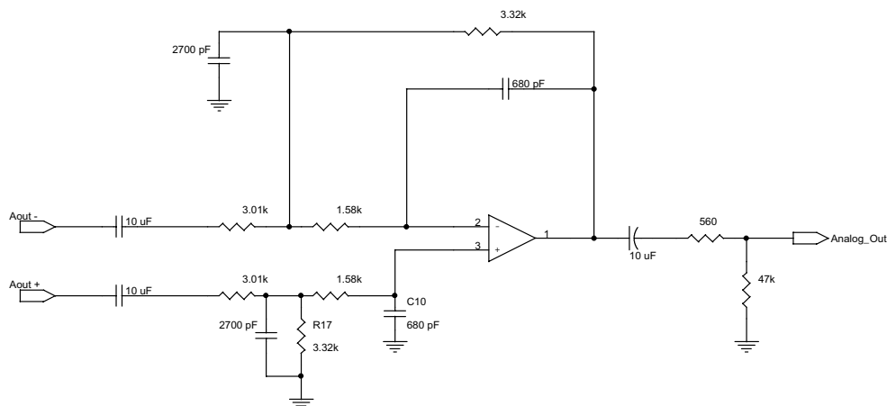
Figure 3. CS4392 Output Filter
