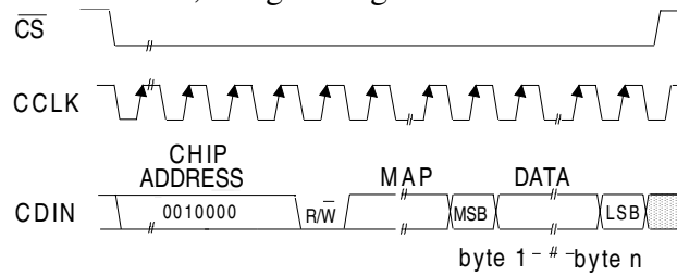
Figure 9. Control Port Timing, SPI mode
