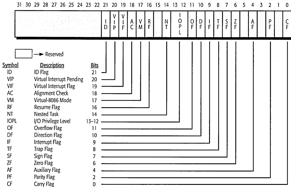
Figure 17. EFLAGS Registers
