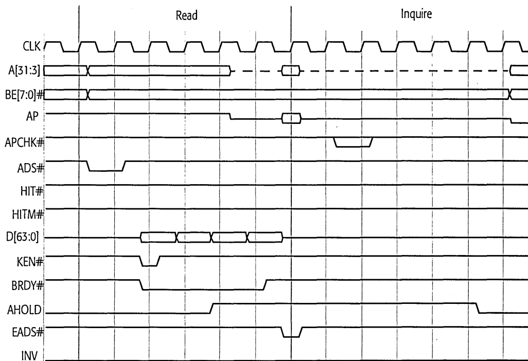
Figure 55. AHOLD-Initiated Inquire Miss
