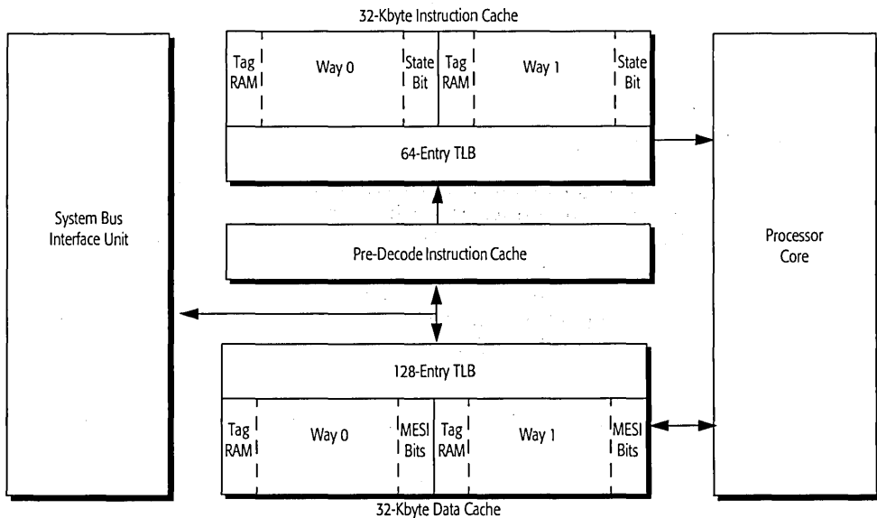
Figure 68. Cache Organization
