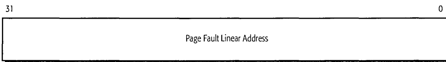
Figure 20. Control Register 2 (CR2)
