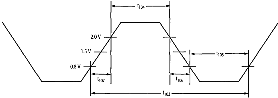
Figure 89. TCK Waveform
