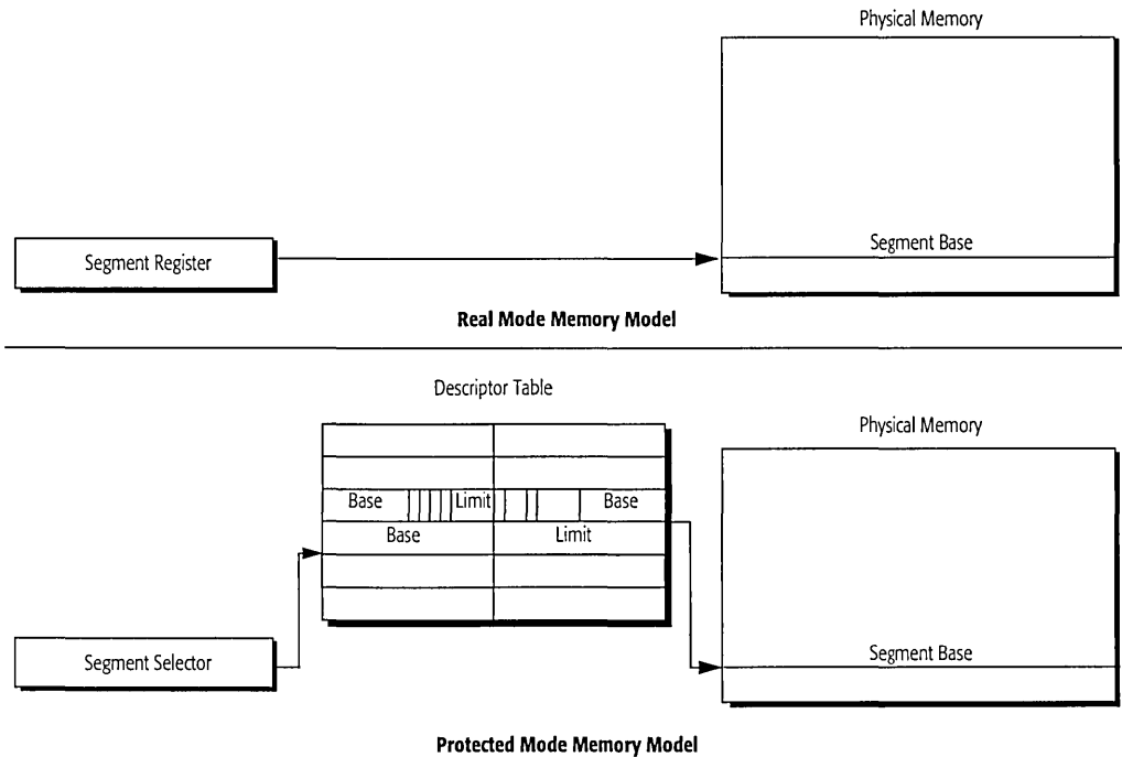
Figure 9. Segment Usage
