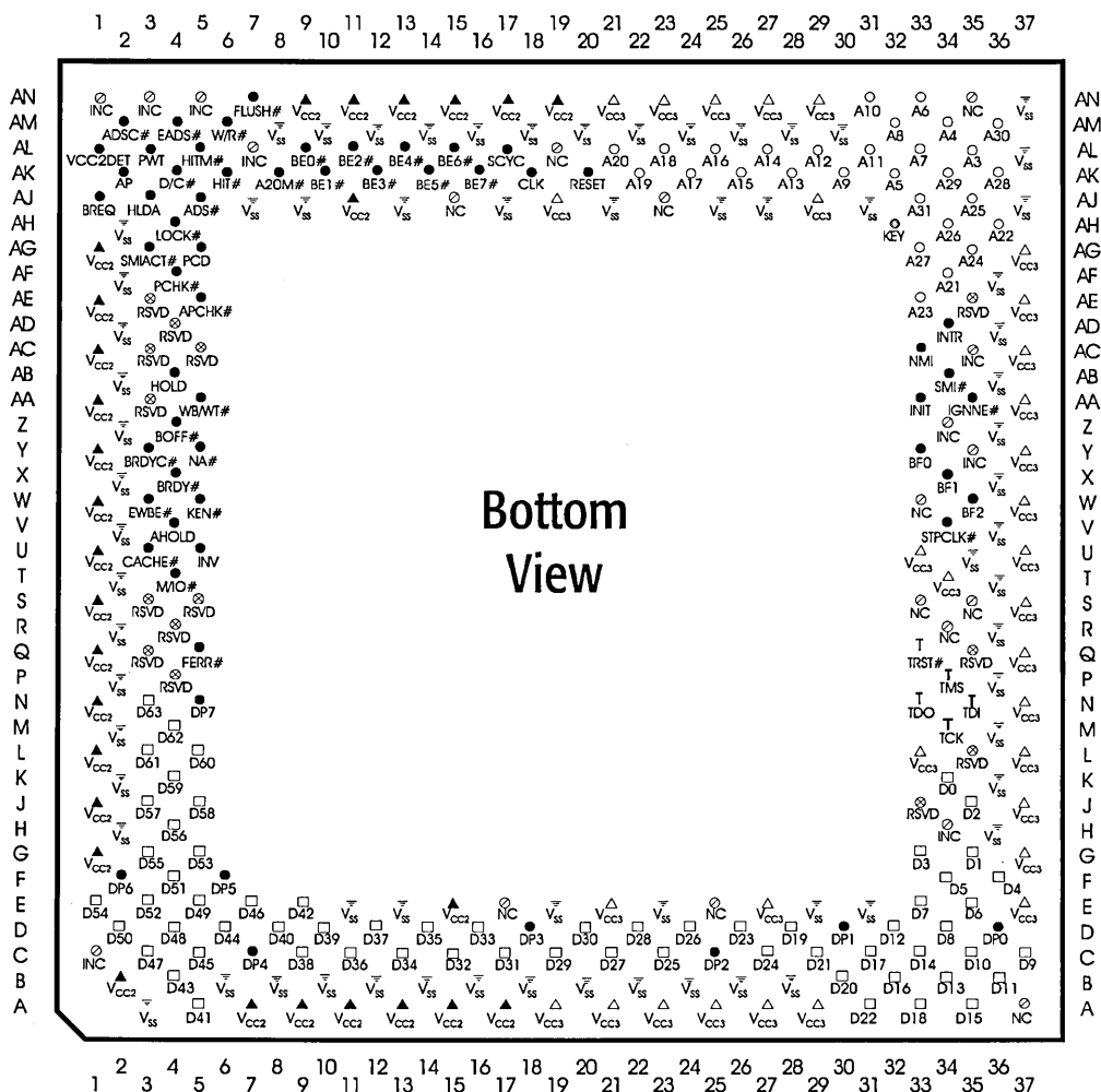
Figure 100. AMD-K6™ MMX™ Enhanced Processor Pin-Side View
