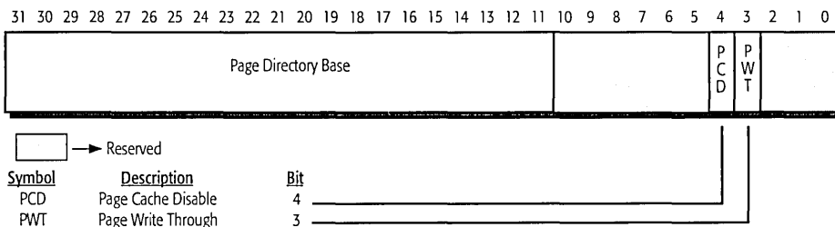
Figure 19. Control Register 3 (CR3)
