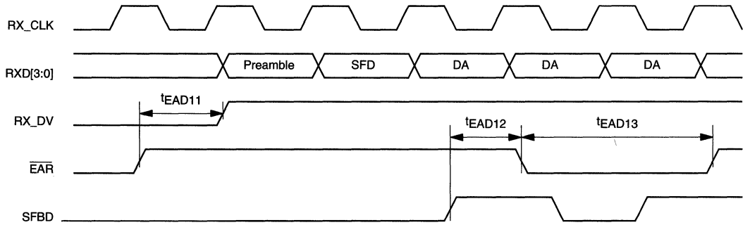
Figure C-10. Reject Timing - External PHY MII @ 2.5 MHz
