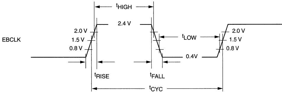
Figure 69. EBCLK Waveform
