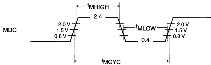
Figure C-6. MDC Waveform
