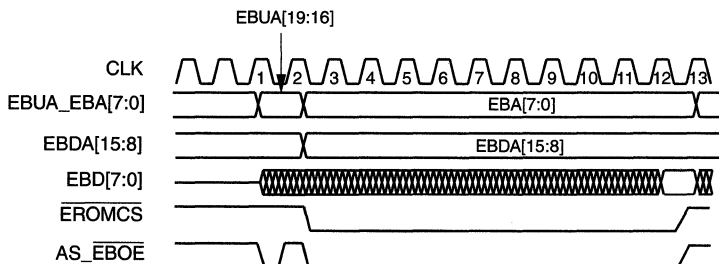
Figure 44. Flash Read from Expansion Bus Data Port
