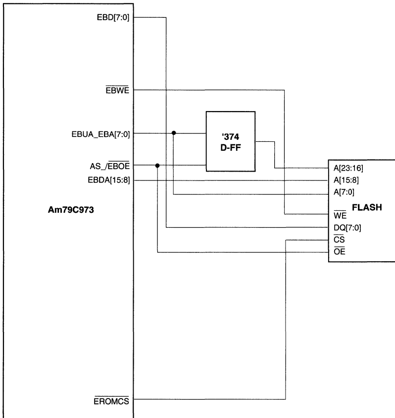
Figure 40. Flash Configuration for the Expansion Bus
