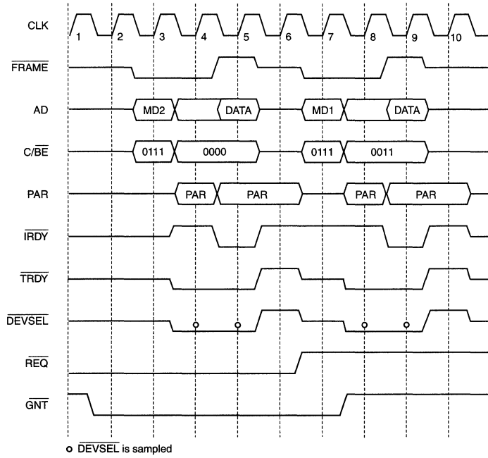
Figure 27. Descriptor Ring Write In Non-Burst Mode
