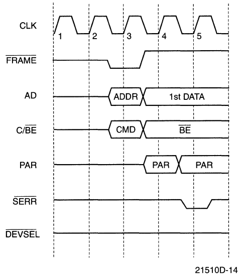
Figure 9. Address Parity Error Response
