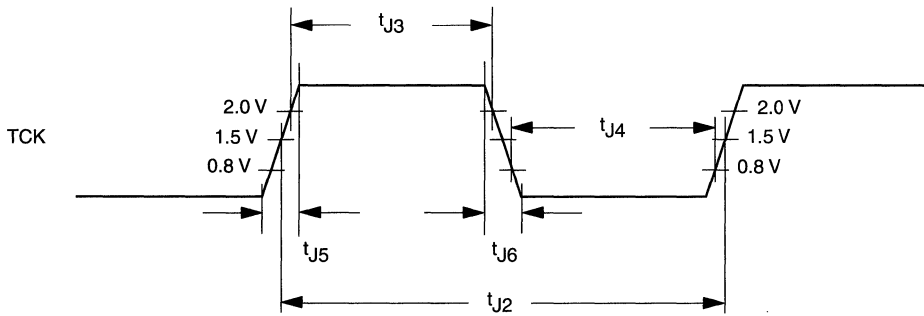
Figure 67. JTAG (IEEE 1149.1) TCK Waveform for 5 V Signaling
