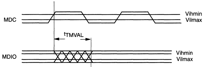
Figure C-8. Management Data Output Valid Delay Timing
