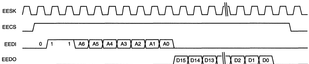
Figure 65. EEPROM Read Functional Timing
