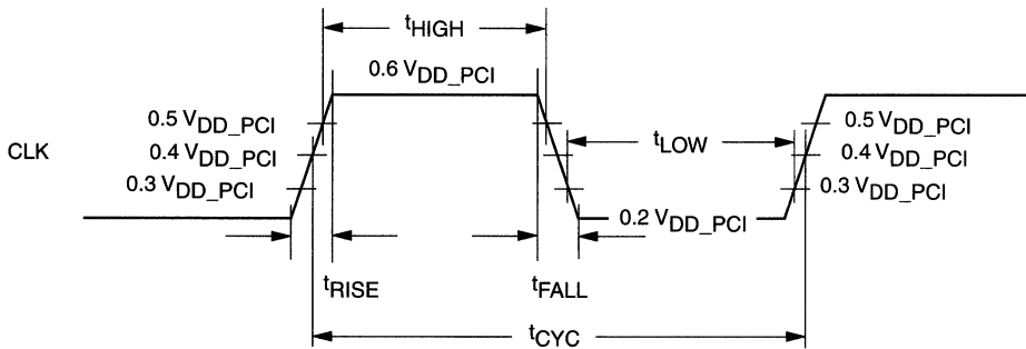
Figure 61. CLK Waveform for 3.3 V Signaling
