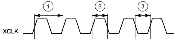
Figure 54. Clock Timing
