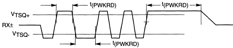
Figure 58. 10 Mbps Receive (RX±) Timing Diagram
