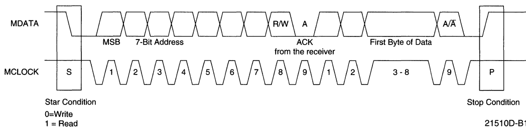
Figure B-1. Standard Data Transfer on the Serial Management Interface
