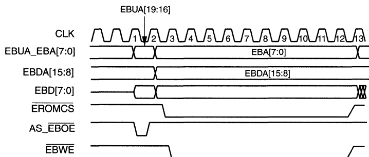
Figure 45. Flash Write from Expansion Bus Data Port
