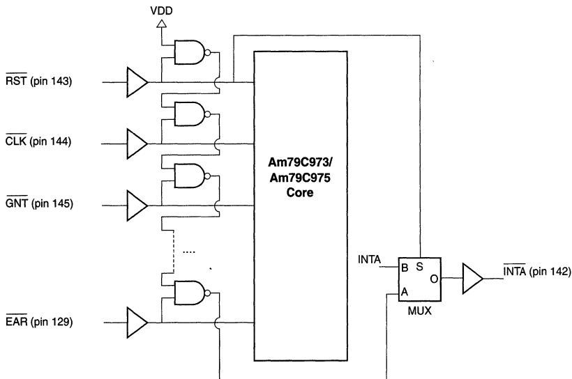
Figure 51. NAND Tree Circuitry
