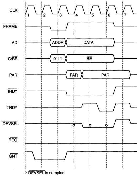
Figure 19. Preemption During Non-Burst Transaction
