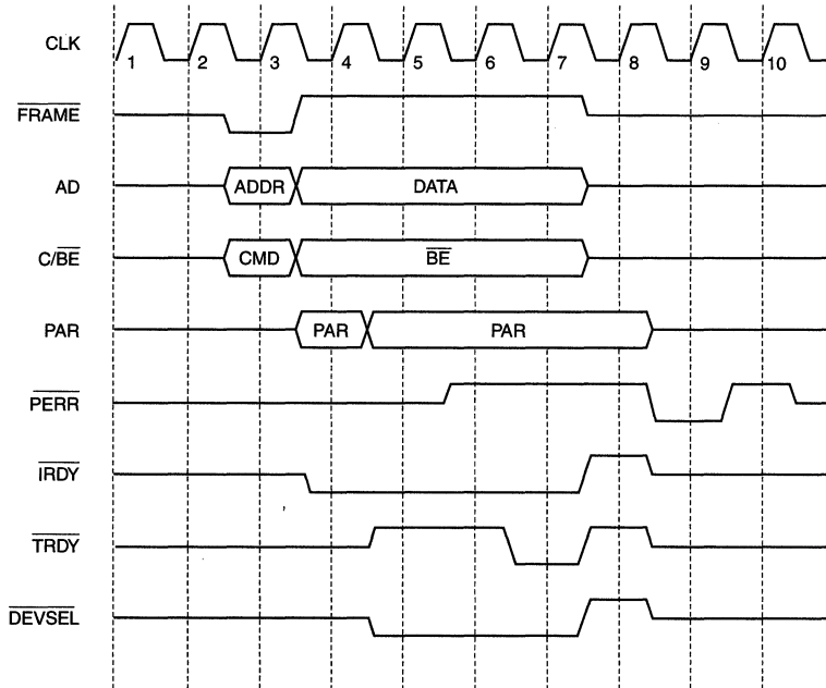
Figure 10. Slave Cycle Data Parity Error Response
