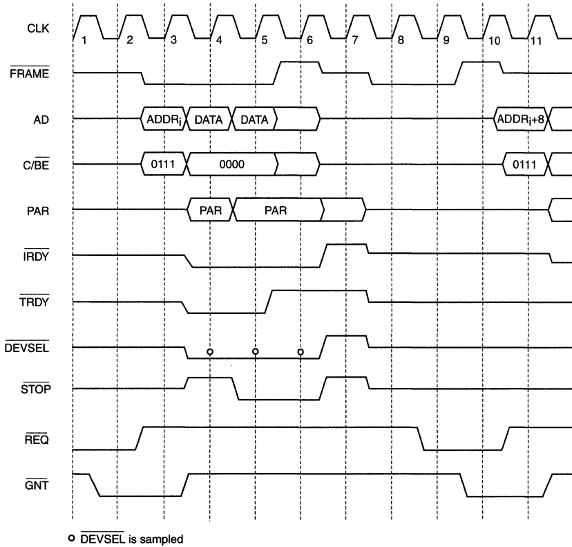
Figure 16. Disconnect With Data Transfer
