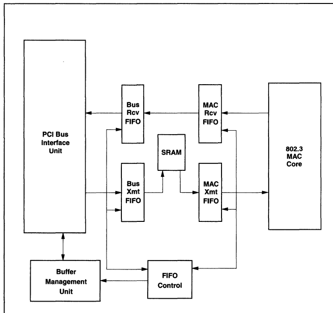
Figure 47. Block Diagram Low Latency Receive Configuration
