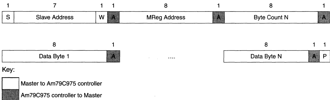
Figure B-5. Block Write Command
