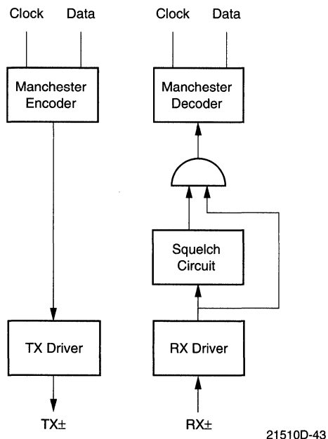
Figure 38. 10BASE-T Transmit and Receive Data Paths
