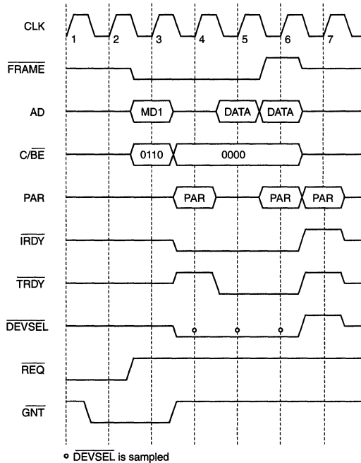
Figure 26. Descriptor Ring Read In Burst Mode
