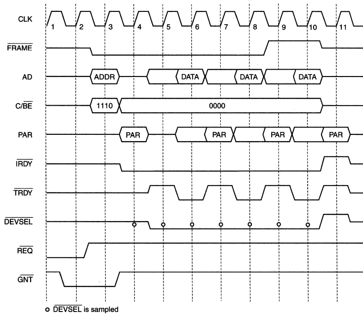
Figure 13. Burst Read Transfer (EXTREQ = 0, MEMCMD = 0)
