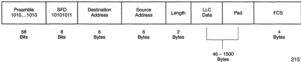
Figure 33. ISO 802-3 (IEEE/ANSI 802.3) Data Frame
