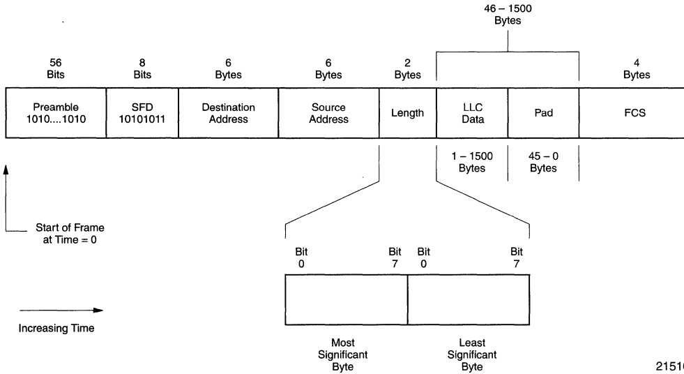
Figure 34. IEEE 802.3 Frame And Length Field Transmission Order
