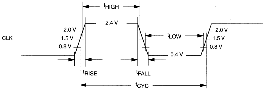
Figure 60. CLK Waveform for 5 V Signaling
