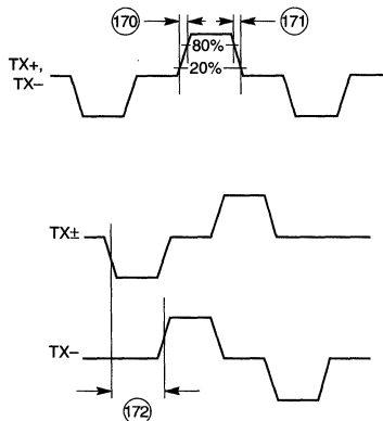
Figure 56. PMD Interface Timing (MLT-3)
