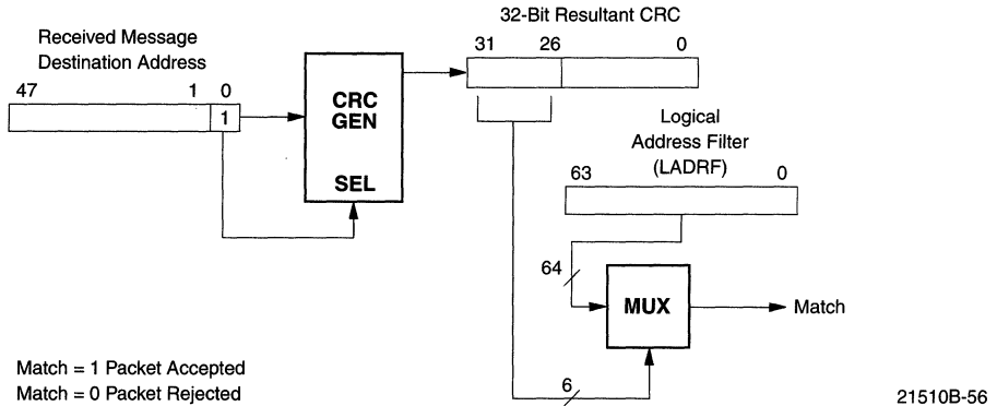
Figure 53. Address Match Logic
