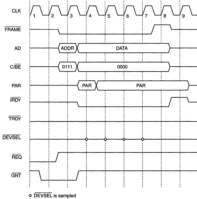
Figure 21. Master Abort
