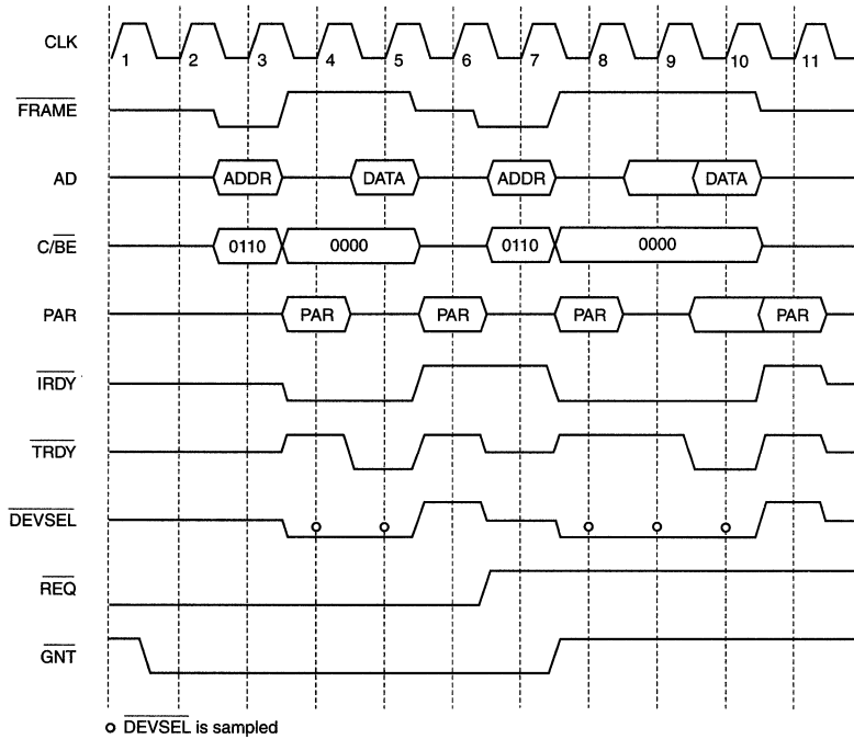
Figure 12. Non-Burst Read Transfer
