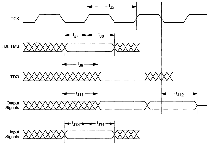
Figure 68. JTAG (IEEE 1149.1) Test Signal Timing
