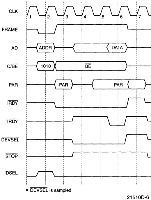
Figure 1. Slave Configuration Read
