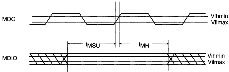
Figure C-7. Management Data Setup and Hold Timing
