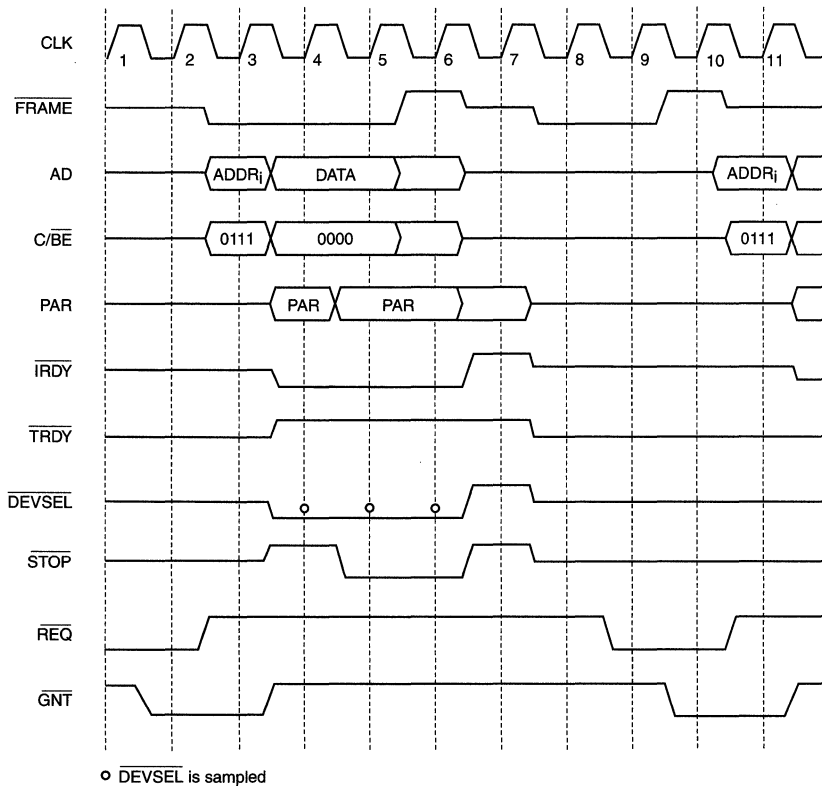
Figure 17. Disconnect Without Data Transfer
