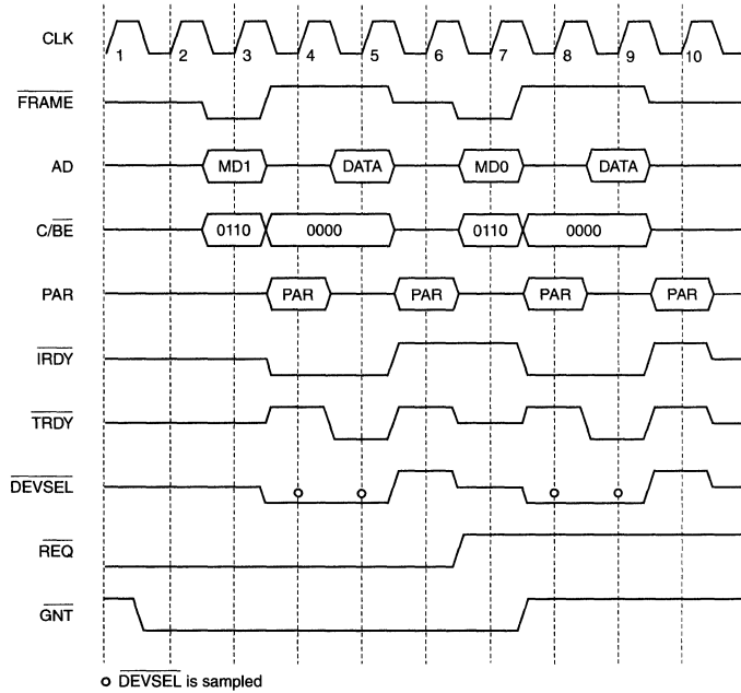
Figure 25. Descriptor Ring Read In Non-Burst Mode
