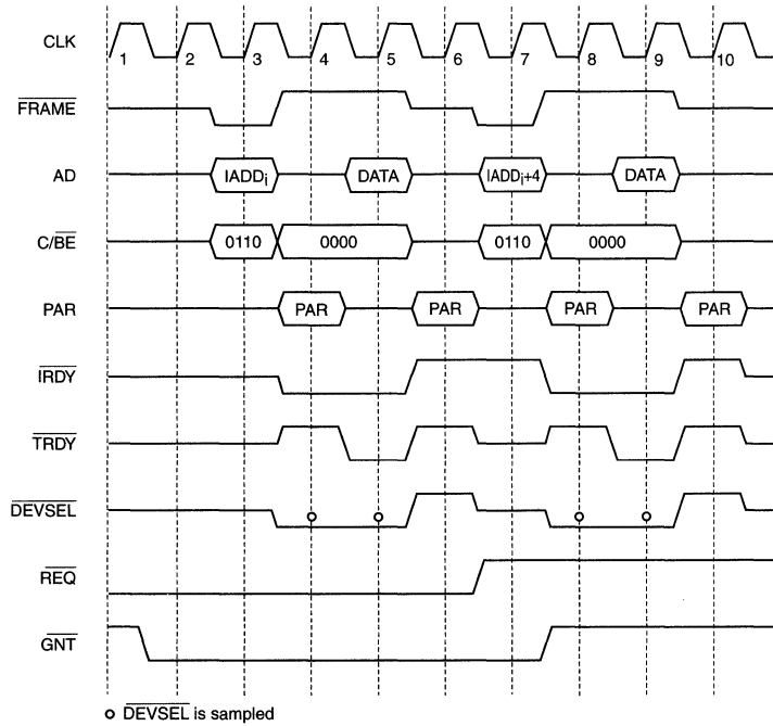
Figure 23. Initialization Block Read In Non-Burst Mode
