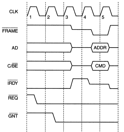
Figure 11. Bus Acquisition
