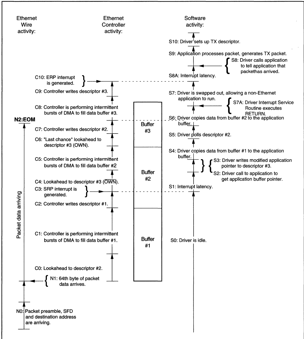
Figure E-3. LAPP Timeline for Two-Interrupt Method
