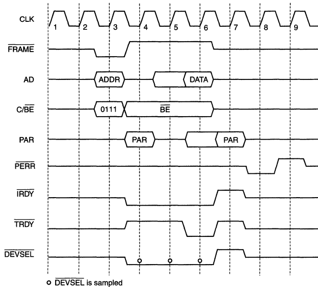
Figure 22. Master Cycle Data Parity Error Response
