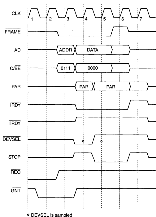
Figure 18. Target Abort
