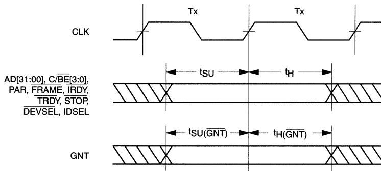
Figure 62. Input Setup and Hold Timing
