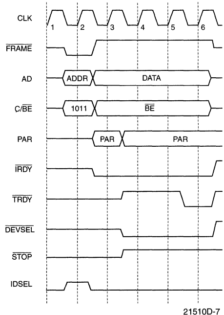
Figure 2. Slave Configuration Write
