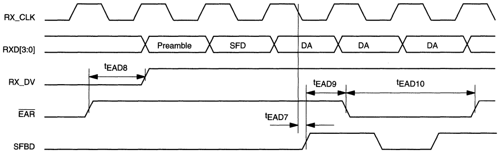
Figure C-9. Reject Timing - External PHY MII @ 25 MHz
