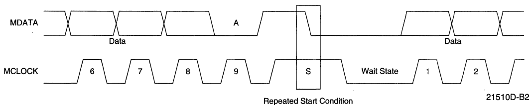
Figure B-2. Data Transfer with Change in Direction (with wait state)
