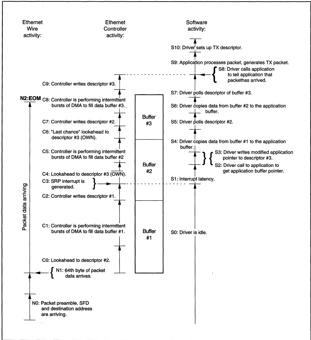
Figure E-1. LAPP Timeline
