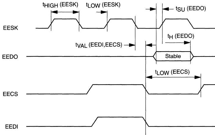
Figure 66. Automatic PREAD EEPROM Timing
