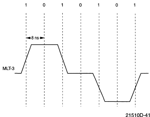
Figure 36. MLT-3 Waveform
