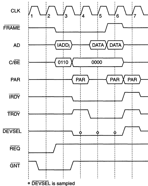
Figure 24. Initialization Block Read In Burst Mode
