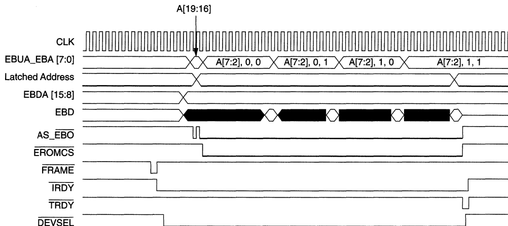
Figure 43. Expansion ROM Bus Read Sequence
