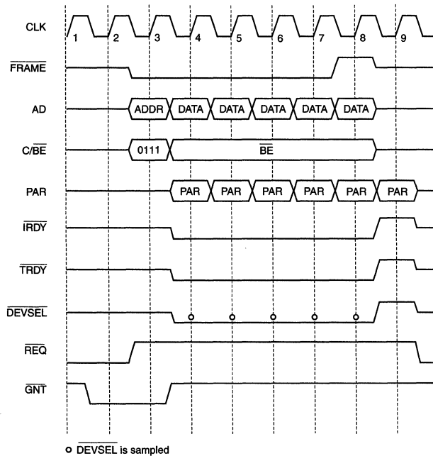
Figure 20. Preemption During Burst Transaction
