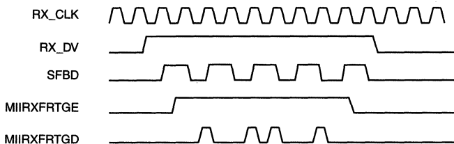
Figure C-3. MII Receive Frame Tagging
