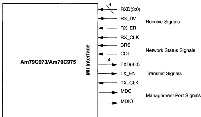
Figure C-1. Media Independent Interface
