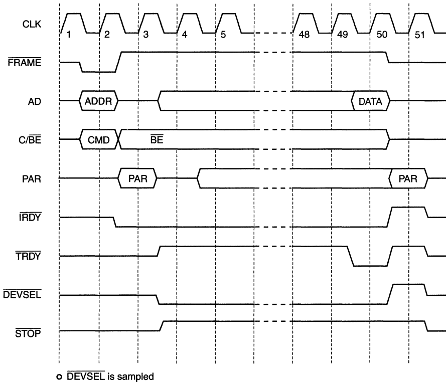
Figure 5. Expansion ROM Read
