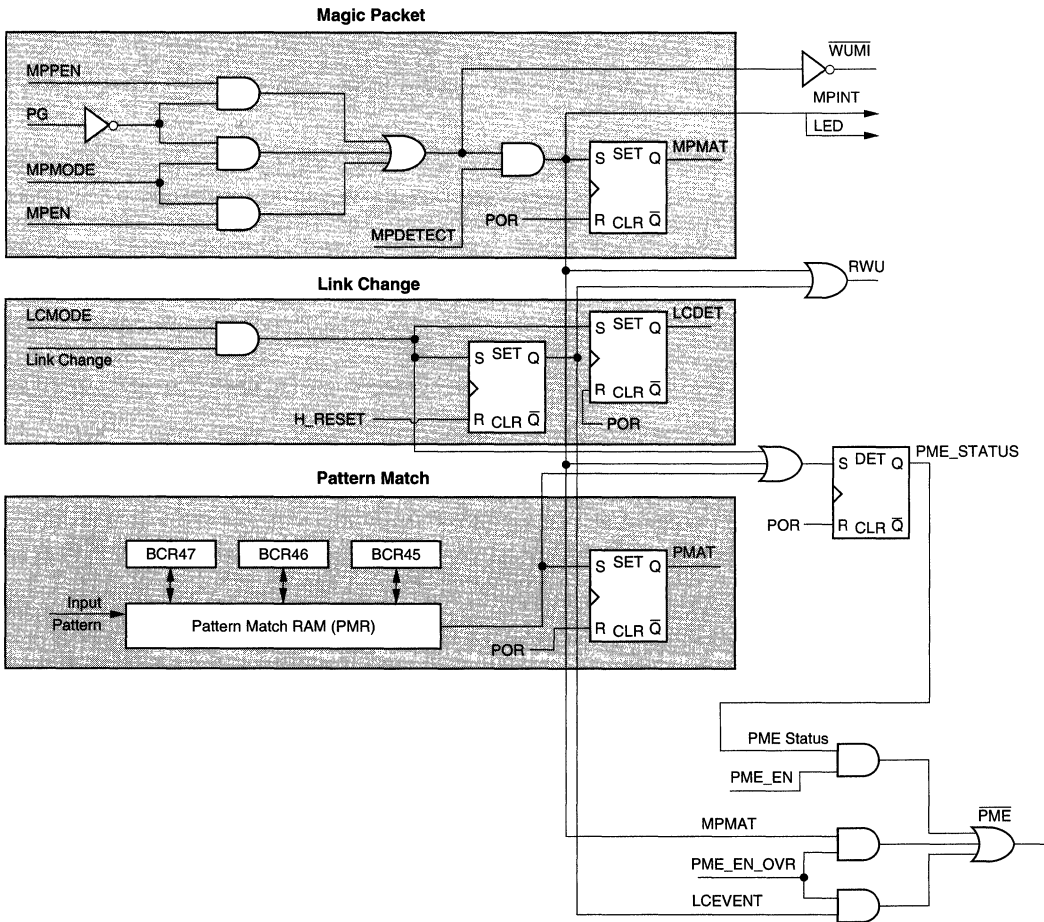
Figure 49. OnNow Functional Diagram
