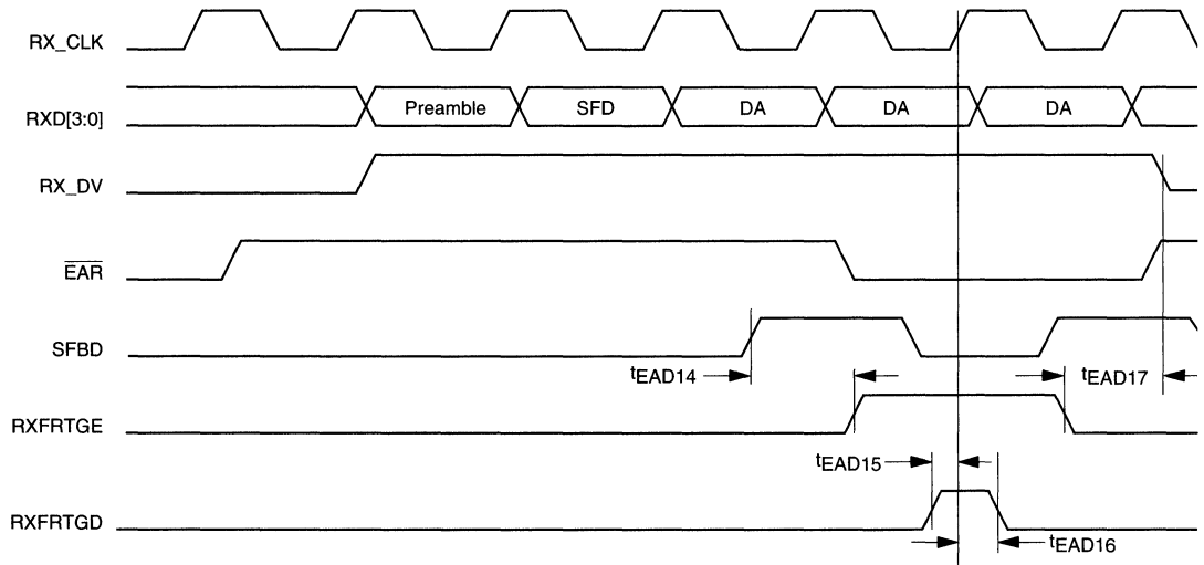
Figure C-11. Receive Frame Tag Timing with Media Independent Interface
