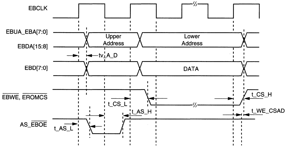
Figure 71. Expansion Bus Write Timing
