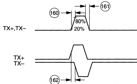
Figure 55. PMD Interface Timing (PECL)
