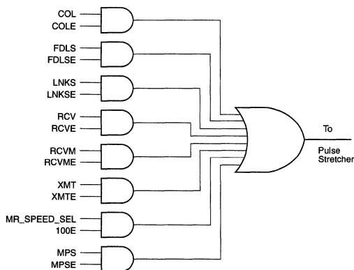
Figure 48. LED Control Logic
