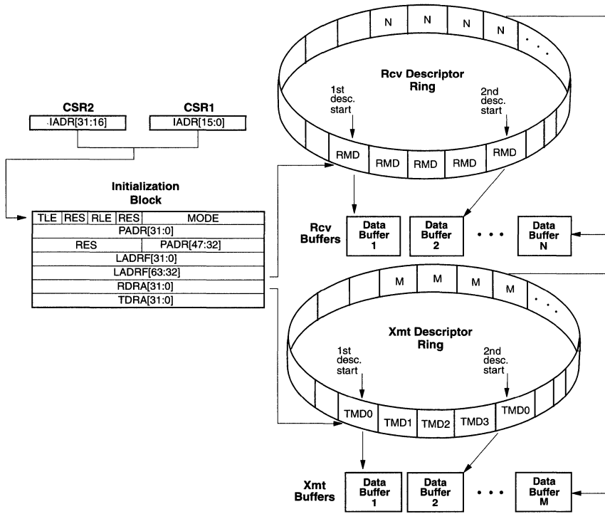
Figure 32. 32-Bit Software Model
