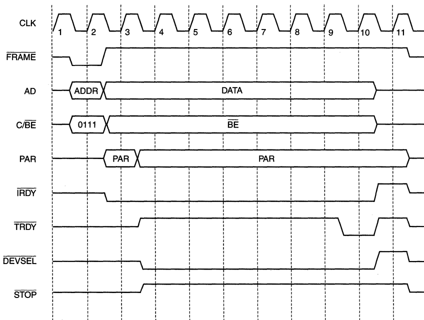
Figure 4. Slave Write Using Memory Command
