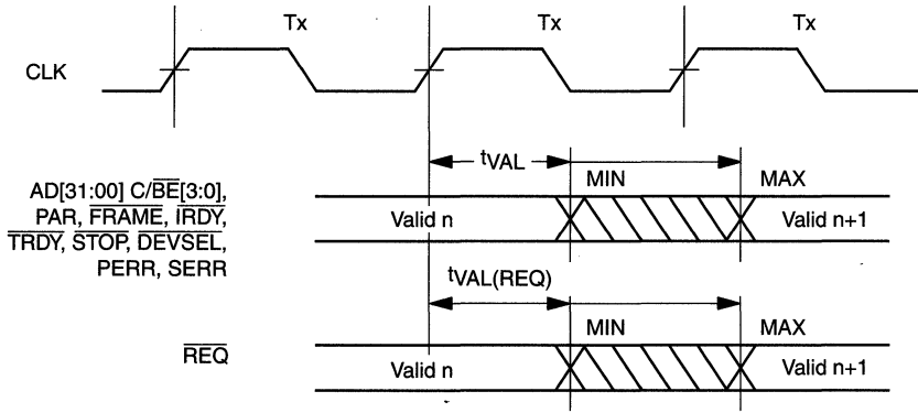
Figure 63. Output Valid Delay Timing
