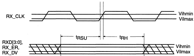
Figure C-5. Receive Timing
