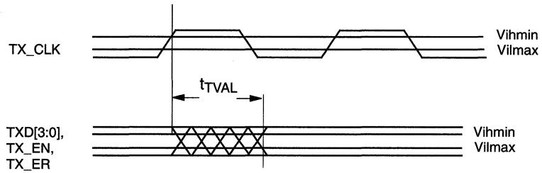
Figure C-4. Transmit Timing
