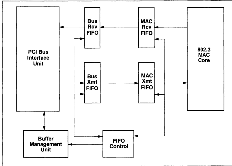
Figure 46. Block Diagram No SRAM Configuration
