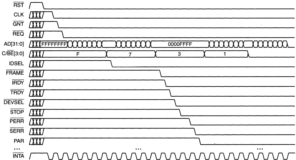
Figure 52. NAND Tree Waveform
