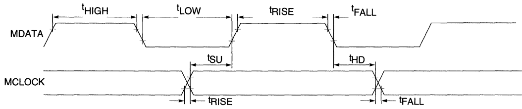
Figure B-8. System Management Interface Timing
