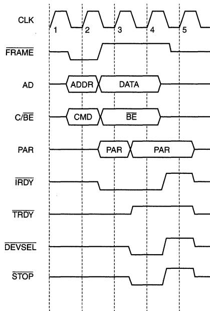
Figure 6. Disconnect Of Slave Cycle When Busy
