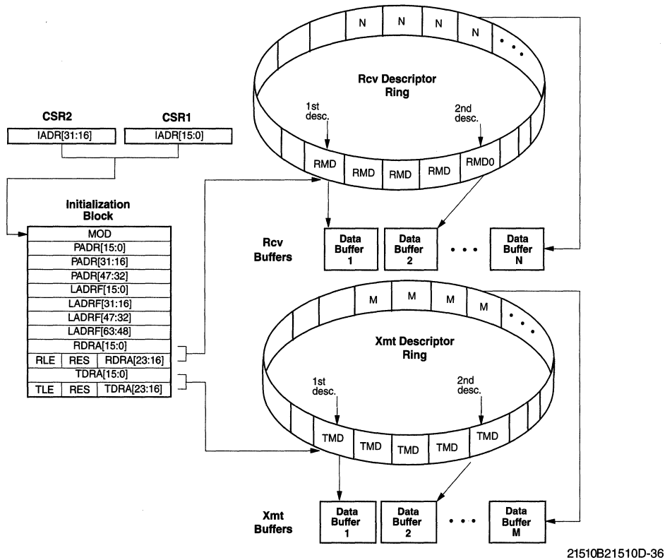
Figure 31. 16-Bit Software Model
