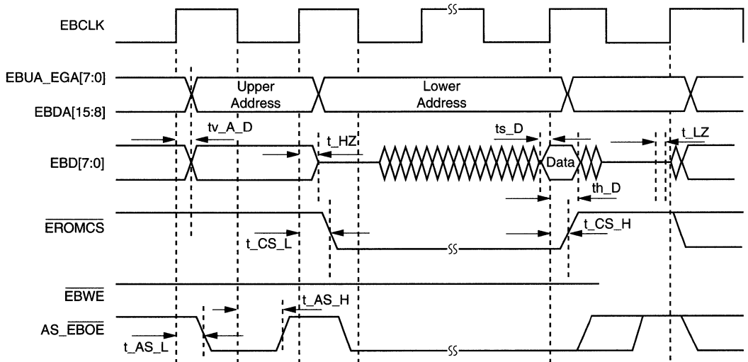
Figure 70. Expansion Bus Read Timing
