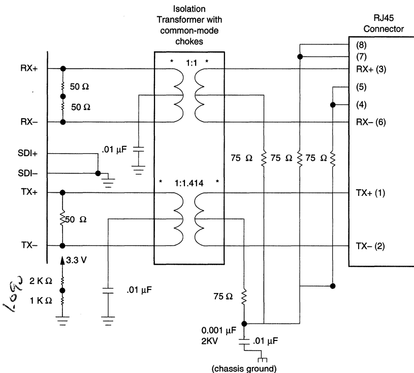
Figure 37. TX± and RX± Termination
