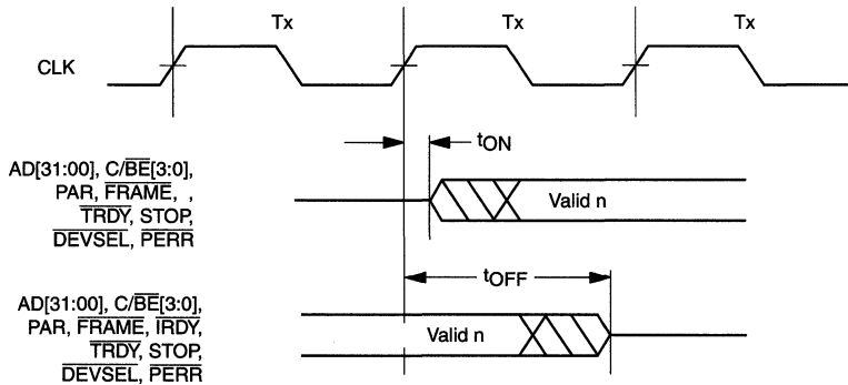
Figure 64. Output Tri-state Delay Timing
