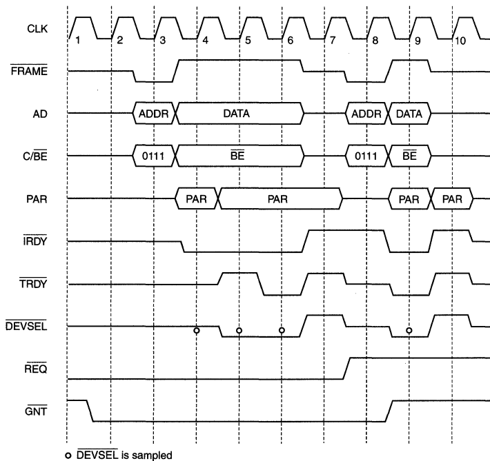
Figure 14. Non-Burst Write Transfer
