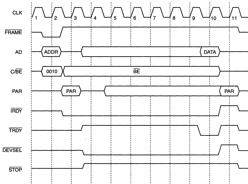
Figure 3. Slave Read Using I/O Command
